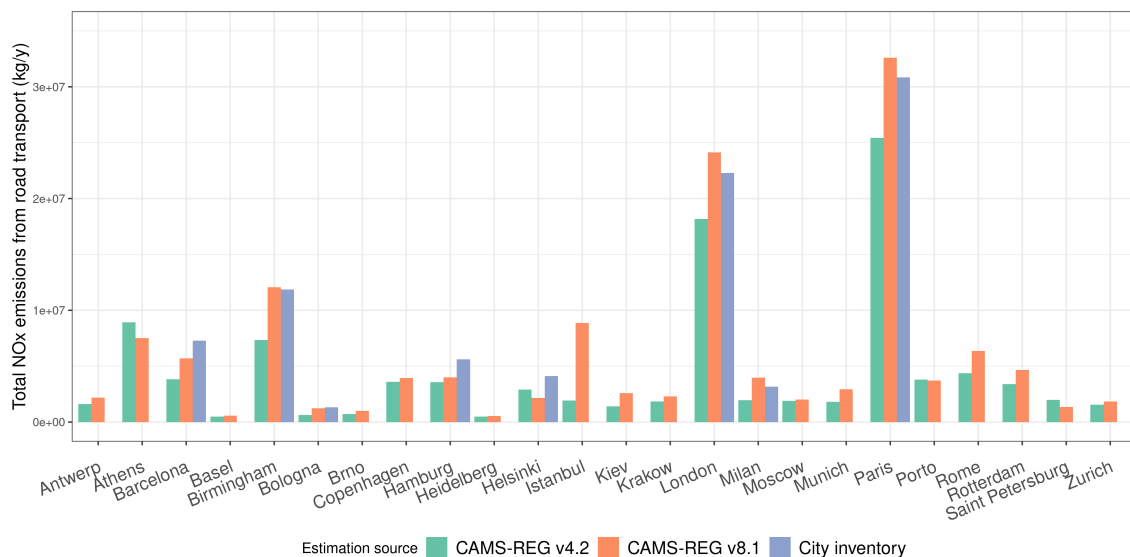
Figure 6. Comparison of annual NOx emissions from road transport of CAMS-REG 4.2, CAMS-REG 8.1 and local city inventories for 2018. Years covered by local inventories are given in Table 2. Note that the areas covered by city boundary shapes vary substantially. The city boundaries used for this comparison are provided in Section 5.
