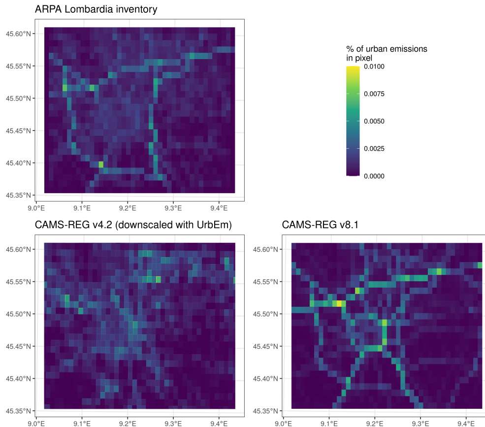
Figure 9. Comparison of the spatial distribution of urban NO x road transport emissions for Milan with local (base year 2019) and CAMS-REG inventories (0.01° x 0.007° resolution, base year 2018).
