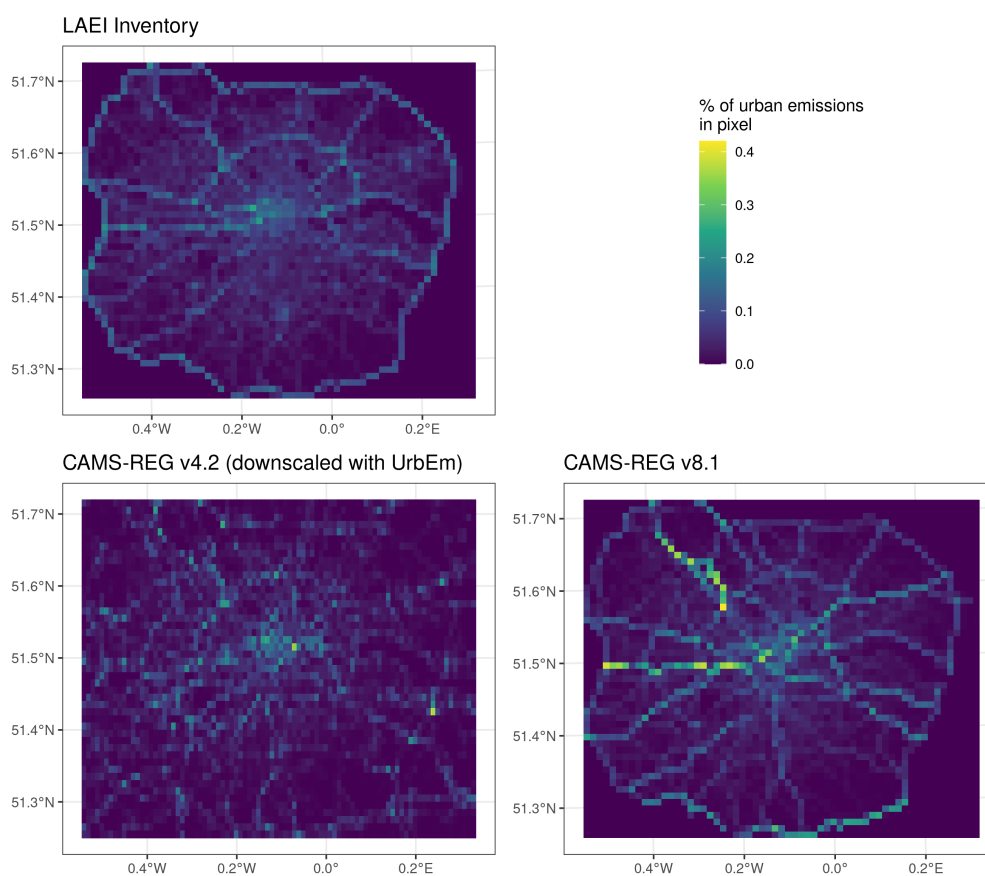
Figure 8. Comparison of the spatial distribution of urban NO x road transport emissions for London with local (LAEI, base year 2019) and CAMS-REG inventories (1 km resolution, base year 2018).
