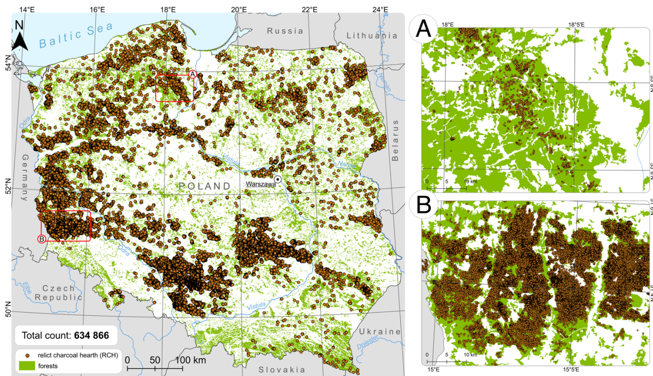
Figure 1. Location of the study area within Poland with all identified relict charcoal hearths (RCHs). The figure includes zoomed-in illustrations showing forest cover based on CORINE Land Cover 2018 (European Environmental Agency). Panels (A) and (B) present contrasting densities of RCH distribution across forested regions of Poland.
