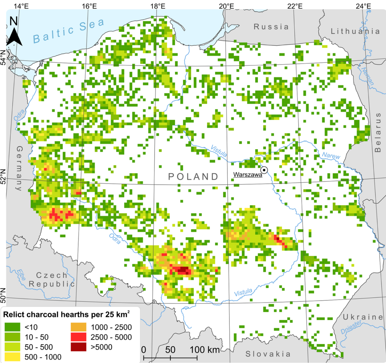
Figure 2. Map of the spatial density of relict charcoal hearths across forested areas of Poland
