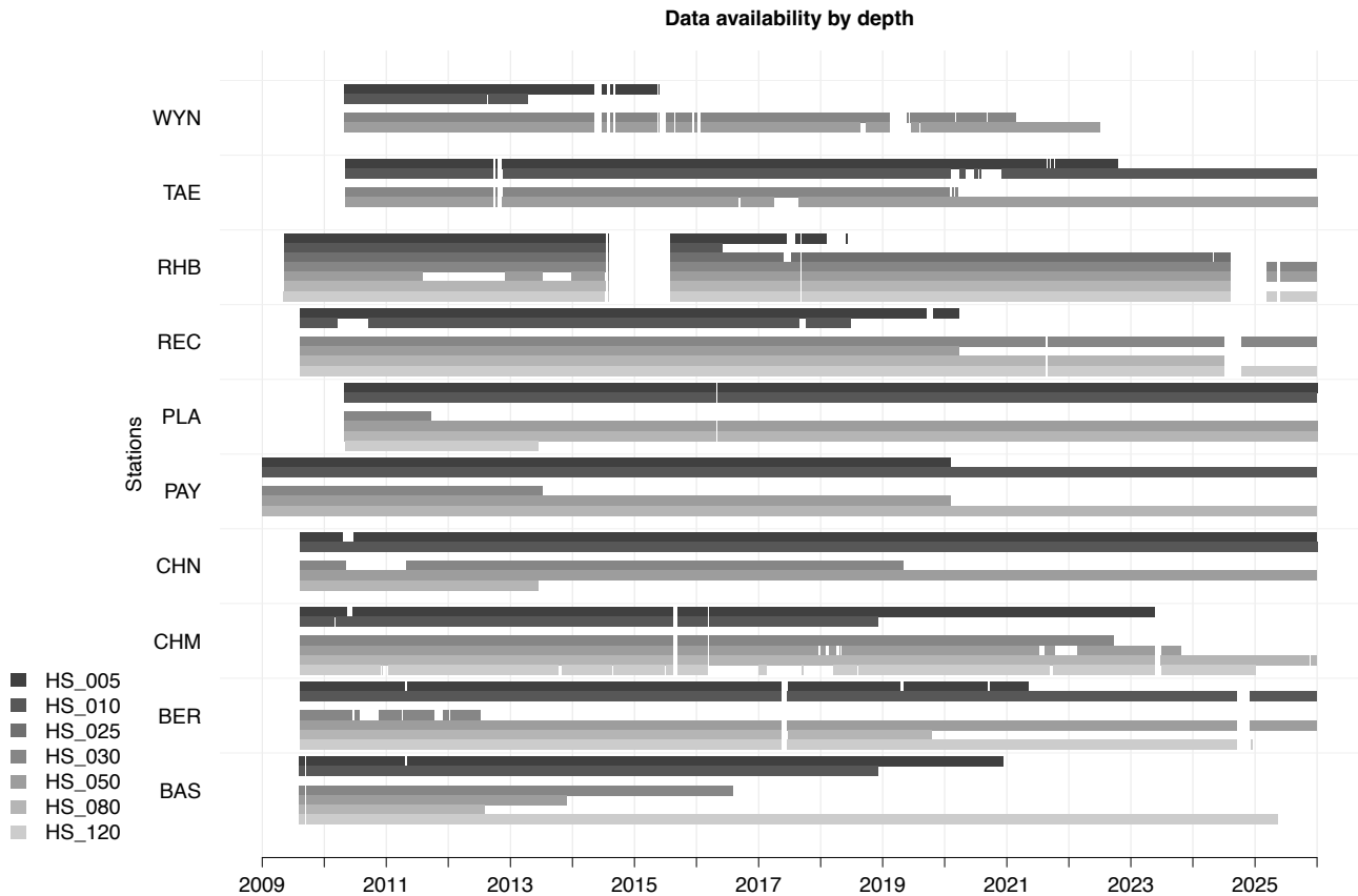
115 Figure 3 As Fig. 2, but for the Decagon 10HS (HS) sensors. In addition to the note on station RHB, REC has a 10HS sensor at 150 cm depth instead of 120 cm, which is shown as HS_120 for simplicity.
