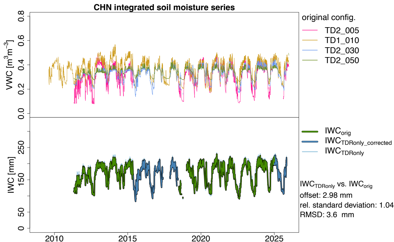
Figure 5 As Fig. 4 but for Changins (CHN), where historical gaps in IWC_{orig} could be filled. Note that IWC_{TDRonly\_corrected} is only shown when IWC_{orig} is not available.
