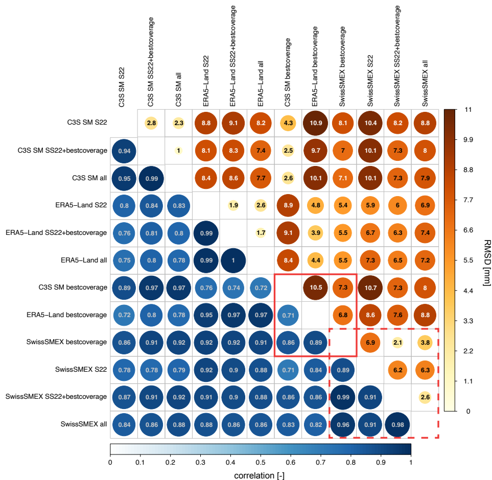
Figure 7 Pearson correlation and RMSD matrices from the pairwise comparison of SwissSMEX, ERA5-Land and C3S SM PASSIVE soil moisture, considering the different station combinations for the Swiss Plateau median time series of summer soil moisture anomalies (expressed as the absolute deviations from the 2010–2020 summer mean). Values are calculated for the common period 2010–2025. All correlations are significant ( p < 0.05 ). The red dashed rectangle highlights the comparison of the different station combinations based on SwissSMEX, while the red solid rectangle highlights the comparison of the gridded products and SwissSMEX based on the best coverage station combination. See Fig. S5 for the corresponding summer-half-year correlations and RMSDs.
