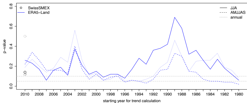
1650 Figure B1. Significance of the Theil-Sen trend slope (p-value of the Mann-Kendall trend test) based on ERA5-Land soil moisture as a function of the starting year for calculating the trend (i.e. the length of the time series). The trends are calculated based on the median time series of the absolute soil moisture anomalies from the best coverage stations (solid lines in Fig. 8). In addition to the summer and summer half-year trends, annual trends are also considered. Starting year 2010 refers to the 2010–2025 trend (or 16 years of data), starting year 1980 refers to the 1980–2025 trend (46 years of data). The p-values for SwissSMEX based on the 16- year time series are shown as circles at starting year 2010. The horizontal lines indicate the p=0.05 and p=0.1 thresholds.
