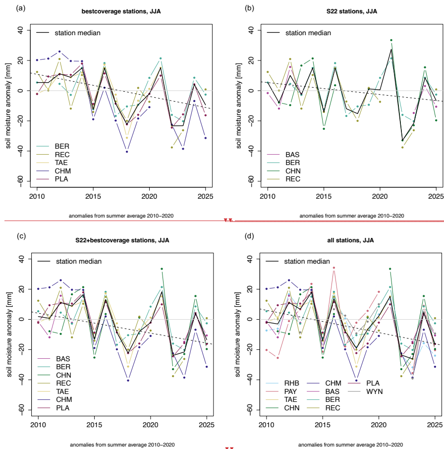
Figure 6 Soil moisture anomaly time series of summer JWC of different SwissSMEX station combinations (see Sect. 2.3, Table 1) and respective station medians. (a) Stations with best temporal coverage, (b) station selection as in S22, (c) S22 and best coverage stations combined, (d) all Swiss Plateau stations. Anomalies are expressed as the absolute deviations from the summer mean over 2010–2020. The straight lines show the Theil-Sen trend slopes for the period 2010–2025 based on the respective station median time series (solid lines indicate a significant trend with p < 0.05 ; dashed lines indicate a non-significant trend).
