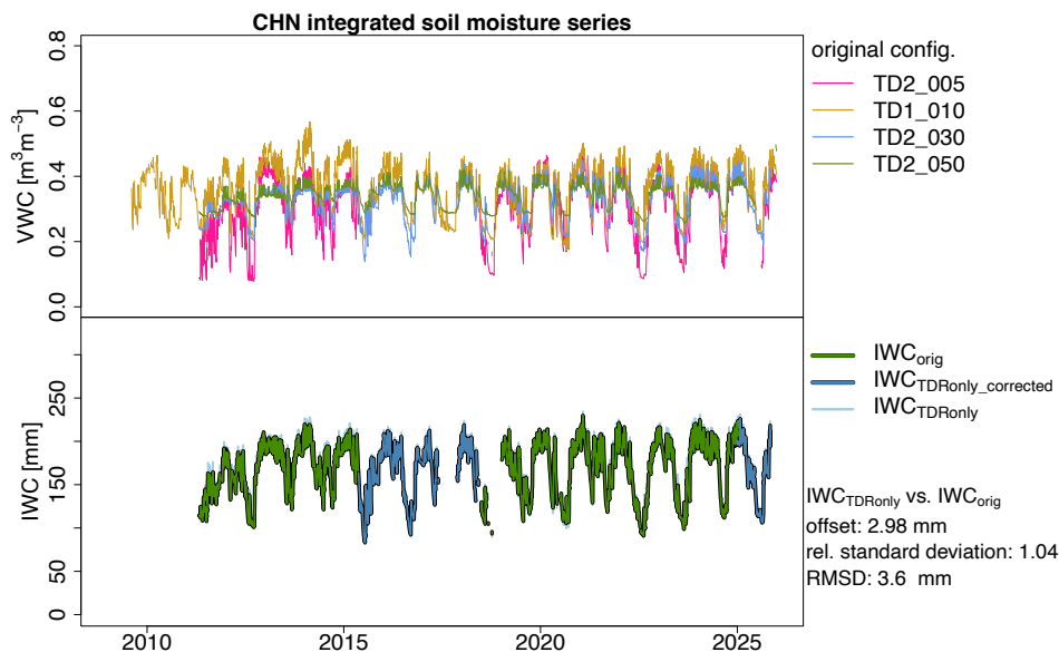
Figure 5 As Fig. 4 but for Changins (CHN), where historical gaps in IWC_{orig} could be filled. Note that IWC_{TDOnly\_corrected} is only shown when IWC_{orig} is not available.
