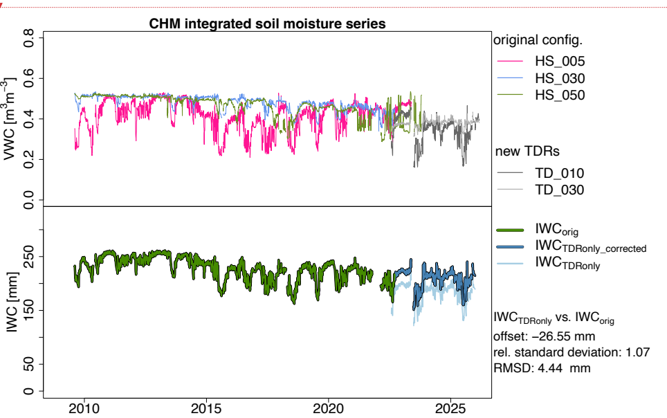
Figure 4. Daily time series of volumetric water content (VWC, in \text{m}^3 \text{m}^{-3} ) and vertically integrated soil water content (IWC, in mm) at the station Chamau (CHM), where IWC orig could be extended to the present. (Top) VWC from the 10HS sensors contributing to IWC orig , based on the original sensor configuration (see also Table S1), and from the two new TDRs installed in 2022 that are used to calculate IWC TDRonly . (Bottom) IWC orig and the 10 and 30 cm TDR-only based IWC TDRonly and IWC TDRonly corrected (see Eq. 3a,b). The original offset of IWC TDRonly is also noted, as well as its relative standard deviation and RMSD compared with IWC orig (all metrics are based on the overlapping hourly time steps). See Figs. S1–S4 for similar plots for the other stations.
