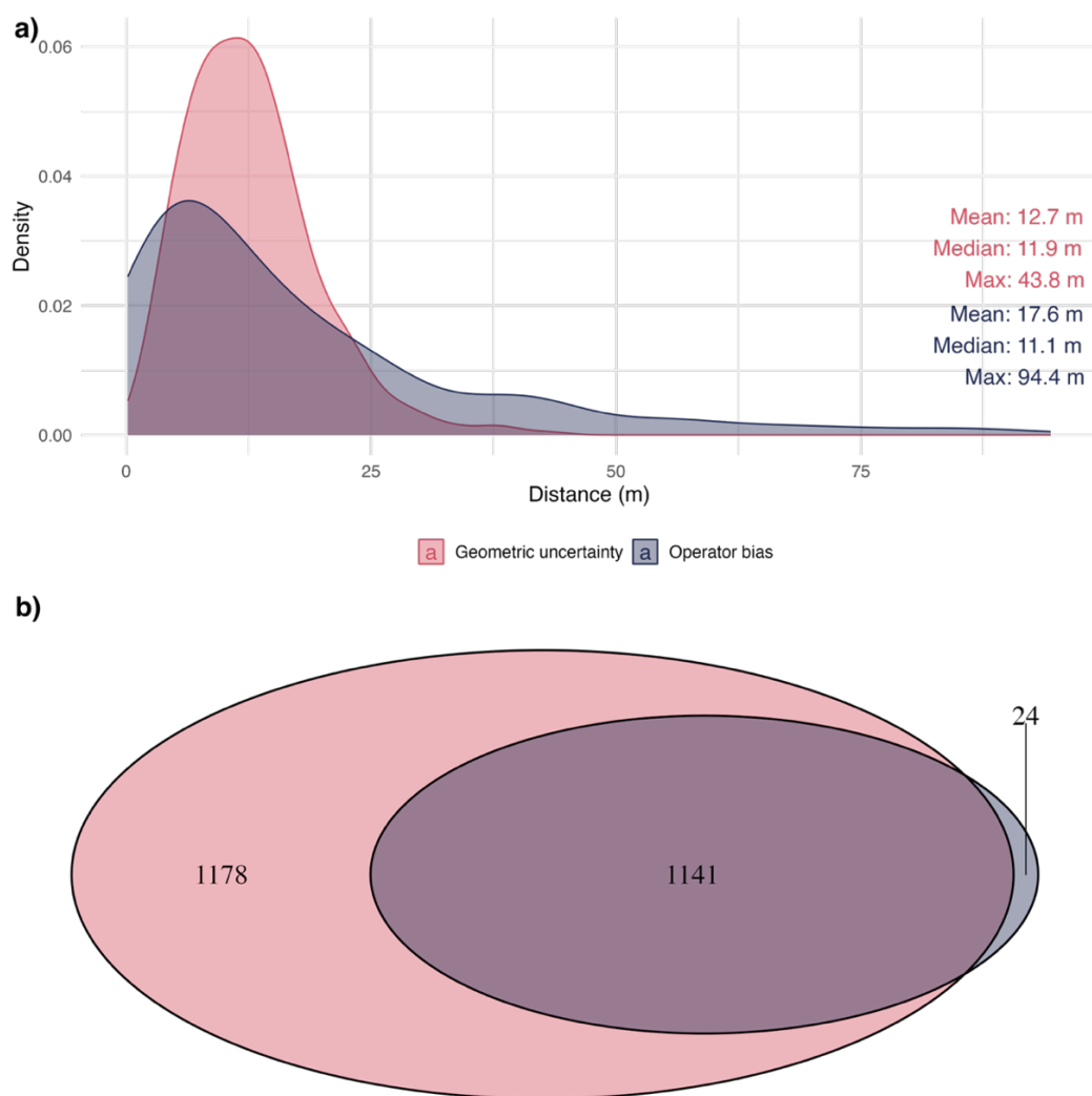
320 Figure 6: Uncertainties of the PROMICE-2022 ice mask. (a) Density distributions of geometric uncertainty and operator bias expressed as Euclidean distances (in meters) between mapped features. Geometric uncertainty reflects discrepancies due to image resolution and geolocation, while operator bias captures variation between independent interpretations. (b) Venn diagram illustrating omission error based on comparison with an independent mapping: 1,141 nunataks were identified by both mappers, 1,178 were unique to the PROMICE-2022 nunatak mapping, and 24 were omitted and only identified by the independent mapper.
