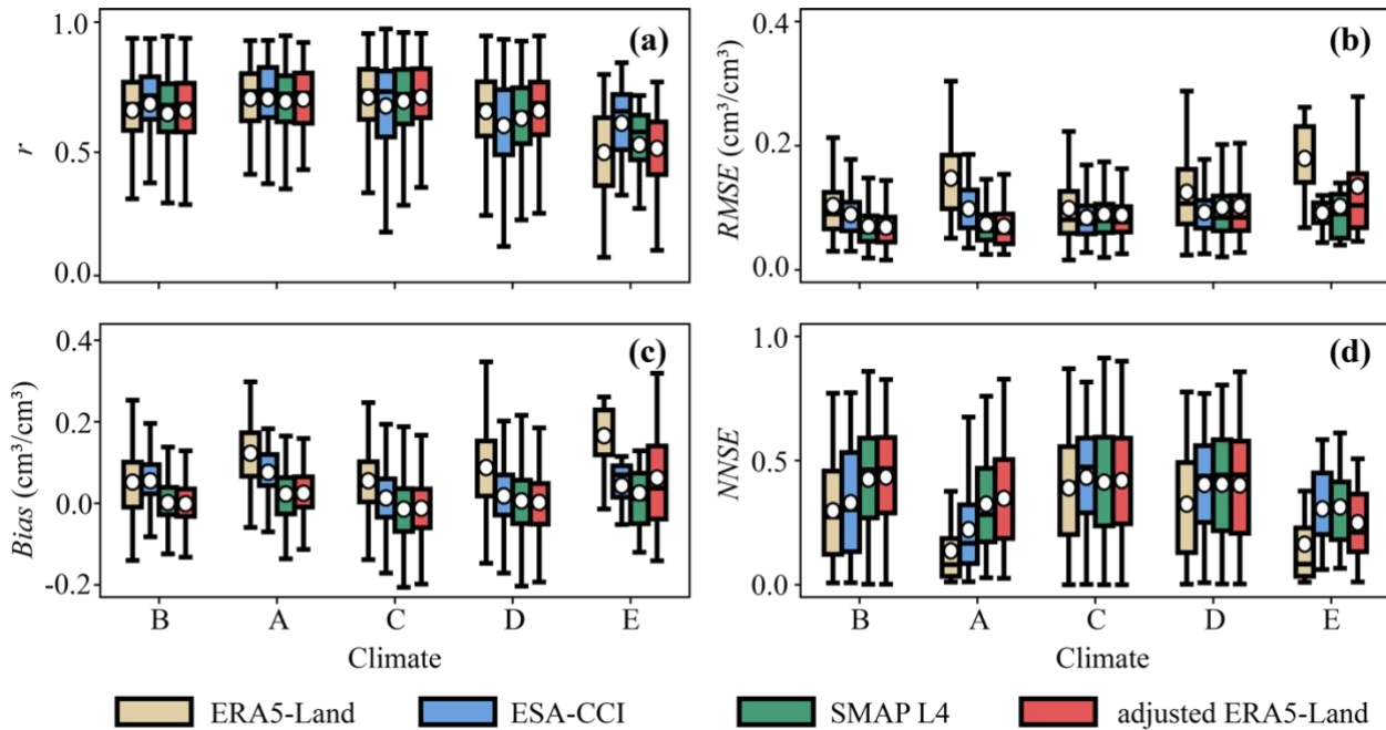
595 Figure 12. Distributions of four performance metrics, including (a) the Pearson correlation coefficient r , (b) RMSE , (c) Bias , and (d) NNSE from the comparison between in situ measurements and the four soil moisture products across different climate zones. The climate zones are categorized as A (Tropical), B (Arid), C (Temperate), D (Cold), and E (Polar). The classification of Zone B is based on precipitation and evaporation, whereas Zones A, C, D, and E are classified by temperature. Accordingly, the x-axis are ordered from the warmest to coldest (A, C, D, and E).
