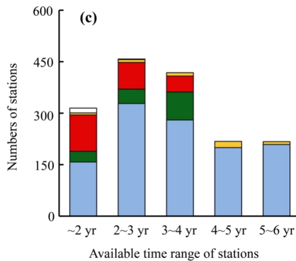
190 Figure 1. Spatiotemporal characteristics of the primary in situ dataset used for the main analysis (2015-2020). (a) Global distribution of the 1,615 in situ soil moisture stations used in this study, with colors differentiating the five source networks: ISMN, CMA, Cemaden, COSMOS-Europe, and SONTE-China; (b) Numbers of in situ soil moisture stations in each continent including North America (NA), Asia (AS), Europe (EU), South America (SA), Africa (AF), and Oceania (OC); (c) Numbers of stations with valid soil moisture data records across time range of different years within the 2015-2020 study window. The map in panel (a) was generated using the Matplotlib Basemap toolkit, with coastline and boundary data sourced from GSHHG and Natural Earth.
