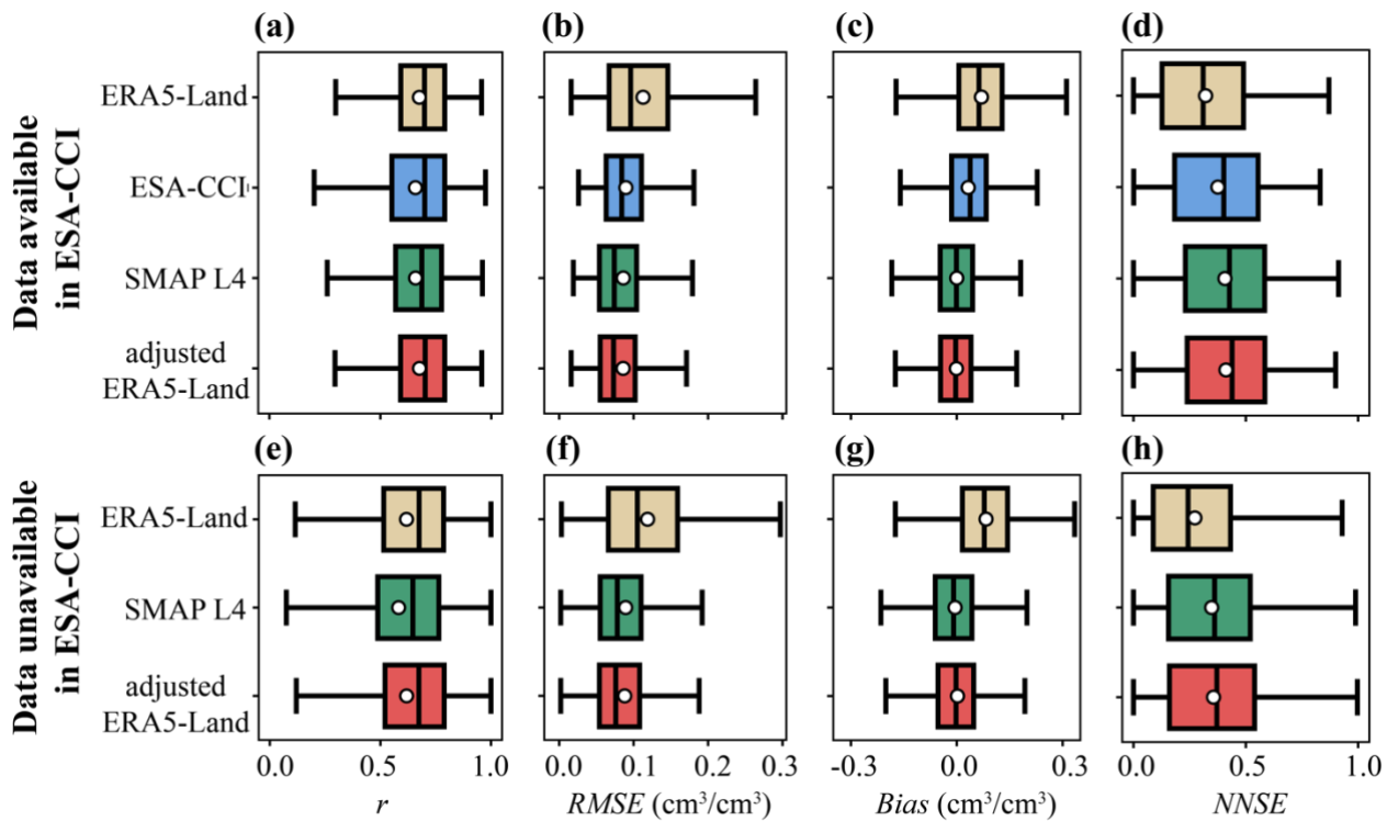
Figure 10. Evaluation of soil moisture products using performance metrics aggregated across all measurement stations. The columns present the results for four metrics: the Pearson correlation coefficient r , RMSE , Bias , and the NNSE . The analysis is stratified into two data subsets with the upper panel showing the metric values for periods when ESA-CCI data are available, while the lower panel indicating the periods when ESA-CCI data are unavailable.
