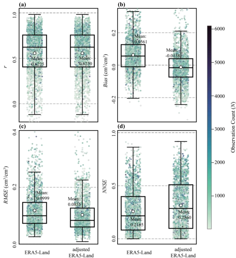
Figure 13. Comparative evaluation of the extended adjusted ERA5-Land soil moisture dataset versus the original ERA5-Land against ISMN in situ observations for the historical period (1960 - March 2015). The panels display the distributions of four performance metrics: (a) Pearson correlation coefficient ( r ), (b) Bias (cm 3 /cm 3 ), (c) RMSE (cm 3 /cm 3 ), and (d) NNSE . In the density scatter plots, each point represents a single ISMN station with more than 10 valid observations ( N > 10) throughout the entire historical period, colored according to the available observation count as shown in the color bar. The overlaid boxplots summarize the statistical distribution: the box spans the interquartile range (25th to 75th percentiles), and the central line marks the median. The white circles and numerical labels indicate the mean value of each distribution.
