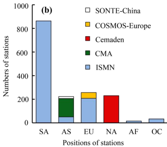
190 Figure 1. Spatiotemporal characteristics of the primary in situ dataset used for the main analysis (2015-2020). (a) Global distribution of the 1,615 in situ soil moisture stations used in this study, with colors differentiating the five source networks: ISMN, CMA, Cemaden, COSMOS-Europe, and SONTE-China; (b) Numbers of in situ soil moisture stations in each continent including North America (NA), Asia (AS), Europe (EU), South America (SA), Africa (AF), and Oceania (OC); (c) Numbers of stations with valid soil moisture data records across time range of different years within the 2015-2020 study window. The map in panel (a) was generated using the Matplotlib Basemap toolkit, with coastline and boundary data sourced from GSHHG and Natural Earth.
