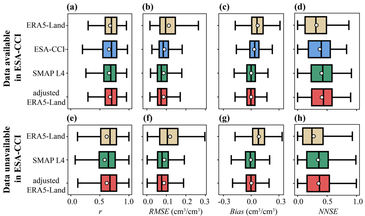
555 Figure 10. Evaluation of soil moisture products using performance metrics aggregated across all measurement stations. The columns present the results for four metrics: the Pearson correlation coefficient r , RMSE , Bias , and the NNSE . The analysis is stratified into two data subsets with the upper panel showing the metric values for periods when ESA-CCI data are available, while the lower panel indicating the periods when ESA-CCI data are unavailable.
