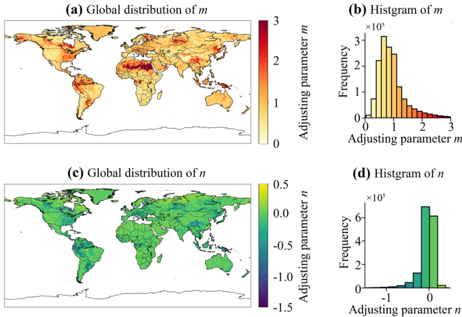
Figure 4. Global maps of mean-variance adjustment parameters m and n used to adjust ERA5-Land dataset for SMAP L4 fusion, with histograms showing the frequency distribution of the parameters.
