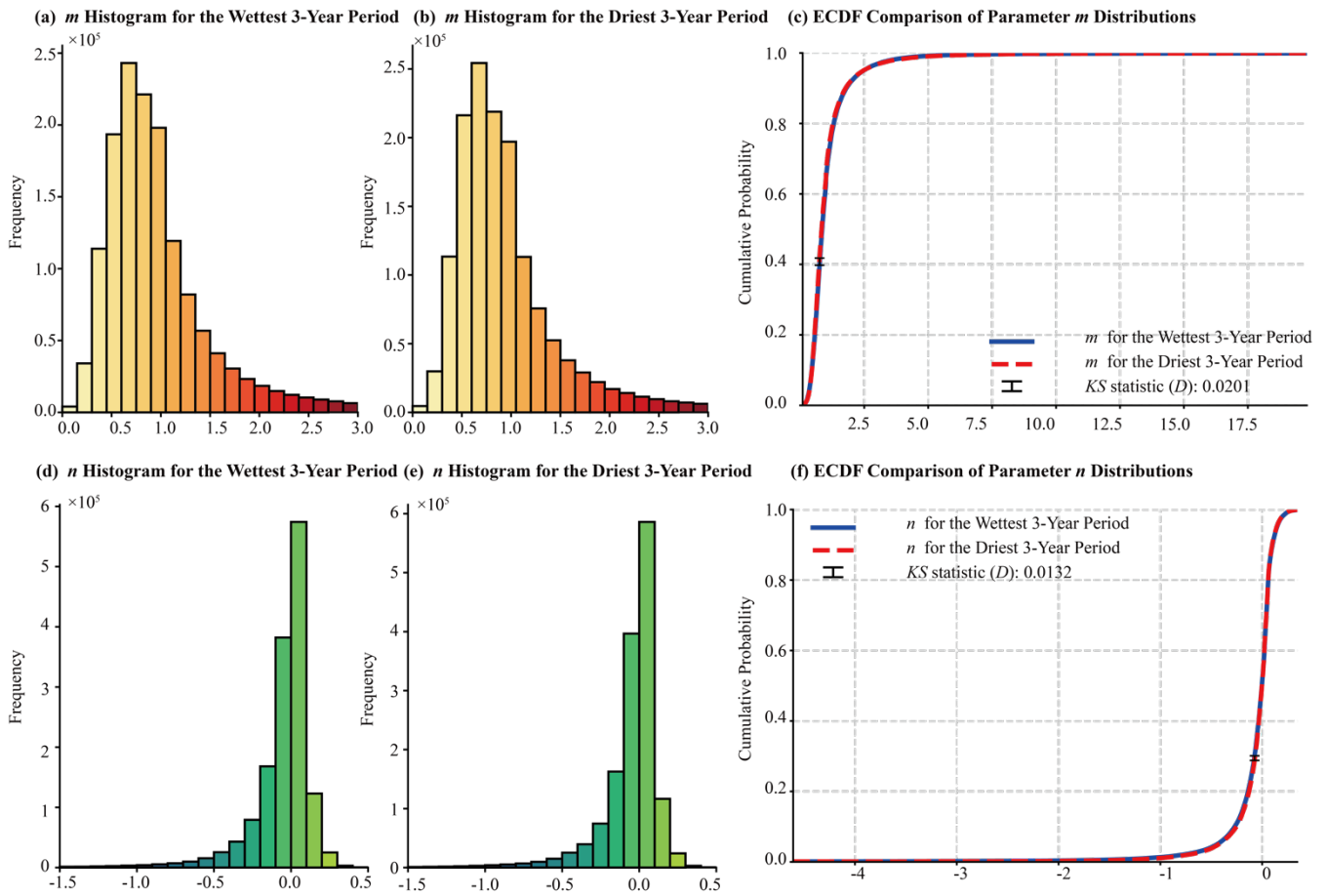
730 Figure 15. Assessment of the temporal stability of the mean-variance adjustment parameters m (top row) and n (bottom row) under contrasting climatic conditions. The distributions are derived from (a, d) the three wettest non-consecutive years and (b, e) the three driest non-consecutive years selected from 2015-2024. Panels (c) and (f) present the comparison of the Empirical Cumulative Distribution Functions (ECDFs), where the blue solid line represents the wettest period and the red dashed line represents the driest period. The black markers indicate the Kolmogorov-Smirnov (KS) statistic ( D ), which quantifies the maximum vertical divergence between the two distributions (0.0201 for m and 0.0132 for n ).
