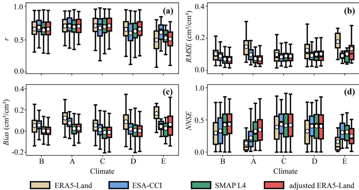
Figure 11. Distributions of four performance metrics, including (a) the Pearson correlation coefficient r , (b) RMSE , (c) Bias , and (d) NNSE from the comparison between in situ measurements and the four soil moisture products across different climate zones. The climate zones are categorized as A (Tropical), B (Arid), C (Temperate), D (Cold), and E (Polar). The classification of Zone B is based on precipitation and evaporation, whereas Zones A, C, D, and E are classified by temperature. Accordingly, the x-axis are ordered from the warmest to coldest (A, C, D, and E).
