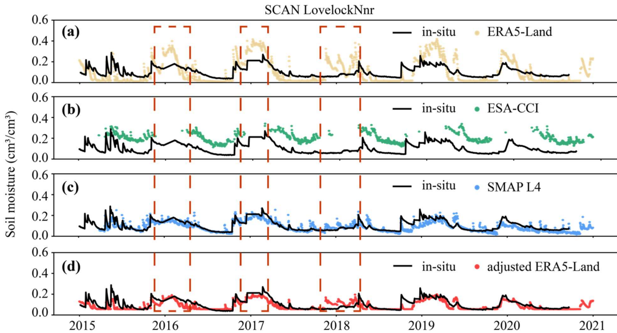
510 Figure 8. Data coverage and gaps at a representative station of SCAN LovelockNnr, Nevada, USA, comparing in situ observations with multiple soil moisture products. The time series of in situ soil moisture measurements is depicted as a solid black line, while corresponding estimates from the moisture products are shown as colored dots. Periods with missing data for the ESA-CCI dataset are highlighted by red dashed boxes.
