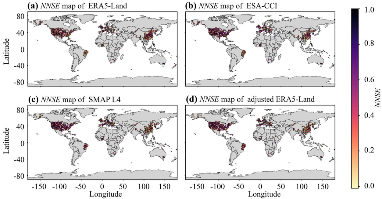
570 Figure 10. Global spatial distribution of the NNSE for four soil moisture products: (a) ERA5-Land, (b) ESA-CCI, (c) SMAP L4, and (d) the adjusted ERA5-Land. The performance of each product is evaluated against time series data from all 1,615 in situ stations.
