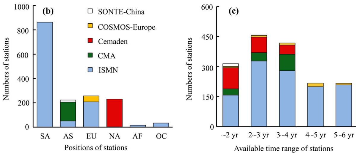
Figure 1. (a) global distribution of in situ soil moisture stations used in this study; (b) numbers of in situ soil moisture stations in each continent including North America (NA), Asia (AS), Europe (EU), South America (SA), Africa (AF), and Oceania (OC); (c) numbers of stations with valid soil moisture data records across time range of different years between 2015 to 2020.
