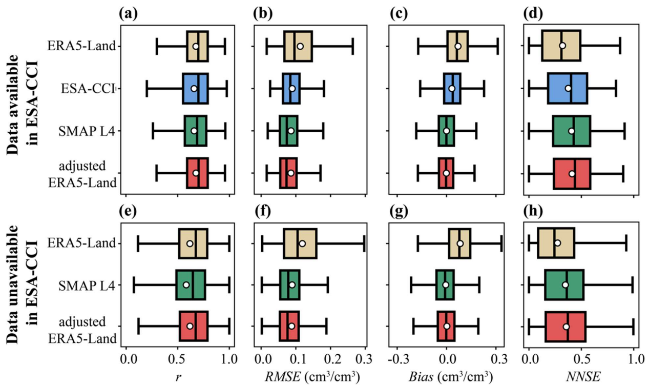
555 Figure 9. Evaluation of soil moisture products using performance metrics aggregated across all measurement stations. The columns present the results for four metrics: the Pearson correlation coefficient r , RMSE , Bias , and the NNSE . The analysis is stratified into two data subsets with the upper panel showing the metric values for periods when ESA-CCI data are available, while the lower panel indicating the periods when ESA-CCI data are unavailable.
