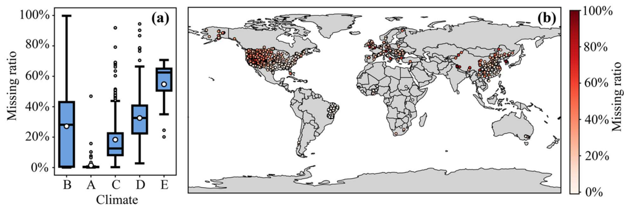
480 Figure 89. The ratio of missing ESA-CCI data at in situ measurement stations, presented for (a) different climate zones and (b) the corresponding global distribution. Climate zones are defined according to the Köppen-Geiger classification taken from Beck et al. (2018) with A (Tropical), B (Arid), C (Temperate), D (Cold), and E (Polar); the “All” category represents an aggregate of all stations. The classification for Zone B is based on precipitation and evaporation criteria, whereas Zones A, C, D, and E are primarily classified based on air temperature. To reflect these thermal distinctions, the zones in panel (a) are ordered from warmest to coldest (A, C, D, and E).
