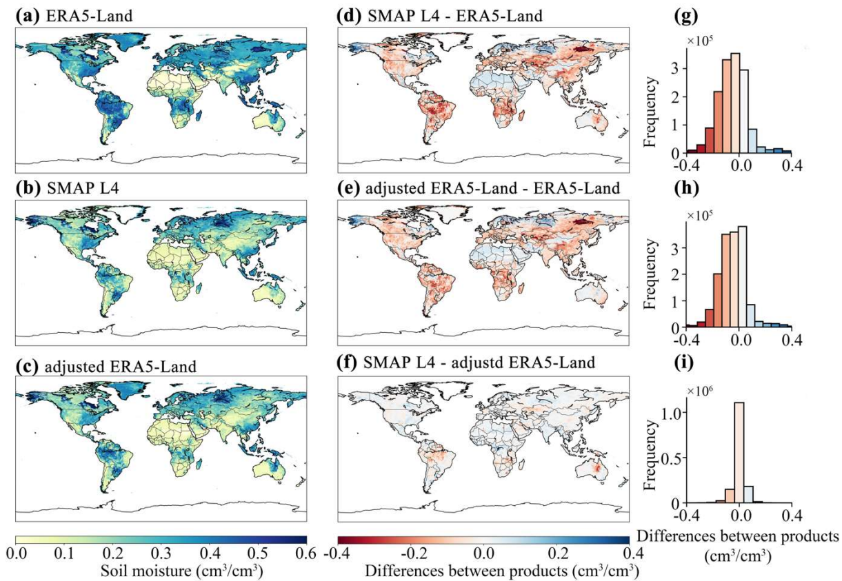
410 Figure 6. Spatial distribution of moisture dataset for an example date (January 1 st , 2016) and corresponding frequency distributions. (a-c) represent the spatial distributions of ERA5-Land, SMAP L4, and adjusted ERA5-Land, respectively. (d-f) show the spatial distributions of differences between (d) SMAP L4 minus ERA5-Land, (e) adjusted ERA5-Land minus ERA5-Land, and (f) SMAP L4 minus adjusted ERA5-Land. (g-i) provide frequency distributions corresponding to panels (d), (e), and (f), respectively.
