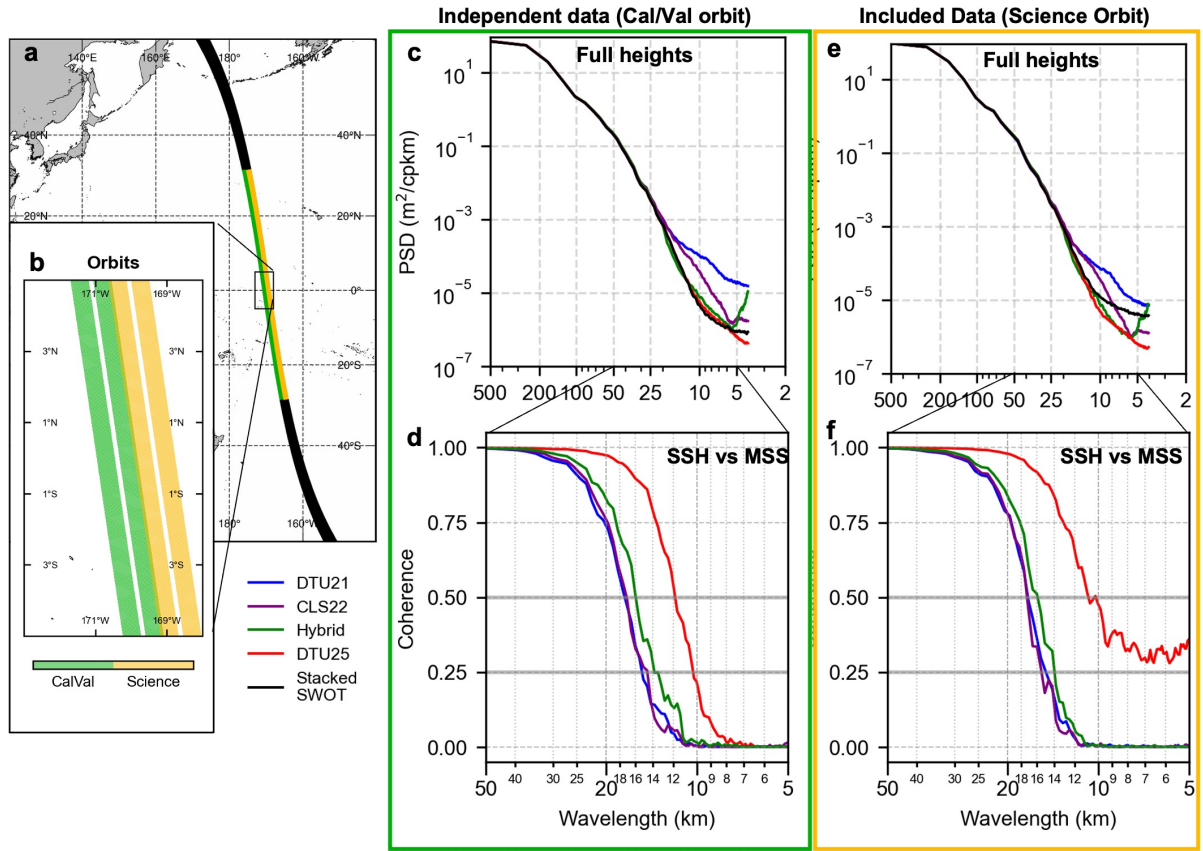
Figure 15. Power spectra and coherence determined from independent SWOT data (green) and included SWOT data (orange), with parallel groundtracks almost identical location ( a , b ). Plot c shows the power spectra of four MSS models interpolated onto the SWOT fixed geographical grid, along with the power spectra of the stacked (90 cycles) SSH observations from SWOT (black) in the Cal/Val orbit, not included in the MSS models. Plot d shows the corresponding coherence of the interpolated MSS models with SWOT. For e and f the same as before, but with the included SWOT data from the Science Orbit. Decoherence thresholds of 0.5 and 0.25 are marked in bold grey.
