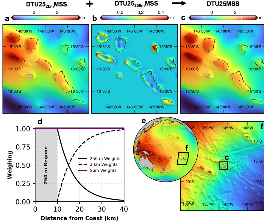
Figure 4. Example of the combination of the \text{DTU25}_{2\text{km}}\text{MSS} (a) and the new part in \text{DTU25}_{250\text{m}}\text{MSS} (b) MSS models to create the DTU25MSS c. Figure d shows the associated distance weighting for the 2 km and 250 m data products from SWOT. Figure e and f show the area depicted in this example.
