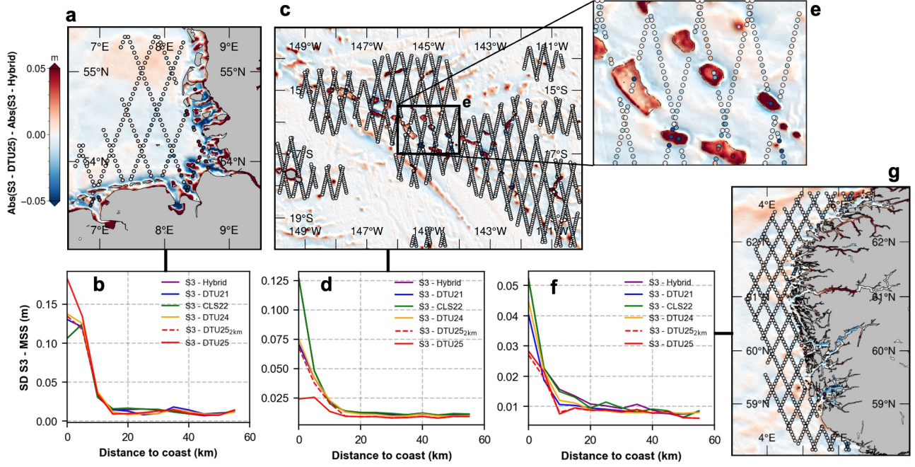
Figure 14. Standard deviation of the Sentinel-3A&B mean profiles subtracted from different MSS models, as a function of distance to the coast. Map a corresponds to the plot in b where the points are the bias-corrected absolute difference of Sentinel-3A&B and DTU25MSS subtracted from the bias-corrected absolute difference of Sentinel-3A&B and HybridMSS. Where blue indicates a better fit for DTU25MSS and red indicates a worse fit. This is equivalent for c-e and f-g . Matching maps and plots are indicated by the connecting line.
