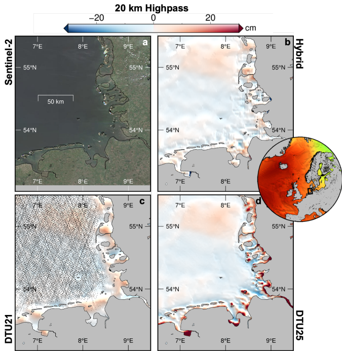
Figure 11. The Wadden Sea seen from Sentinel-2 (a) and highpass filtered at 20 km with the HybridMSS (b), DTU21MSS (c) and DTU25MSS (d). Black points in c shows where nadir altimetry observations are located that is used in the creation of the DTU21MSS.
