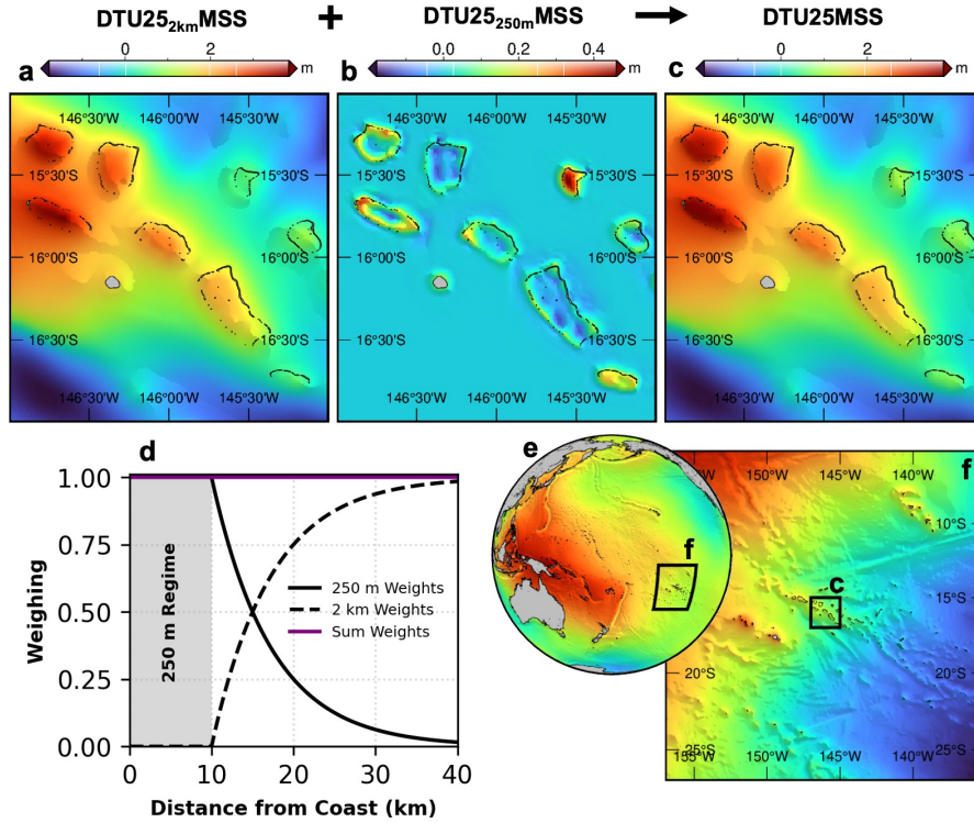
Figure 4. Example of the combination of the \text{DTU25}_{2\text{km}}\text{MSS} (a) and the new part in \text{DTU25}_{250\text{m}}\text{MSS} (b) MSS models to create the \text{DTU25MSS} c. Figure d shows the associated distance weighting for the 2 km and 250 m data products from SWOT. Figure e and f show the area depicted in this example.
