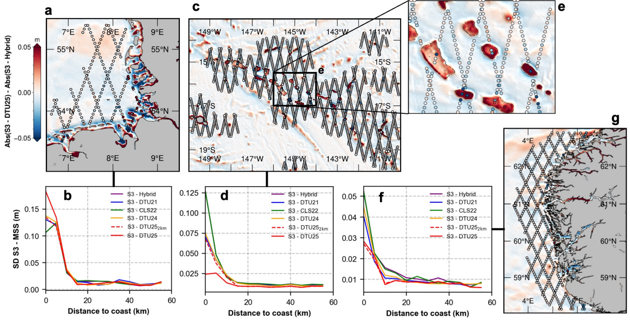
Figure 14. Standard deviation of the Sentinel-3A&B mean profiles subtracted from different MSS models, as a function of distance to the coast. In-maps Map a corresponds to e the plot in b where the points are the bias-corrected absolute difference of Sentinel-3A&B and DTU25MSS subtracted from the bias-corrected absolute difference of Sentinel-3A&B and HybridMSS, with. Where blue indicating indicates a better fit for DTU25MSS and red indicating indicates a worse fit. This is equivalent for c-e and f-g. Matching maps and plots are indicated by the connecting line.
