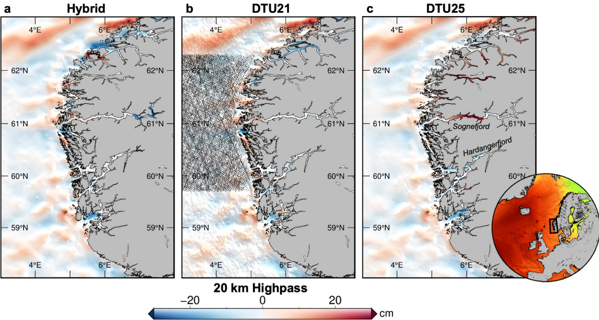
Figure 12. The western coast of Norway highpass filtered at 20 km with the HybridMSS, DTU21MSS and DTU25MSS in a , b and c respectively. Black points in b indicate where nadir altimetry observations are located (between 59.7°N and 62.3°N) in the creation of the DTU21MSS.
