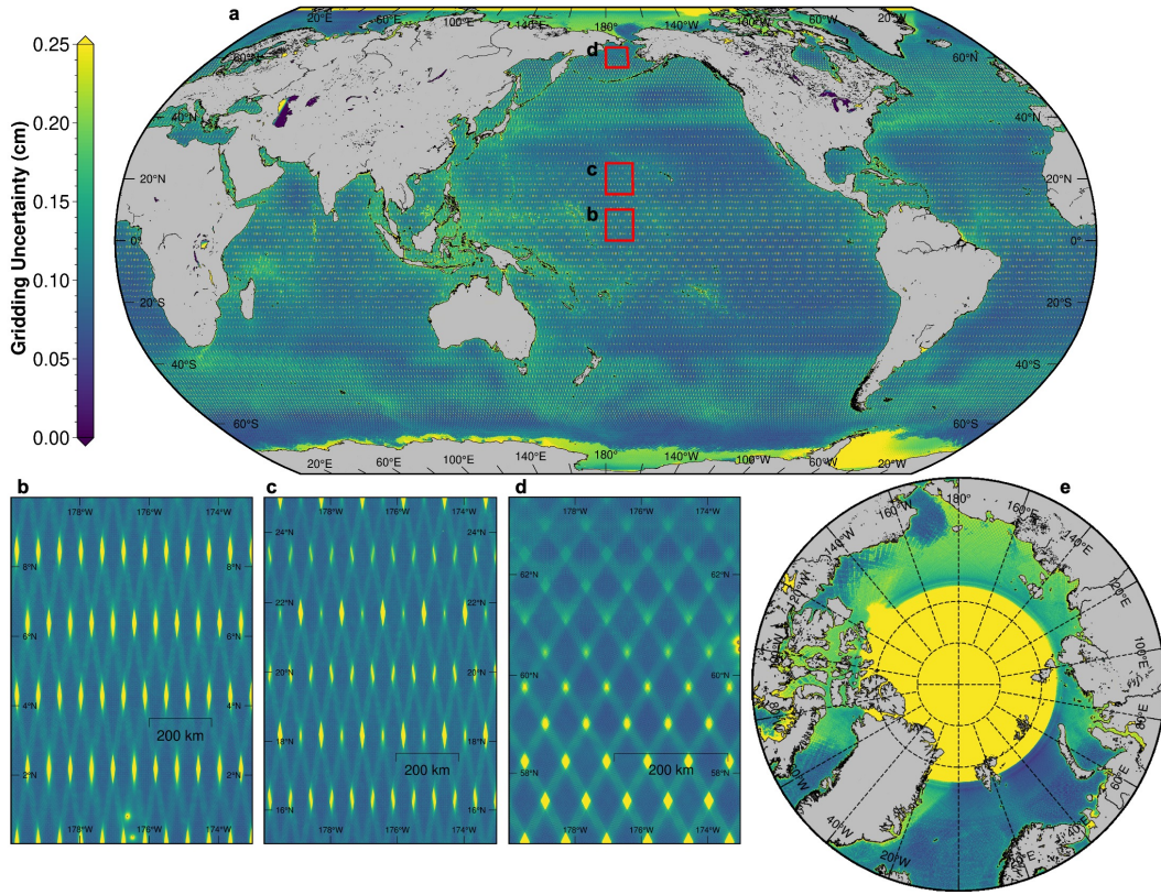
Figure 8. Gridding uncertainty ( \sigma_{\text{SLA}}^2 ) for DTU25 2km MSS. The focus on areas b-d shows the diamond shaped data-gaps left due to the coverage of the SWOT mission, as well as the closing of the gaps at specific latitudes. The arctic is shown in e , with the ice coverage clearly seen due to lower number of SWOT cycles available for the MSS determination. Uncertainty above 78°N is set to zero.
