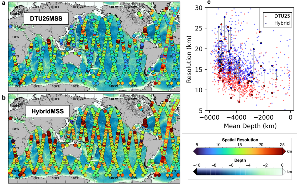
Figure 16. Spatial resolution determined as the wavelength at 0.5 coherence between SWOT Cal/Val orbit and the DTU25MSS or the HybridMSS in 6^\circ latitude bands, with 50% overlap. In c all resolutions for both MSS is shown as a function of mean ocean depth in the latitude band. Points with black border ( in c ) is points associated with the indicated track in a and b with red borders, and the connected vertical line indicates that the points are at the same location.
