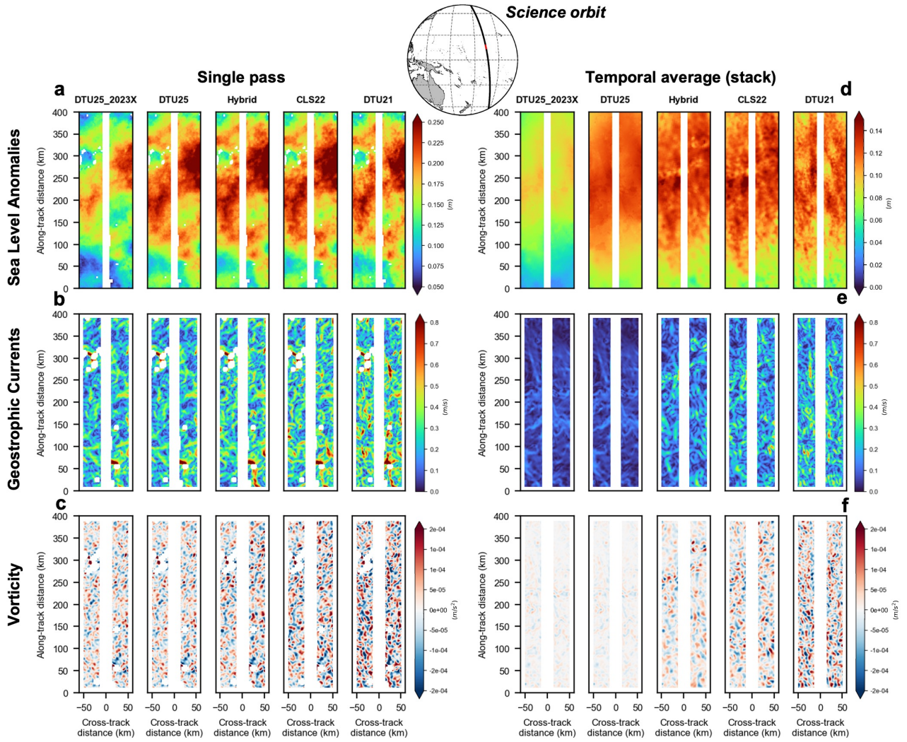
Figure 17. Three oceanographic variables (sea level anomaly a+d , geostrophic currents b+e and vorticity c+f ) computed for a single SWOT pass from the science orbit ( left , cycle 28 pass 28) and from the temporal average of 31 cycles ( right ) with different MSS models as reference.
