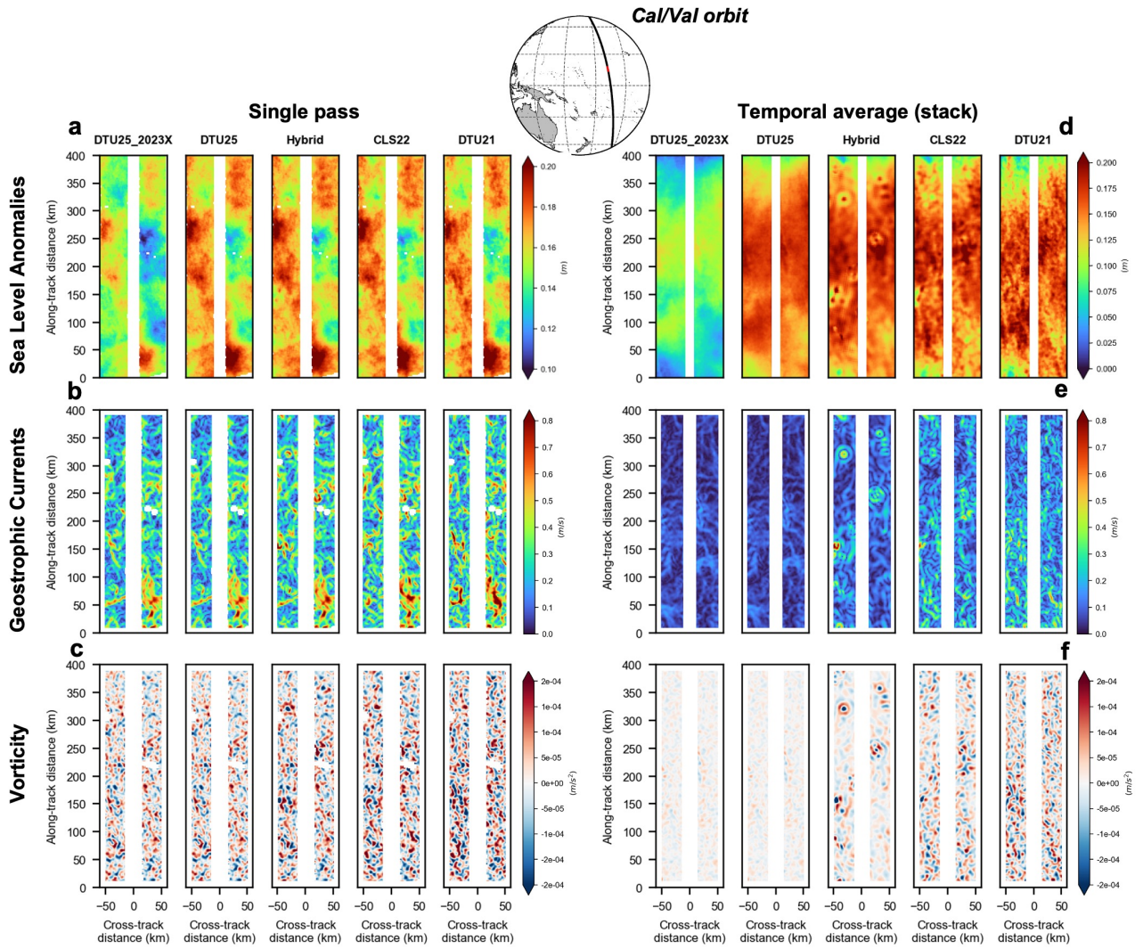
Figure 18. Three oceanographic variables (sea level anomaly a+d , geostrophic currents b+e and vorticity c+f ) computed for a single SWOT pass from the Cal/Val orbit ( left , cycle 475 pass 2) and from the temporal average of 90 cycles ( right ) with different MSS models as reference.
