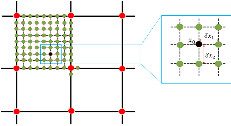
260 Figure 2. Schematic diagram of the spatial relationship between a main grid point and its surrounding auxiliary points in the Cauchy-Green strain tensor field. The black dot represents an auxiliary grid point x_0 , \delta x_1 and \delta x_2 denotes the distance between the auxiliary grid point (green) and the main grid point (red).
