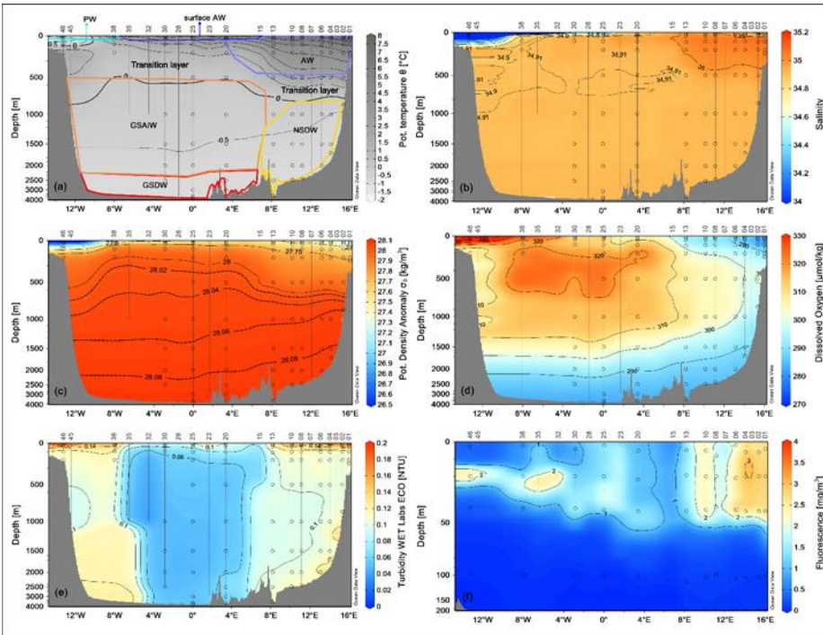
384 385 Figure 3 - Vertical distribution of (a) potential temperature ( ^{\circ}\text{C} ), (b) salinity, (c) potential density anomaly ( \text{kg m}^{-3} ), (d) 386 dissolved oxygen ( \mu\text{mol kg}^{-1} ), (e) turbidity (NTU), and fluorescence ( \text{mg m}^{-3} ) along the zonal transect at 75^{\circ}\text{N} in 387 September 2021. The empty dots indicate the sampling points of the Niskin bottles. Panel a show also the distribution of 388 principal water masses according to their core values [AW - Atlantic Water; GSAIW - Greenland Sea Arctic Intermediate 389 water; NSDW - Norwegian Sea Deep Water; GSDW - Greenland Sea Deep Water; PW - Polar Water or Melting Water]. 390 Depths on y-axis are non-linear. 391
