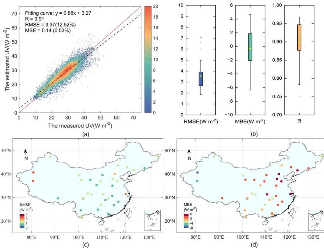
270 Figure 5. Same as Figure 4 but for daily mean clear-sky UV radiation.
