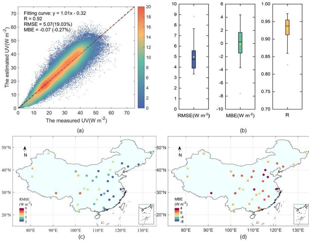
255 Figure 4. Validation results of the estimated hourly clear-sky UV dataset against observations at 37 CERN stations from 2005-2013. (a) Density scatter plot between the estimated dataset and observations. (b) Box plots of the three statistical error metrics (RMSE, MBE, and R). (c) Spatial distribution of RMSE at individual stations. (d) Spatial distribution of MBE at individual stations.
