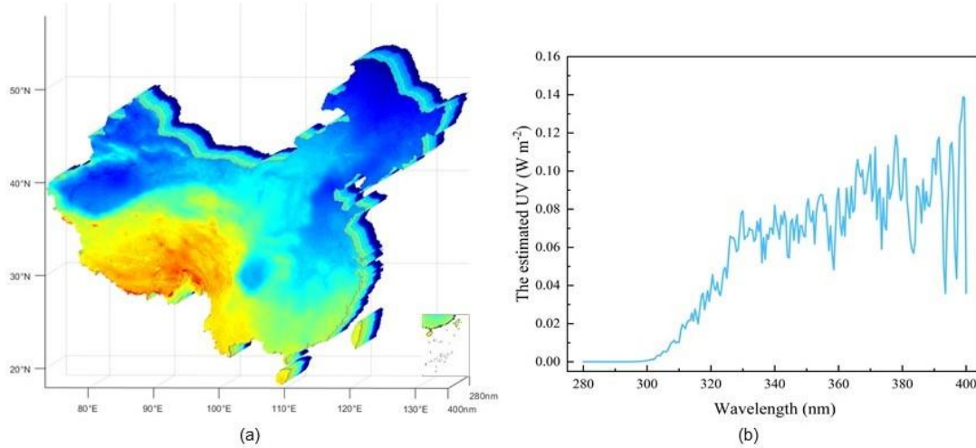
395 Figure 10. (a) 3D hyperspectral distribution of clear-sky UV radiation in China (2023). (b) Spectral variation of clear-sky UV radiation (280–400 nm) across entire China.
