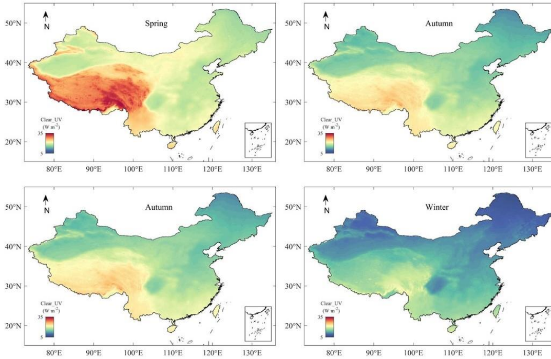
Figure 12. Average seasonal spatial distribution of clear-sky UV radiation in China from 1981 to 2023.
