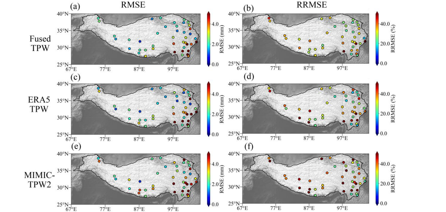
Figure 6. Comparison of RMSE (first column) and RRMSE (second column) at the station scale for the fused TPW, ERA5 TPW, and MIMIC-TPW2 under all-weather conditions. (a, b: fused TPW; c, d: ERA5 TPW; e, f: MIMIC-TPW2)
