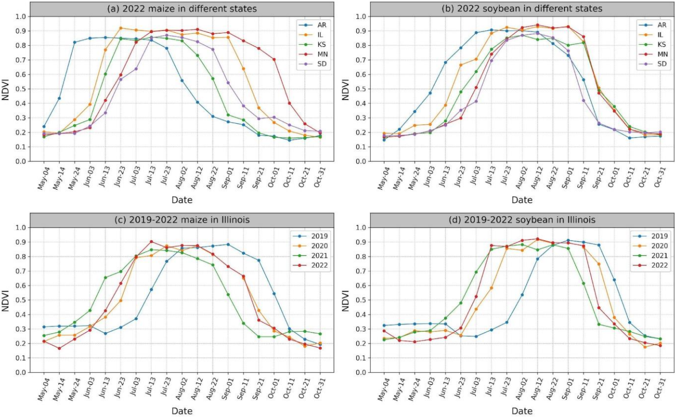
410 411 Figure 18: NDVI time series for maize and soybean from representative sites. (a) 2022 maize NDVI in Arkansas (AR), Illinois (IL), 412 Kansas (KS), Minnesota (MN), South Dakota (SD); (b) the same as (a) but for soybean; (c) 2019-2022 interannual NDVI variations 413 for maize in Illinois; (d) the same as (c) but for soybean. The details about the sites are shown in Figure S4 and Table S6.
