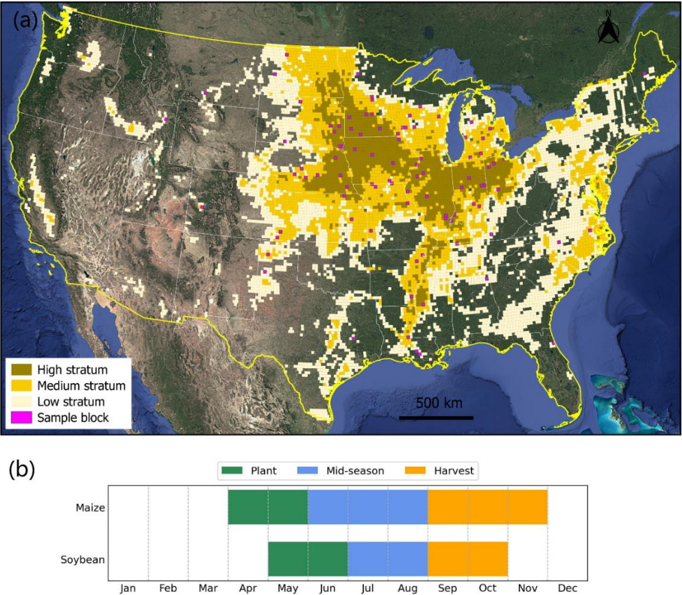
207 Figure 5: 2022 stratified sampling design for field survey. (a) stratified sampling design. 20 km × 20 km equal-area blocks were 208 stratified into high, medium and low strata. (b) crop calendar for maize and soybean over the US. Google Earth imagery is used as 209 background. 210
