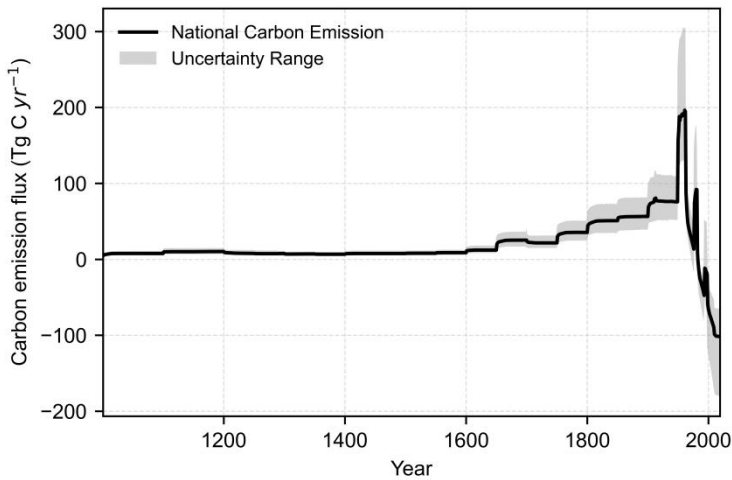
Figure 10. Carbon emission fluxes from land-use change in China with their uncertainties. The black line represents the mean result of 1000 Monte Carlo simulations using the grassland-priority allocation rule in land use conversion. The gray shaded area represents the uncertainty interval defined by the maximum and minimum values across all 3000 simulation runs (1000 iterations for each of the three allocation rules: grassland-priority, area-weighted, and forest-priority). This interval incorporates the combined uncertainties from input data, carbon density parameters, and the allocation rule. For details, refer to the sections 2.3.2 and 2.3.3.
