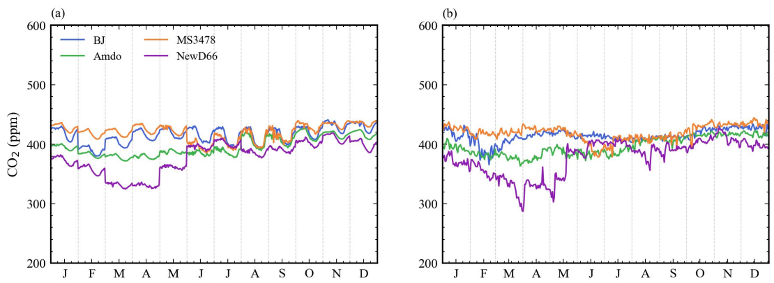
Figure 8. Monthly variations of the diurnal (a) and daily mean (b) CO 2 concentration at the 4 stations. As shown in Figure 8a, CO 2 concentrations exhibit a diurnal cycle characterized by an increase during nighttime and a decrease during daytime. This cycle shows minimal monthly variation across the observation period. The NewD66 station displays only a weak diurnal signal between June and August, which may be attributed to the sparse vegetation over the bareland underlying surface, resulting in a relatively limited influence on local CO 2 . In contrast, the diurnal cycle of CO 2 concentration is more pronounced at the BJ and MS3478 stations due to their dense vegetation. Figure 8b illustrates the annual variation in CO 2 concentration. The BJ station consistently exhibits lower CO 2 levels throughout the year, with more pronounced fluctuations during summer. Seasonal amplitude is greater at Amdo in summer and at MS3478 in winter. The most substantial annual variation is observed at NewD66, where CO 2 concentrations reach a minimum in April and peak in June.
