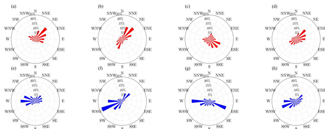
Figure 5. Wind direction during the monsoon season at NewD66 (a, 10.4 m), Amdo (b, 12.0 m), MS3478 (c, 10.35 m), and BJ (d, 12.0 m), compared to their wind direction during the non-monsoon season (e-h).
