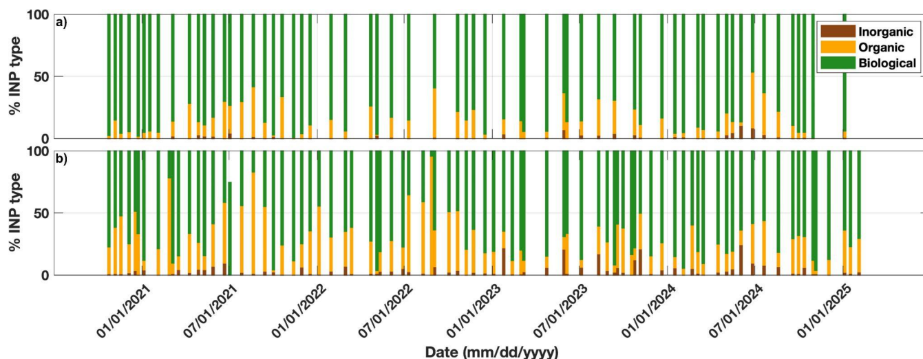
75 76 Figure 5: Relative abundance of INP type at the SGP C1 site at a) -15^{\circ}\text{C} and b) -25^{\circ}\text{C} that are currently available on DOE ARM 77 Data Discovery. INP types are determined through heat and peroxide treatments. We assume that the reduction of INPs from heat are 78 biological in nature (e.g., heat labile proteins) while the reduction of INPs from peroxide, UV, and heat are organic (e.g., heat labile organics). 79 INPs remaining (unaffected) by both treatments are inorganic (e.g., mineral dust). Data are from 84 samples that have been heat- and 80 peroxide-treated (34% of the processed SGP samples in Figure 4).
