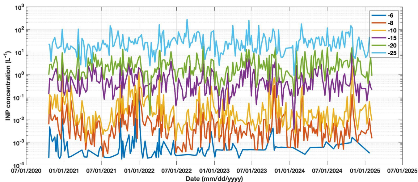
61 Figure 4: Complete time series of INP concentrations at select temperatures from the SGP C1 site that are currently publicly 62 available on DOE ARM Data Discovery. Each line shows cumulative INP concentrations per liter of air ( \text{L}^{-1} ) at freezing temperatures 63 designated in the legend (in ^{\circ}\text{C} ). Data are from 247 total processed filter samples.
