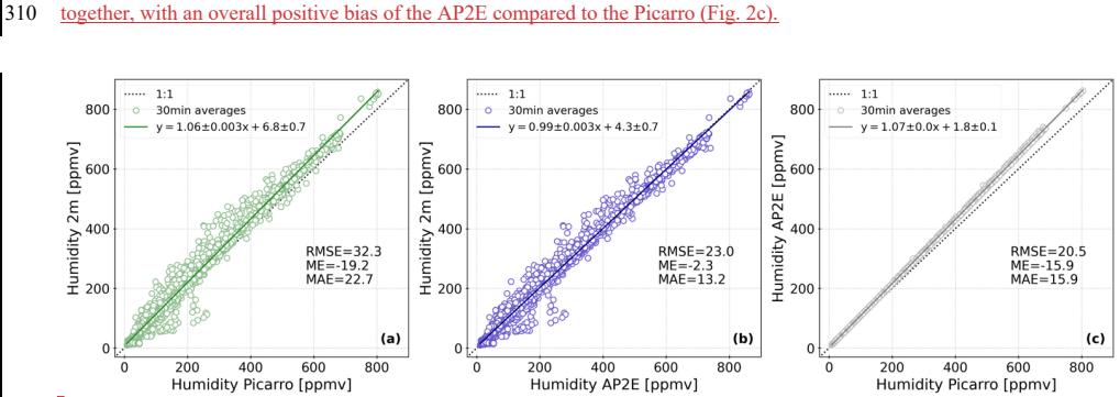
Figure 2: Comparison of the humidity (ppmv) measured by the two laser spectrometers (Picarro and AP2E) and by the independent sensor (modified HMP155, Sect. 2.2.1): (a) Picarro versus HMP155, (b) AP2E versus HMP155, and (c) Picarro versus AP2E. All available 30 min averages between January 1 st and March 15 th 2024 are shown in the figure. On each panel the root mean square error (RMSE, in ppmv), mean error (ME, analyser – HMP155 or Picarro – AP2E, in ppmv) and mean absolute error (MAE, in ppmv) calculated between the two humidity measurements are shown.
