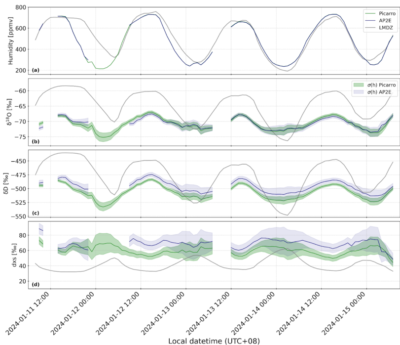
845 Figure 9: Zoom on the period from January 11 th to 15 th 2024 of the atmospheric humidity (in ppmv, panel (a)), \delta^{18}\text{O} (in ‰, panel (b)), \delta\text{D} (in ‰, panel (c)) and d-excess (in ‰, panel (d)) measured by the Picarro analyser (green lines), the AP2E analyser (blue lines), and modelled by LMDZ6-iso (grey lines). In panels (b) to (d), the green and blue shaded areas correspond respectively to \sigma(h) (Sect. 2.2.4) of the Picarro and AP2E analysers.
