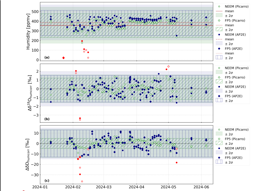
435 Figure 4: Results of the regular calibrations performed with two laboratory standards (FP5 and NEEM) between January 11 th and June 6 th with the new version of the LHLG (description in Sect. 2.2.2 and 2.2.3). Panel (a) shows the humidity measured by both analysers during each calibration. The red markers show the calibrations that were discarded (outside of two standard deviations around the mean humidity). Panels (b) and (c) show the measured isotopic ratios, corrected for the humidity-isotope response (Sect. 2.2.2 and 3.1.2), by both analysers during each calibration as a deviation of the mean over the whole period ( \Delta\delta^*_{i,humcorr} = \delta_{i,humcorr} - \delta_{i,humcorr,mean} subscript i is for each isotope species). The isotopic ratios of each calibration are corrected for the isotope-humidity response of each analyser. In panels (b) and (c), only the accepted calibration from panel (a) are shown. The red markers show the calibrations that are discarded in a second step (outside of two standard deviations around the mean isotopic ratio). 440
