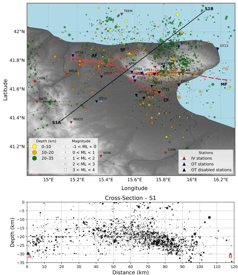
Figure 8. Maps of the epicenters of the H71 catalog with time with a cross section. Circle dimension is proportional to M_L in both map and vertical cross section as shown in the superimposed legend. Color refers to depth as indicated in the superimposed legend. Plot of the seismicity for the entire period, from April 2013 to December 2022
