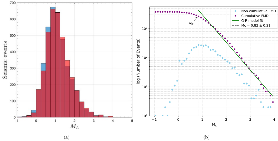
Figure 15. a) c2 Overlapped histograms of local magnitude M_L for the H71-catalog (orange+red areas), NLL-catalog (blue+red areas). c3 The areas in red color should be considered as common parts for both the H71 and NLL catalogs.. b) Frequency magnitude distribution (FMD) for the H71 catalog. Green line is the fit of the Gutenberg-Richter law between the computed M_C and the maximum magnitude of the catalog. Blue diamonds and purple circles are, respectively, the non-cumulative and cumulative frequency magnitude distribution.
