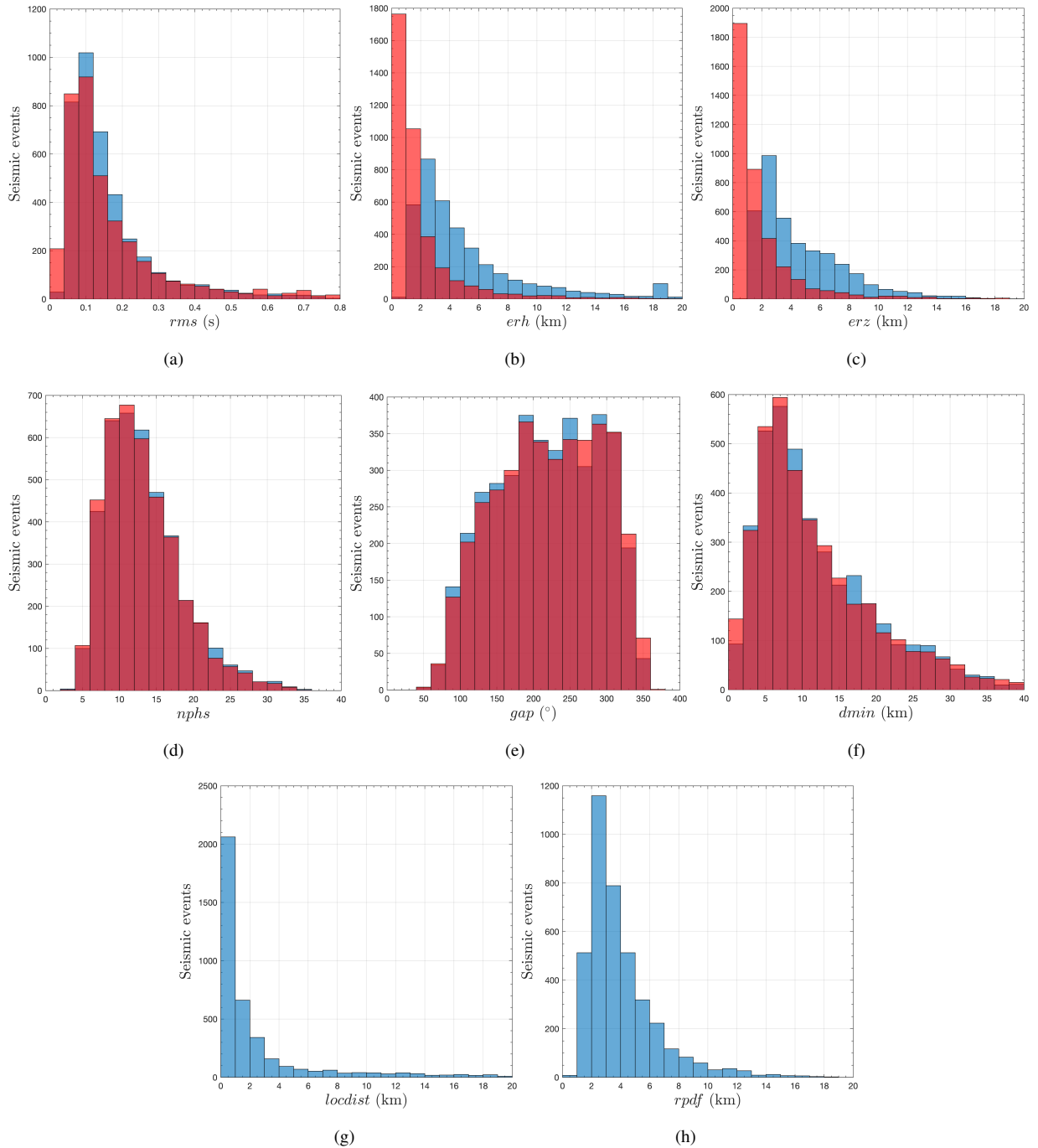
Figure 10. c1 Overlapped histograms of quality location estimators for the H71-catalog ( c2 orange+red areas) and NLL-catalog ( c3 blue+red areas) c4 . c5 The areas in red color should be considered as common parts for both the H71 and NLL catalogs.
