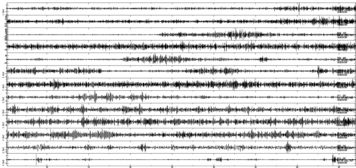
Figure 4. Example of false event c5 FE picked by CASP. c6 The Z components of the 13 stations that detected the false events are shown. Vertical axes are "Velocity" in counts/sec; horizontal axis is "Time" in sec from the begin time indicated on the trace.
