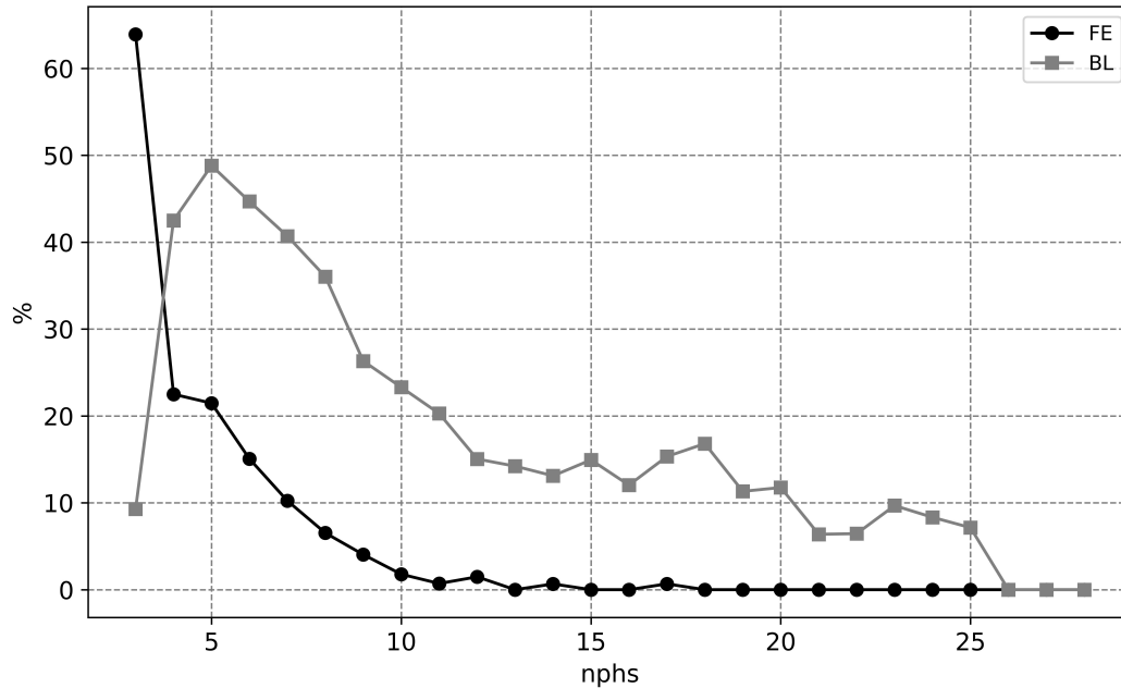
Figure 6. Curves of percentage of BL and of FE (gray and black respectively) respect to the number of AL plotted versus the number of phases used by CASP for the detection.
