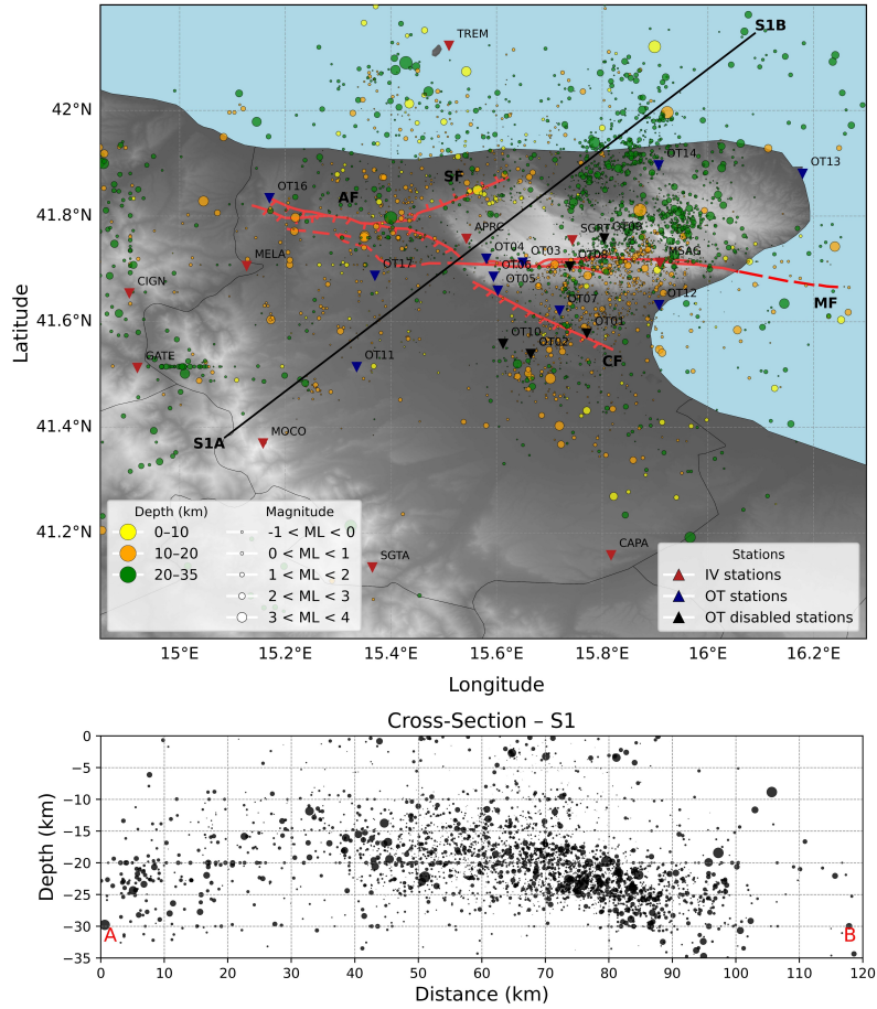
Figure 8. Maps of the epicenters of the H71 catalog with time c_1 with a cross section. Circle dimension is proportional to M_L c_2 in both map and vertical cross section as shown in the superimposed legend. Color refers to depth as indicated in the superimposed legend. Plot of the seismicity for the entire period, from April 2013 to December 2022
