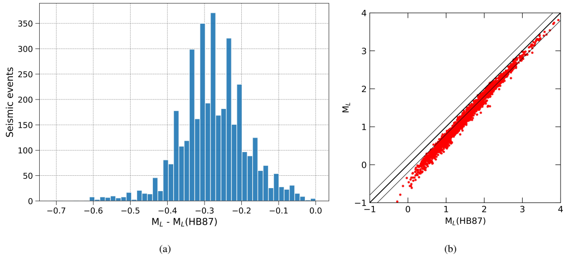
Figure 16. c1 Local magnitudes computed with two different attenuation functions: M_L which refers to Di Bona (2016) and M_L(\text{HB87}) which refers to Hutton and Boore (1987), are compared with each other. (a) Histogram of the difference M_L - M_L(\text{HB87}) computed for each EQ of the NLL-catalog. (b) plot of M_L vs M_L(\text{HB87}) for each EQ of the NLL-catalog with the lines M_L = M_L(\text{HB87}) and M_L = M_L(\text{HB87}) \pm 0.2 also plotted.
