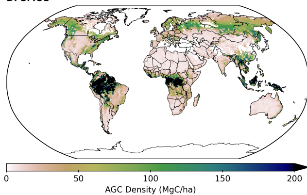
Figure S2. Comparison of the mean spatial distribution in AGC from 2017 to 2020 between our study and three other AGC products.
