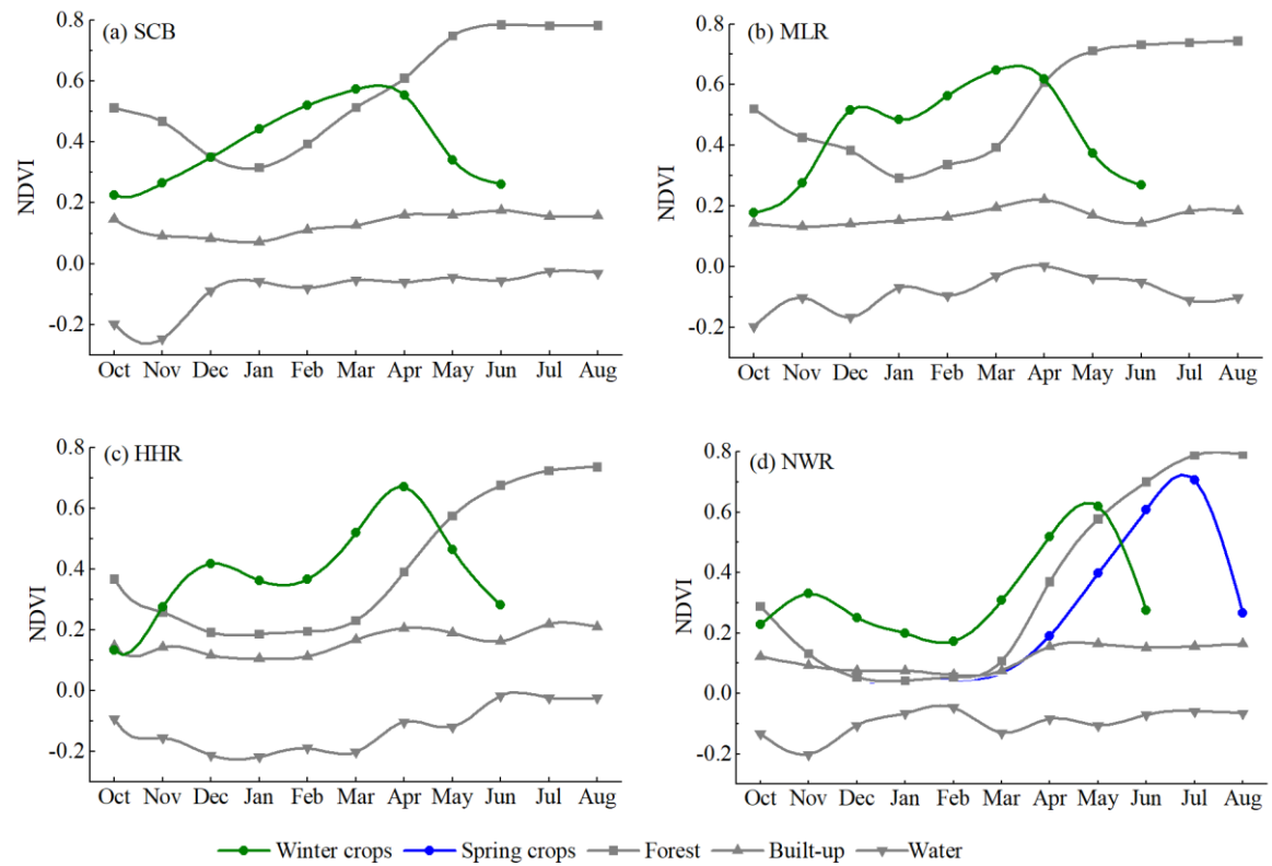
Figure 6: NDVI curves for different land cover types.
