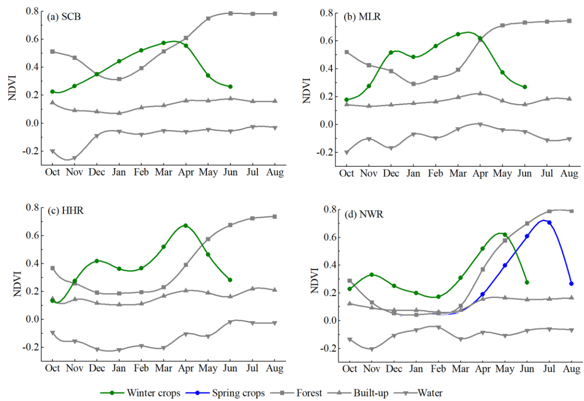
Figure 6: NDVI curves for different land cover types.
