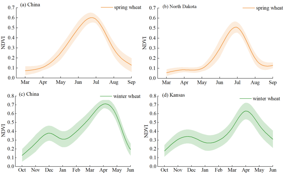
Figure 3: Comparison of NDVI time series curves between spring and winter wheat in China and the United States.
