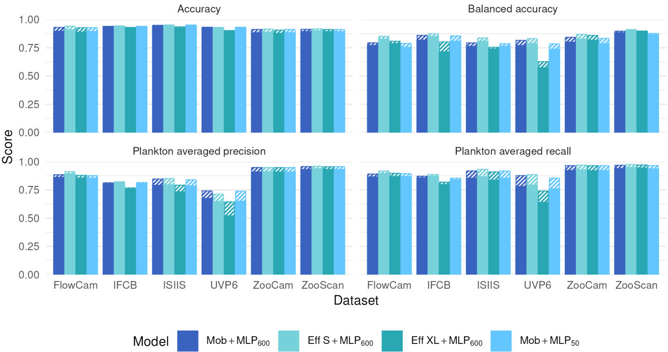
Figure 3: Performance comparison between our reference CNN (Mob + MLP600), a CNN with a larger feature extractor (Eff S + 410 MLP600 and Eff XL + MLP600) and a MobileNet followed by a smaller MLP (Mob + MLP50) on all six datasets. The models are described in Fig. 1. Plain bars show the value of each metric at the finest taxonomic level, striped bars show the value after regrouping objects into broader ecological groups. All values, including F1-scores, are reported in Table S8.
