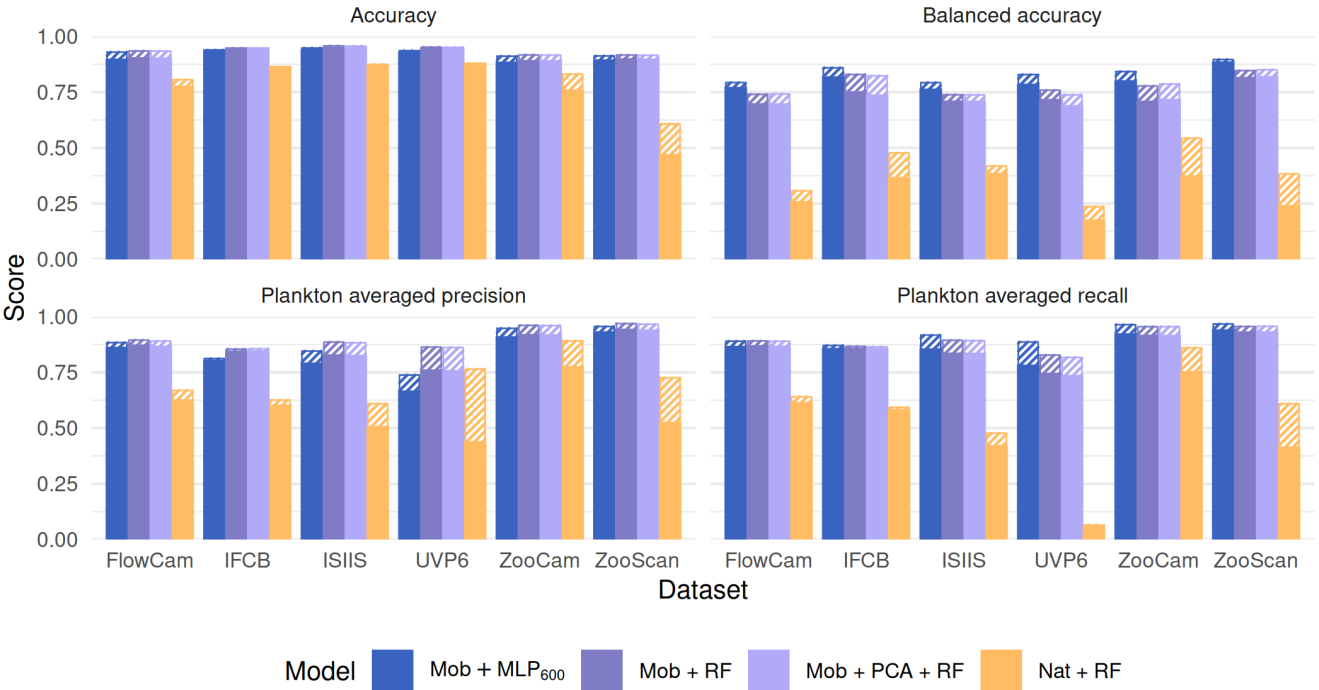
415 Figure 4: Performance comparison between our reference CNN (Mob + MLP600), a RF trained on deep features extracted by a MobileNet V2 without (Mob + RF) and with (Mob + PCA + RF) feature reduction, and a RF trained on handcrafted features on all six datasets. The models are described in Fig. 1. Plain bars show the value of each metric at the finest taxonomic level, striped bars show the value after regrouping objects into broader ecological groups.
