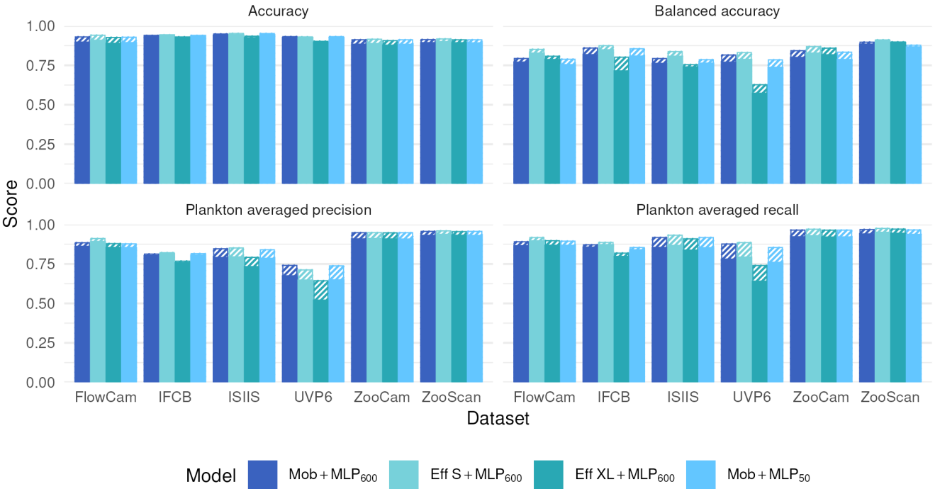
400 Figure 3: Performance comparison between our reference CNN (Mob + MLP600), a CNN with a larger feature extractor (Eff S + MLP600 and Eff XL + MLP600) and a MobileNet followed by a smaller MLP (Mob + MLP50) on all six datasets. The models are described in Fig. 1. Plain bars show the value of each metric at the finest taxonomic level, striped bars show the value after regrouping objects into broader ecological groups.
