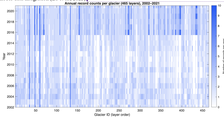
Fig. 9: Ice front positions delineation density (2002–2021) for 465 Greenland glaciers. Each column represents a glacier, each row a calendar year, and the colour scale indicates the number of manually digitized ice front positions per glacier per year.
