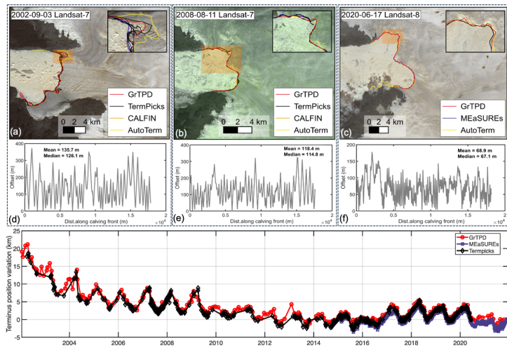
810 Fig. 5: Spatial and quantitative comparison of calving fronts for Jakobshavn Isbræ Glacier at three representative dates (2002-09-03, 2008-08-11, 2020-06-17). (a–c) show GrTPD (red) alongside TermPicks (black), CALFIN (orange), AutoTerm (yellow) and MEaSUREs (blue). Insets highlight zones of mélange or lateral embayment complexity. (d–f) plot the along-front offset distributions. (d) and (e) show comparisons between this dataset and TermPicks, corresponding to (a) and (b), respectively. (f) compares this dataset with MEaSUREs, corresponding to (c). Each profile displays both the average and median offsets. (g) presents the time series of manually delineated ice front position variation (km) from 2002 through 2021.
