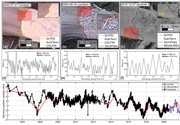
840 Fig. 7: Multi-temporal assessment of Helheim calving front positions on 2002-07-27, 2005-09-14 and 2015-12-07. (a-c) overlay GrTPD (red) with TermPicks (black), CALFIN (orange), AutoTerm (yellow) and MEaSUREs (blue) on Landsat and Sentinel-1 images; zoomed insets show areas of high morphological complexity. Panels (d-f) illustrate along-front offset profiles for each date. (d) show comparisons between this dataset and CALFIN, corresponding to (a). (e) and (f) compares this dataset with TermPicks, corresponding to (b) and (c), respectively. Each profile displays both the average and median offsets. (g) presents the time series of manually delineated calving front position variation (km) from 2002 through 2021.
