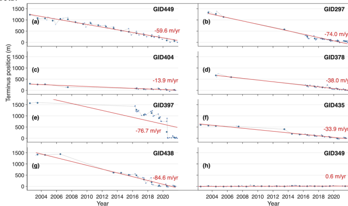
960 Fig. 10: Time series of terminus position change for several lake-terminating glaciers in Greenland derived from the GrTPD dataset. For each glacier, terminus positions are projected along the glacier-specific centerline to quantify frontal migration relative to a fixed upstream reference. Blue points indicate individual terminus observations with temporal sampling varying according to satellite availability. Annual mean positions are shown as filled circles, and red lines indicate linear trends with annotated rates (m/yr).
