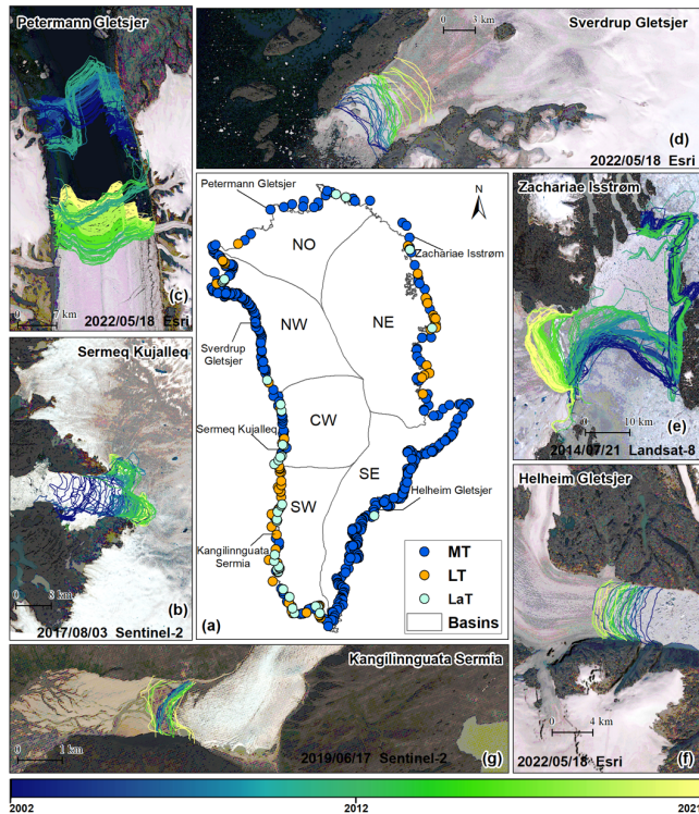
350 Fig. 1: Spatial overview of the glaciers included in this dataset. Central panel (a) shows glacier locations grouped by drainage basin (Rignot and Mouginot, 2012). Coloured points indicate the glaciers included in the dataset: marine-terminating glaciers (MT, blue), land-terminating glaciers (LT, orange), and lake-terminating glaciers (LaT, turquoise). Surrounding maps illustrate (b–g) six examples of temporally resolved ice front positions (colour-coded by year) derived from multi-source imagery.
