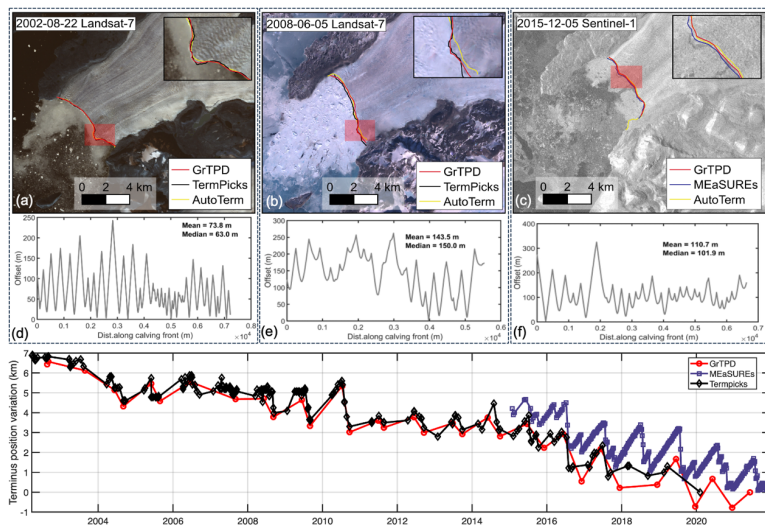
Fig. 8: Multi-temporal assessment of Sverdrup Gletsjer calving front positions on 2002-08-22, 2008-06-05 and 2015-12-05. (a–c) overlay our manual fronts (red) with TermPicks (black), AutoTerm (yellow) and MEaSUREs (blue) on Landsat and Sentinel-1 images; zoomed insets show areas of high morphological complexity. Panels (d–f) illustrate along-front offset profiles for each date. (d) and (e) show comparisons between this dataset and TermPicks, corresponding to (a) and (b), respectively. (f) compares this dataset with MEaSUREs, corresponding to (c). Each profile displays both the average and median offsets. (g) presents the time series of manually delineated calving front position variation (km) from 2002 through 2021.
