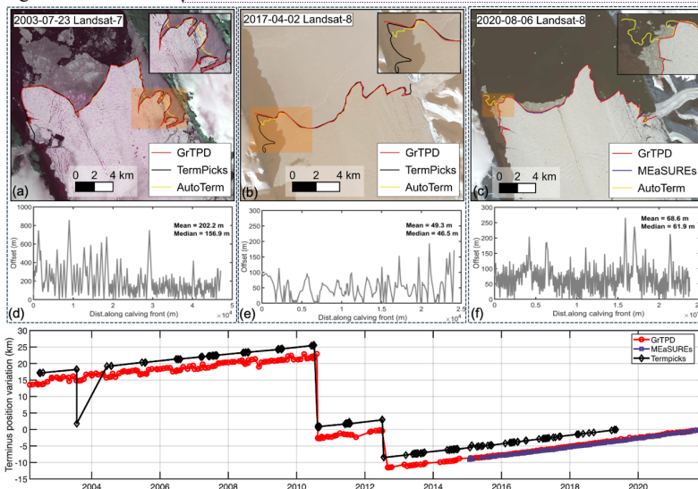
Fig. 4: Comparison of delineated calving fronts for Petermann Gletsjer on three dates (2003-07-23, 2017-04-02 and 2020-08-06). (a–c) overlay GrTPD (red) with TermPicks (black), AutoTerm (yellow) and MEaSUREs (blue) on Landsat scenes; insets zoom in on areas of complex mélange cover or irregular geometry. (d–f) show the along-front offset profiles (AMD) for each date. (d) and (e) show comparisons between this dataset and TermPicks, corresponding to (a) and (b), respectively. (f) compares this dataset with MEaSUREs, corresponding to (c). Each profile displays both the average and median offsets. (g) presents the time series of manually delineated ice front position variation (km) from 2002 through 2021.
