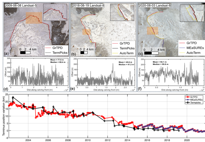
825 830 Fig. 6: Multi-temporal assessment of Zachariae Isström calving front positions on 2009-08-08, 2018-08-19 and 2020-08-03. (a–c) overlay GrTPD (red) with TermPicks (black), AutoTerm (yellow) and MEaSURES (blue) on Landsat images; zoomed insets show areas of high morphological complexity. Panels (d–f) illustrate along-front offset profiles for each date. (d) and (e) show comparisons between this dataset and TermPicks, corresponding to (a) and (b), respectively. (f) compares this dataset with MEaSURES, corresponding to (c). Each profile displays both the average and median offsets. (g) presents the time series of manually delineated calving front position variation (km) from 2002 through 2021.
