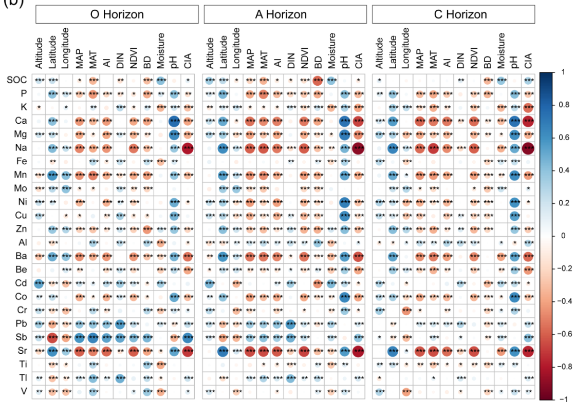
Fig. 5 The environmental factors influencing the elemental concentrations in the soils. (a) Redundancy analysis (RDA) shows the relationships of soil elements with environmental factors across soil horizons. The inserted figure shows the distribution of samples along the axes. (b) Correlation heatmap shows the correlation between soil element concentrations and environmental variables in each soil horizon. The color and circle size represent the correlation coefficient, and * indicates statistical significance ( p < 0.05 ). SOC, soil organic carbon; MAP, mean annual precipitation; MAT, mean annual temperature; AI, aridity index; DIN, dissolved inorganic nitrogen; NDVI, normalized difference vegetation index; BD, bulk density; CIA, chemical index of alteration
