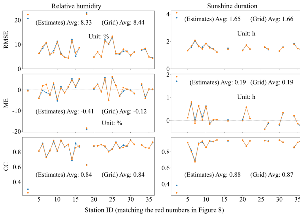
425 Figure 11: Comparison of dotted line plots for RMSE, ME, and CC between in-situ data and station-based estimates, as well as 430 between in-situ data and gridded data.
