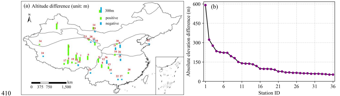
Figure 10: Elevation differences between station elevations and corresponding DEM grid values: (a) spatial distribution, where red numbers denote station IDs with differences greater than 50 m; (b) point-line plot showing absolute elevation differences as a function of station ID.
