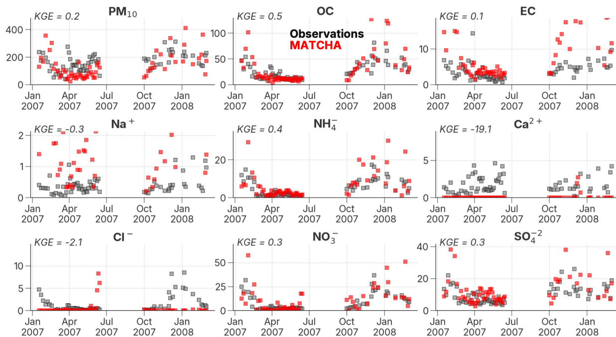
1640 Figure 17: Observed (black) versus MATCHA-simulated (red) daily averaged (between 0600–1800 IST) concentrations (in \mu\text{g}/\text{m}^3 ) of total \text{PM}_{10} and eight chemical species at Kanpur (26.5° N, 80.3° E) from January 2007 to March 2008.
