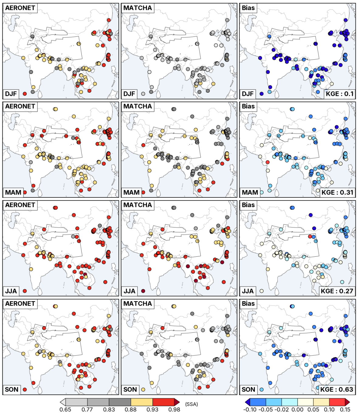
1615 Figure 12: Seasonal averages of SSA at 550 nm (unitless) from AERONET sites across the domain (left column), from MATCHA (middle), and the associated model bias (MATCHA-AERONET, right column).
