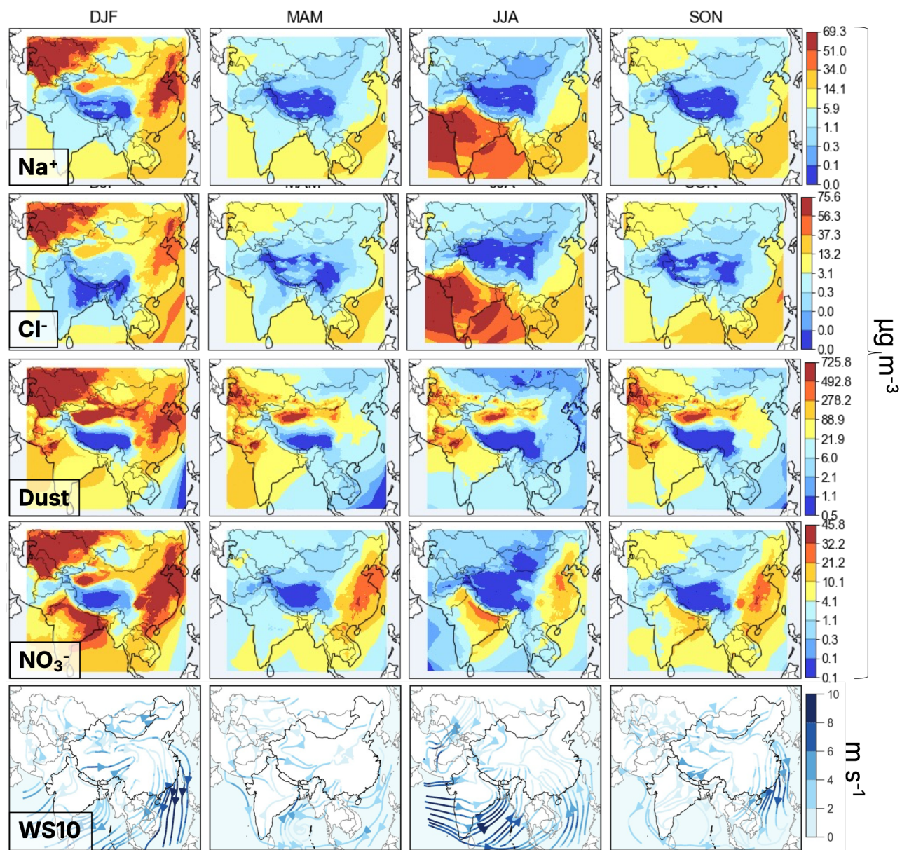
Figure A4: Seasonal averages of surface sea-salt partitioned to sodium and chloride (in \mu\text{g/m}^3 ), surface nitrate aerosols (in \mu\text{g/m}^3 ), surface dust (in \mu\text{g/m}^3 ) and wind speed at 10 m (in \text{m/s} ) over the model domain.
