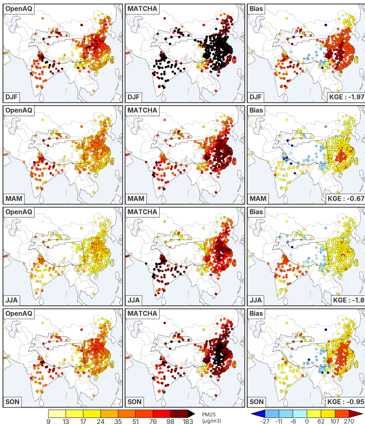
Figure 13: Seasonal averages of surface PM 2.5 (in µg/m 3 ) across the domain from OpenAQ (left column), MATCHA (middle), and the associated model bias (MATCHA-OpenAQ, right column).
