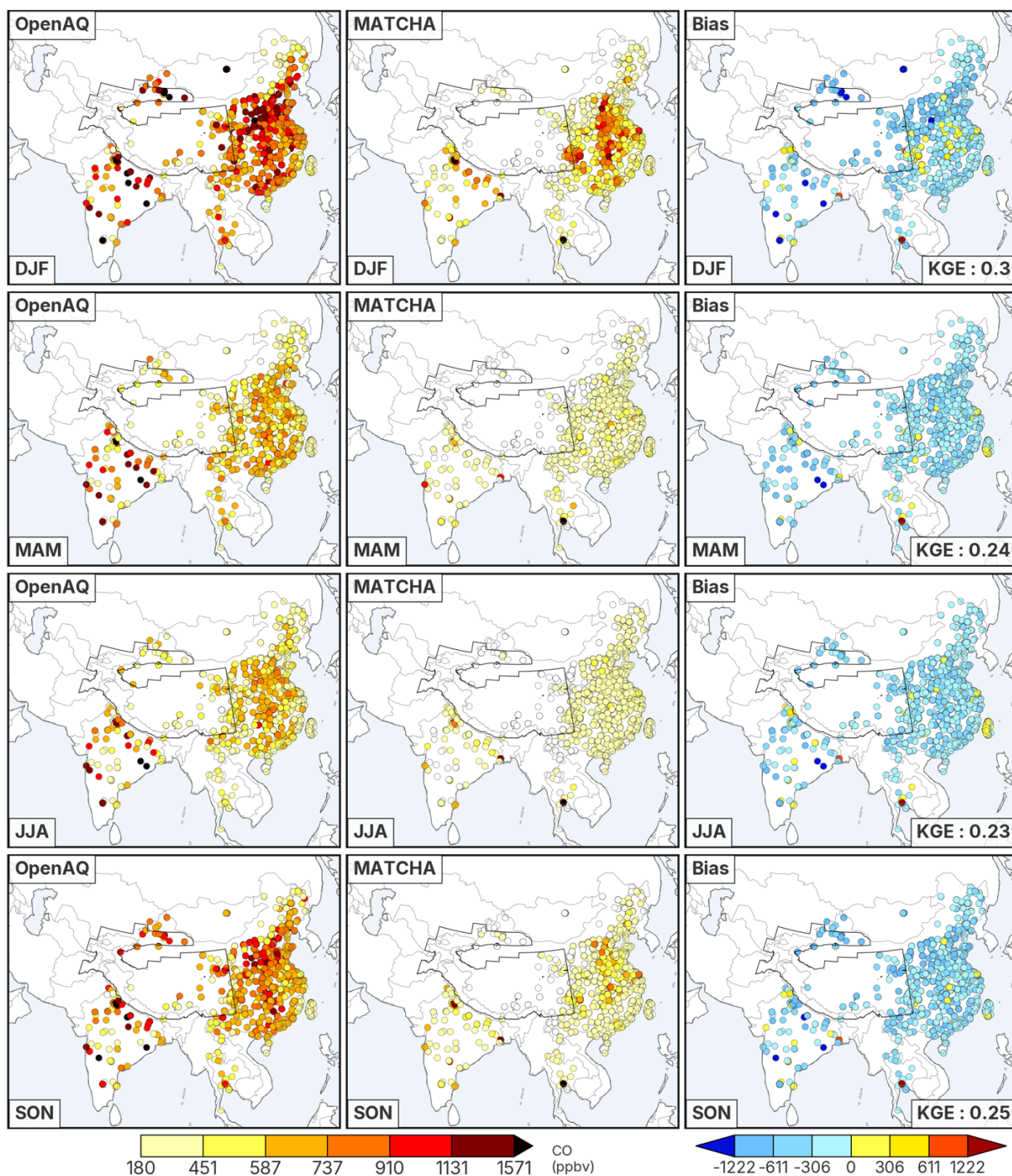
1630 Figure 15: Seasonal mean of surface CO (in ppbv) across the domain from OpenAQ (left column), MATCHA (middle), and the associated model bias (MATCHA-OpenAQ, right column).
