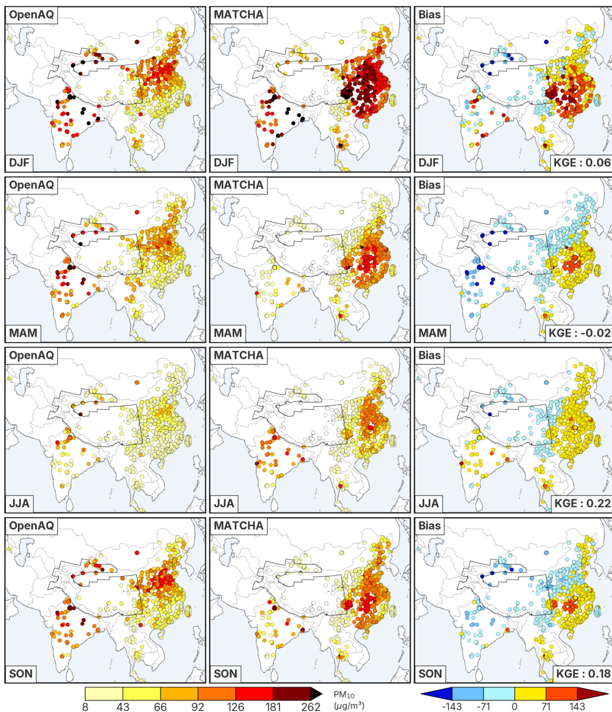
1625 Figure 14: Seasonal averages of adjusted surface PM_{10} (after removing surface sea salt and dust) (in \mu g/m^3 ) across the domain from OpenAQ (left column), MATCHA (middle), and the associated model bias (MATCHA-OpenAQ, right column).
