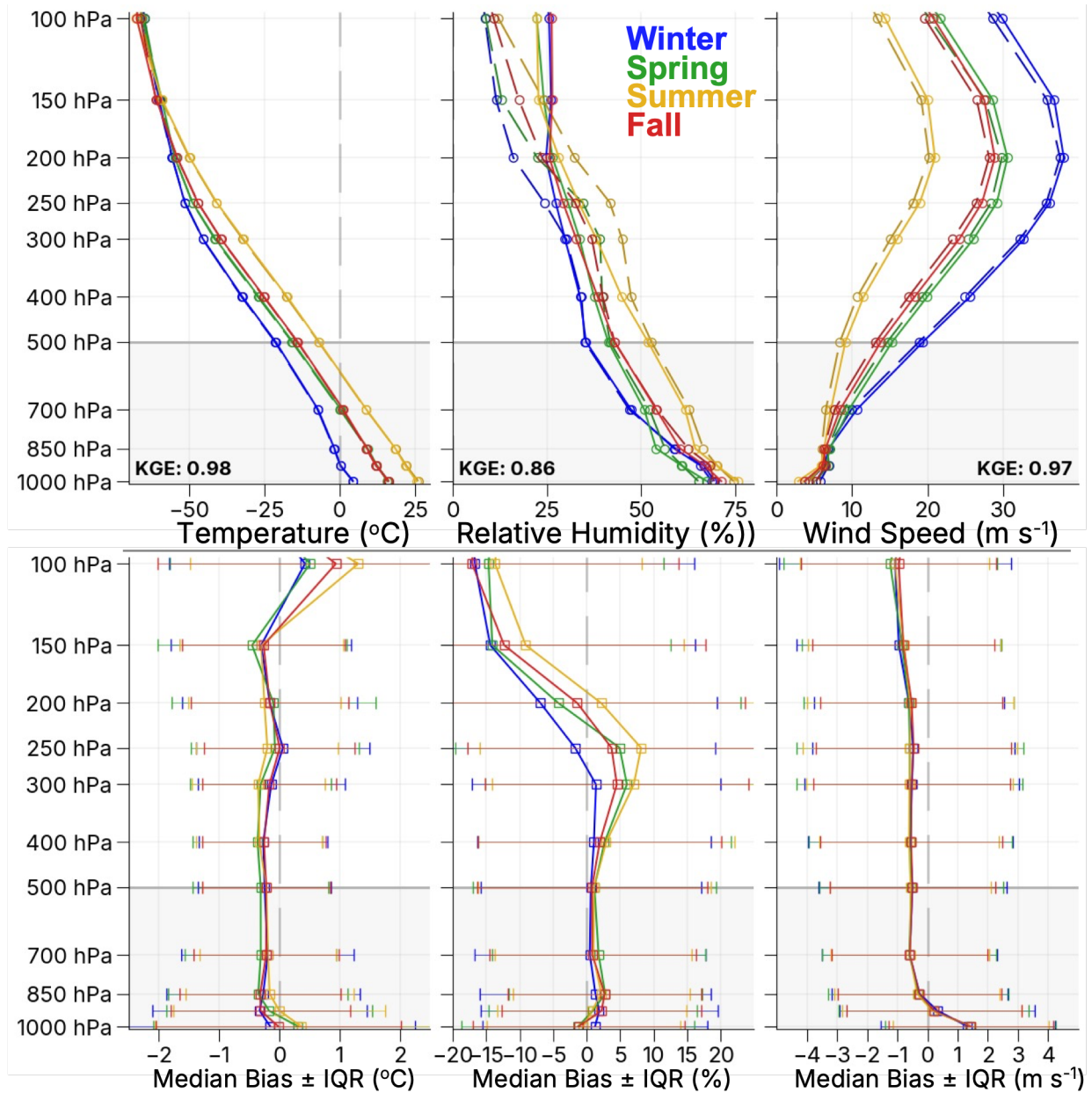
1580 Figure 4: Seasonal averages of temperature, relative humidity, and wind speed profiles across the domain (top panel) from the IGRA radiosonde archive, and their relative biases (MATCHA-IGRA) in the bottom panel. The dashed lines in the top panel refer to profiles from MATCHA, while the solid lines refer to profiles from IGRA. Horizontal error bars in the bottom panel correspond to the interquartile range of the relative bias across all sites.
