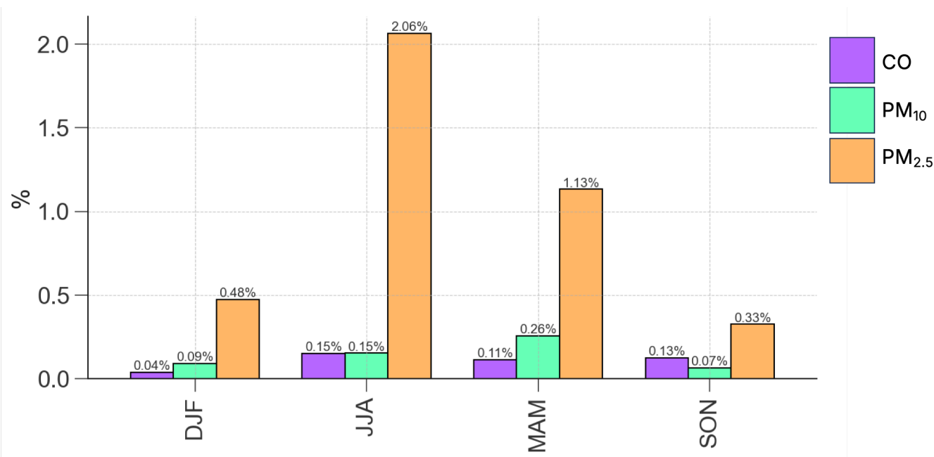
Figure A1: Percentage of outliers removed from retrieved OpenAQ data of surface CO, PM 10 , and PM 2.5 (purple, green and orange, respectively) using the outlier detection system in Wu et al., 2018 (see main text).
