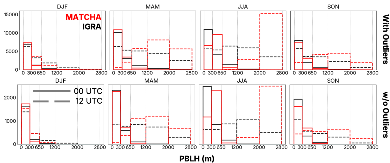
Figure A2: Histograms of both model (red) and observed (black) PBLH values compared across seasons and standard radiosonde launch times (solid for 00 UTC and dashed for 12 UTC) before and after applying the outlier-detection approach 955 described in Section 2.2.4 of the main text.
