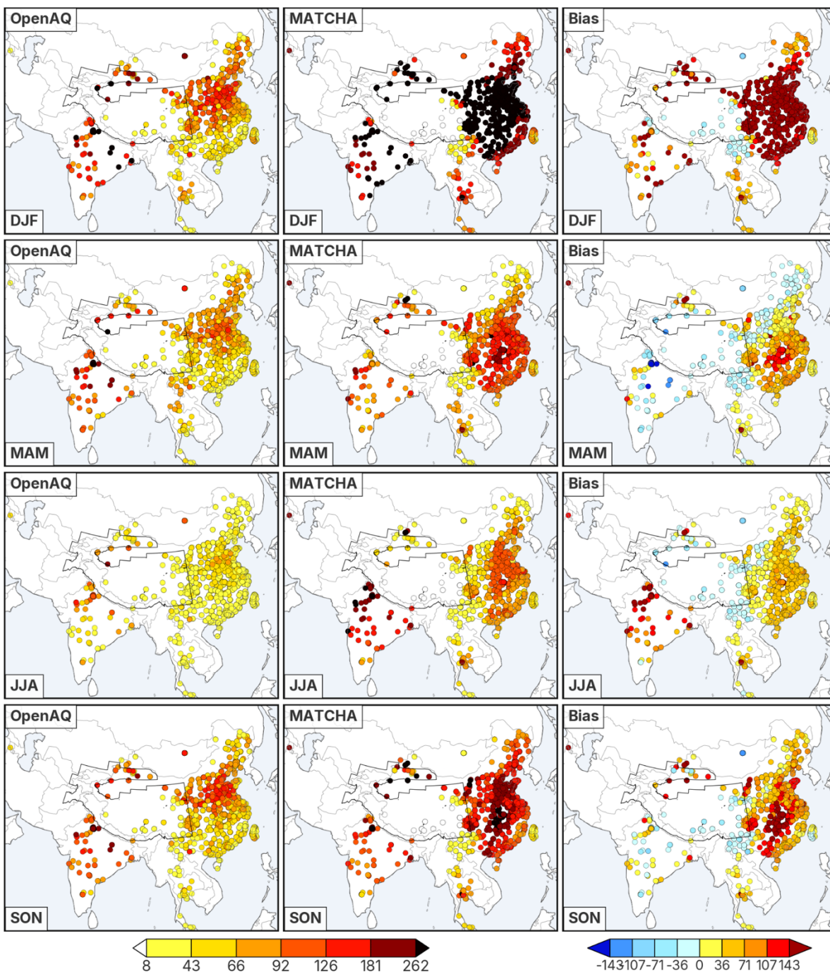
Figure A5. Seasonal averages of total surface PM 10 (in \mu\text{g}/\text{m}^3 ) across the domain from OpenAQ (left column), MATCHA (middle), and the associated model bias (MATCHA-OpenAQ, right column).
