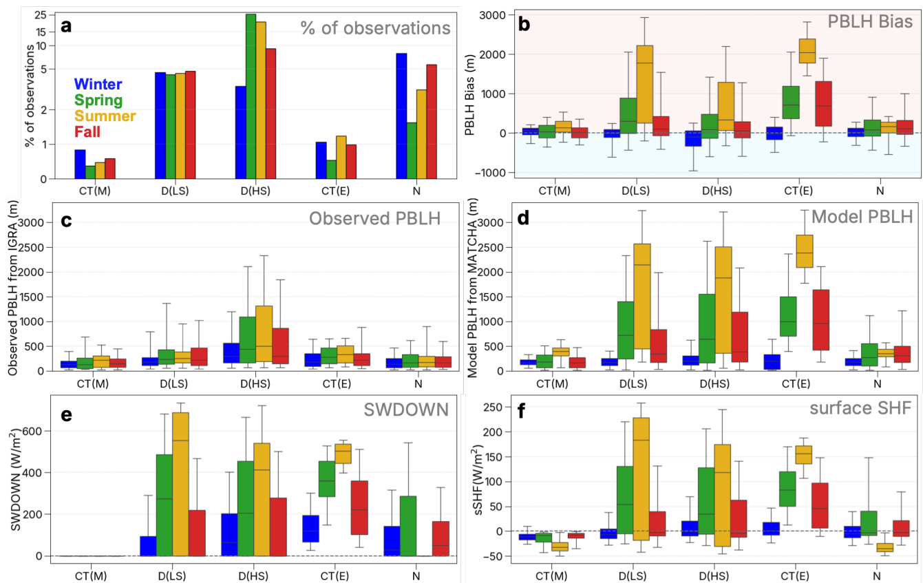
965 Figure A3: (a) Fraction (in %) of all 00 UTC and 12 UTC radiosonde launches in the domain across different solar regimes (CT(M) = Morning Civil Twilight; D(LS) = Day – Low Sun; D(HS) = Day – High Sun; CT(E) = Evening Civil Twilight; N = Night) for each season. Solar regimes were defined by computing the solar elevation angle at the exact launch time of each radiosonde observations and classifying them into five exclusive categories: N ( \leq -6^\circ ), CT ( -6^\circ to 0^\circ , split into morning or evening by solar azimuth), D (LS) ( 0^\circ to 10^\circ ), and D(HS) ( > 10^\circ ). (b) PBLH bias (model-observed), (c) observed PBLH, 970 and (d) modeled PBLH from IGRA and MATCHA across the solar regimes and seasons. (e) Downward shortwave radiation flux (SWDOWN) and (f) surface sensible heat flux (sSHF) collocated at IGRA sites from MATCHA across solar regimes and seasons.
