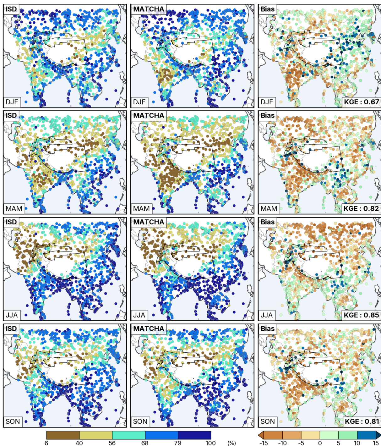
1585 Figure 5: Seasonal averages of relative humidity at 2 m (in %) from the ISD archive (left column), MATCHA (middle column), and the associated model bias (MATCHA - ISD, right column).
