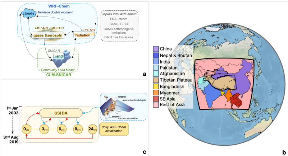
Figure 1: The MATCHA framework. (a) Schematic representation of the model setup in MATCHA. Within WRF-Chem (blue box), gas-phase chemistry and aerosols (MOZART-MOSAIC) are coupled to radiation (RRTMG), clouds (Morrison double-moment microphysics), and the land surface (CLM with the SNICAR snow-radiation module; green box), with grey arrows denoting the exchange of fields between components. External forcings (grey dashed box) comprise emission inputs as well as meteorological and chemical initial and boundary conditions. (b) the 10 tagged source regions for anthropogenic BC over the entire study domain. (c) the assimilation workflow used in MATCHA, where MODIS AOD and MOPITT CO profiles were assimilated every 3 hours into the WRF-Chem-CLM-SNICAR model for the 17 years of simulation period. The model advances through successive 3-hour windows daily. Blue arrows show MODIS AOD and MOPITT CO retrievals together with the model background state, ingested into the GSI data assimilation system; red arrows show the analysis returned to WRF-Chem and the re-initialization carrying the model state at the end of the day into the next day's 0 UTC cycle.
