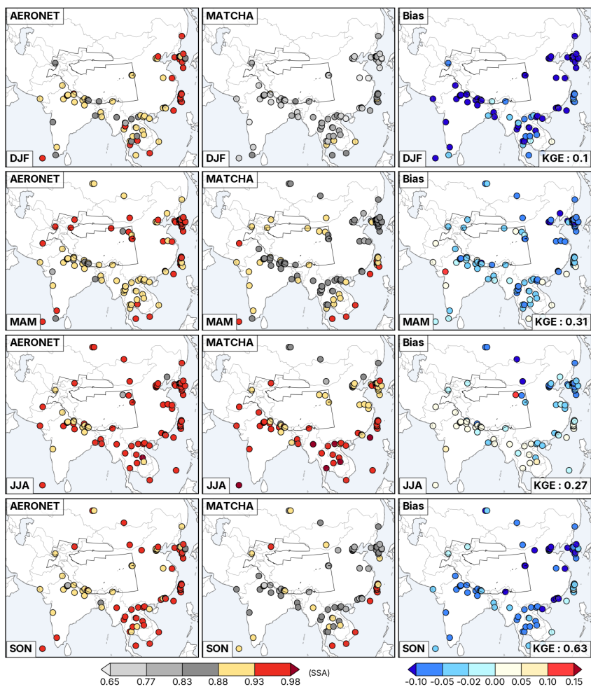
1710 Figure 12: Seasonal averages of SSA at 550 nm (unitless) from AERONET sites across the domain (left column), from MATCHA (middle), and the associated model bias (MATCHA-AERONET, right column).
