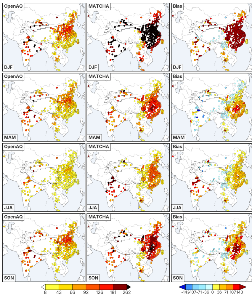
Figure A5. Seasonal averages of total surface PM10 (in \mu\text{g}/\text{m}^3 ) across the domain from OpenAQ (left column), MATCHA (middle), and the associated model bias (MATCHA-OpenAQ, right column).
