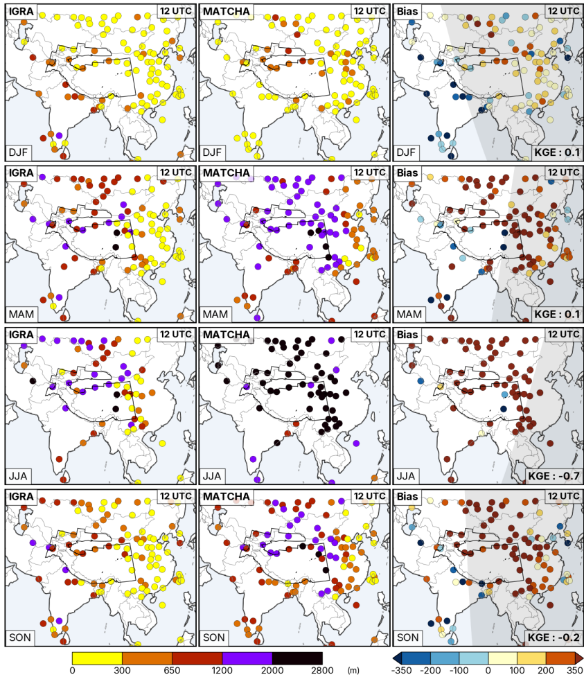
Figure 9: Seasonal mean of boundary layer height at approximately 12 UTC from the IGRA archive (left column), MATCHA (middle column), and the associated model bias (MATCHA - IGRA, right column). The shadow zones show parts of the domain with nighttime conditions depending on the solar elevation angle on the 15 th of the months; January (for DJF), April (for MAM), July (for JJA), and October (for SON), for the year 2003.
