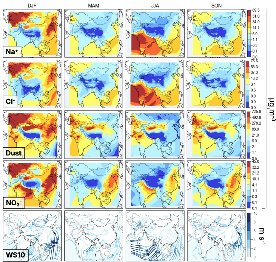
Figure A4: Seasonal averages of surface sea-salt partitioned to sodium and chloride (in \mu\text{g}/\text{m}^3 ), surface nitrate aerosols (in \mu\text{g}/\text{m}^3 ), surface dust (in \mu\text{g}/\text{m}^3 ) and wind speed at 10 m (in \text{m}/\text{s} ) over the model domain.
