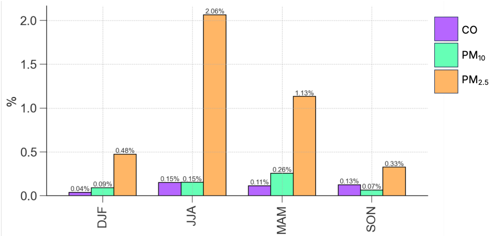
Figure A1: Percentage of outliers removed from retrieved OpenAQ data of surface CO, PM 10 , and PM 2.5 (purple, green and orange, respectively) using the outlier detection system in Wu et al., 2018 (see main text).
