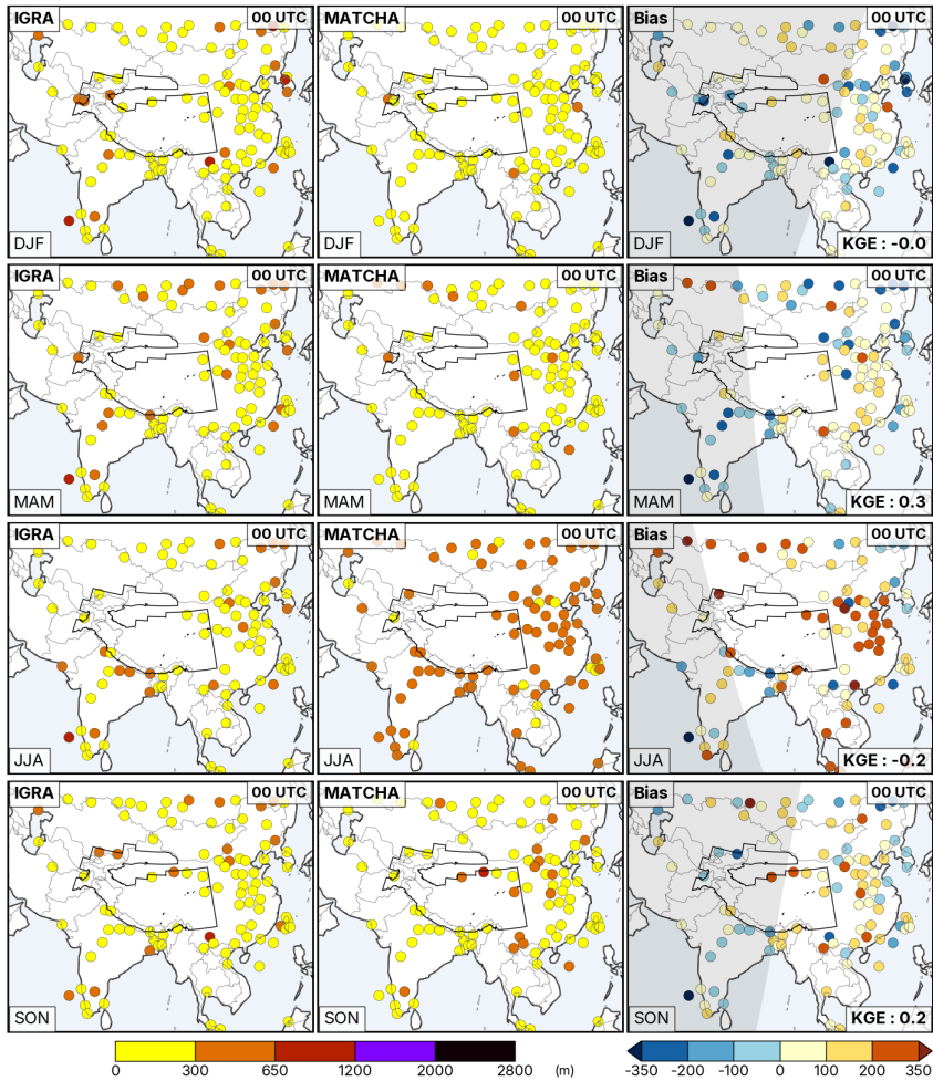
Figure 8: Seasonal averages of planetary boundary layer height at approximately 00 UTC from the IGRA archive (left column), MATCHA (middle column), and the associated model bias (MATCHA - IGRA, right column). The shadow zones show parts of the domain with nighttime conditions depending on the solar elevation angle on the 15 th of the months; January (for DJF), April (for MAM), July (for JJA), and October (for SON), for the year 2003.
