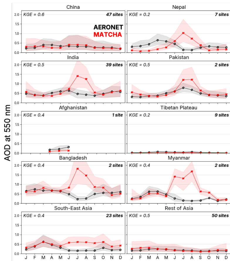
Figure A8: Monthly median AOD at 550 nm with their interquartile ranges across AERONET sites (black) compared with corresponding values from MATCHA (red) across the ten tagged tracer regions within MATCHA (defined in the main text).
