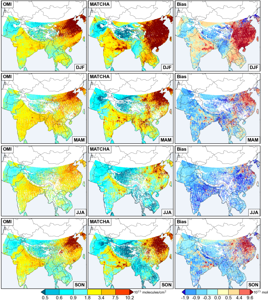
Figure A6: Seasonal averages for the year 2014 of tropospheric column NO 2 concentrations (molecules cm -2 ) from OMI satellite observations (L2 products) regridded to MATCHA's 12 km resolution (left column), MATCHA (middle column), and the associated model bias (MATCHA-OMI, right column).
