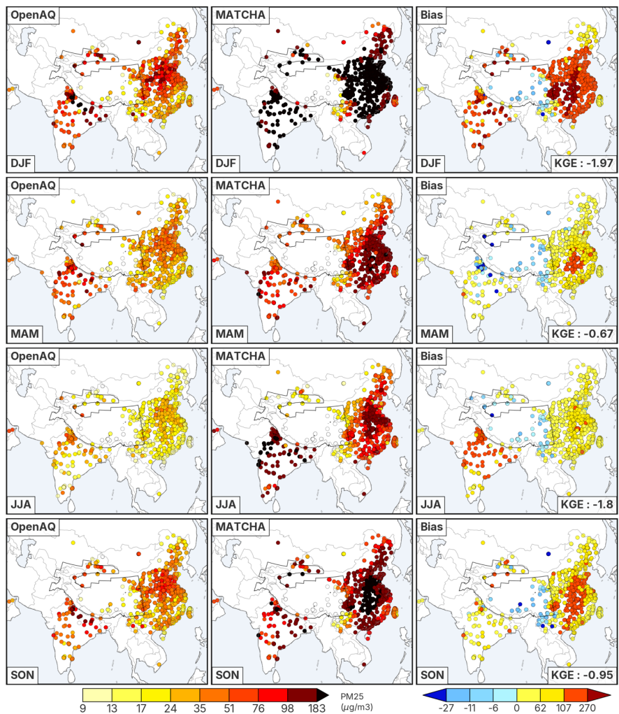
Figure 13: Seasonal averages of surface PM 2.5 (in \mu\text{g}/\text{m}^3 ) across the domain from OpenAQ (left column), MATCHA (middle), and the associated model bias (MATCHA-OpenAQ, right column).
