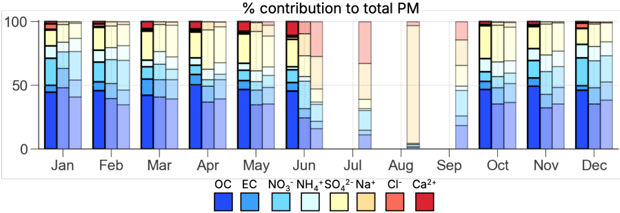
Figure A7: Monthly averaged percentage contribution of eight chemical species to total particulate matter over the Kanpur site based on ~1 year of observations from the site (first group of bars), ~1 year of model simulation over the site (second group) and 17-year contribution (third group) from the model simulation over the site.
