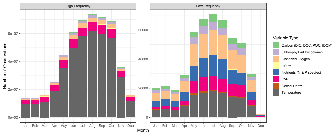
Figure 4. Temporal Distribution of observations in LakeBeD-US: Ecology Edition LakeBeD-US-EE. Colors represent categories of variables.
