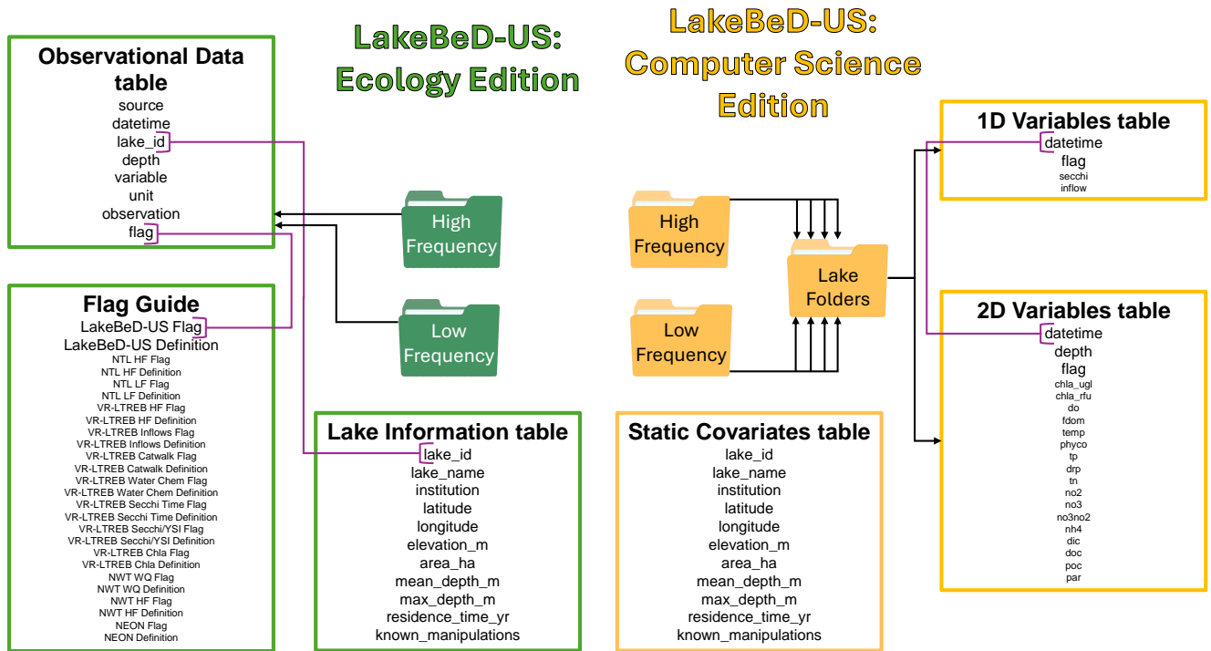
Figure 3. Structure of LakeBeD-US: Ecology Edition and LakeBeD-US: Computer Science Edition . Arrows indicate folder contents (e.g. LakeBeD-US: Ecology Edition contains High- and Low-Frequency folders that each contain an observational data table). Purple connectors indicate common columns by which to link tables. LakeBeD-US: Computer Science Edition contains High- and Low-Frequency Folders that each contain separate folders separating data from each lake. Each lake folder contains its own static covariate, 2D variables, and 1D variables tables.
