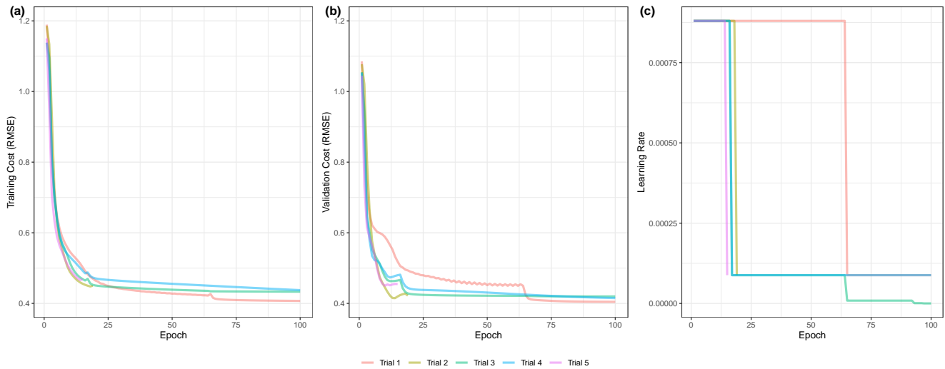
Figure 7. Training cost, validation cost, and learning rate of machine learning benchmark. The cost, a measure of model error, for the training (a) and validation (b) splits is shown as a function of the number of epochs. The learning rate, or amount of change between iterations of the model in response to error, is shown (c). Five trials are shown in different colors.
