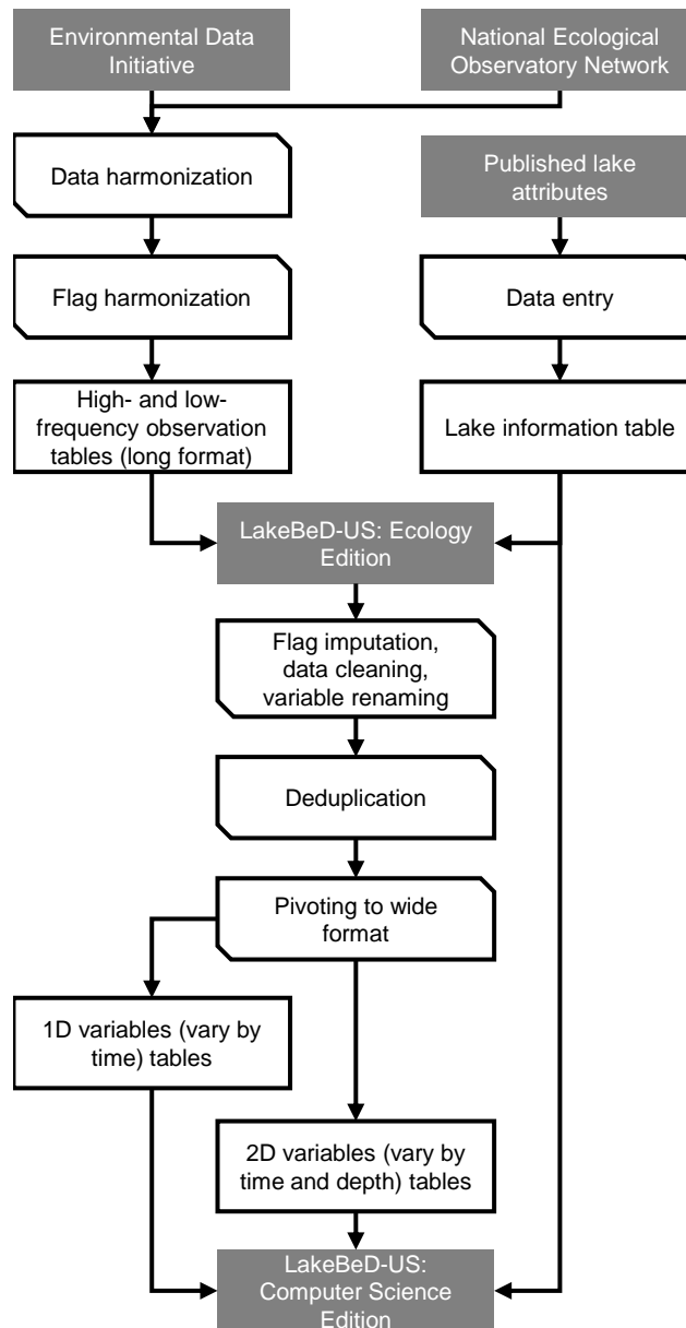
Figure 2. Harmonization workflow for LakeBeD-US. Boxes represent states of data and corner-snipped parallelograms represent processes. Grey boxes represent published products and sources of published products.
