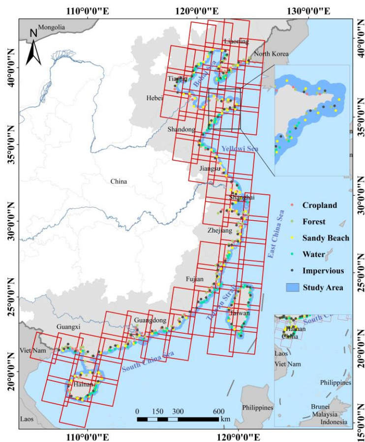
100 Figure 1: Location of China's coastal zone and distribution of partial typical land feature points for results verification.
