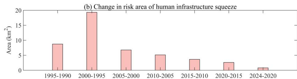
Figure 10: Interannual changes in human infrastructure squeeze on sandy beaches: (a) Risk area of human infrastructure squeeze from 1990 to 2024, (b) Changes in risk area of human infrastructure squeeze from 1990 to 2024.
