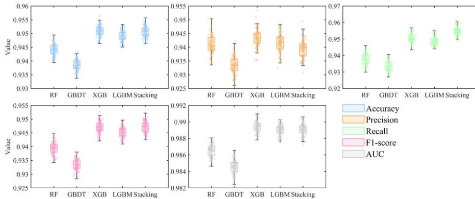
Figure 13: Comparison of F1-score and overall accuracy across models.
