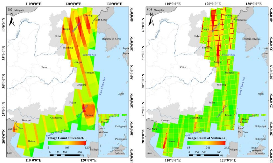
Figure 2: Spatial distribution of Sentinel-1 and Sentinel-2 images used in this study from 2016 to 2024: (a) Image Count of Sentinel-1, (b) Image Count of Sentinel-2.
