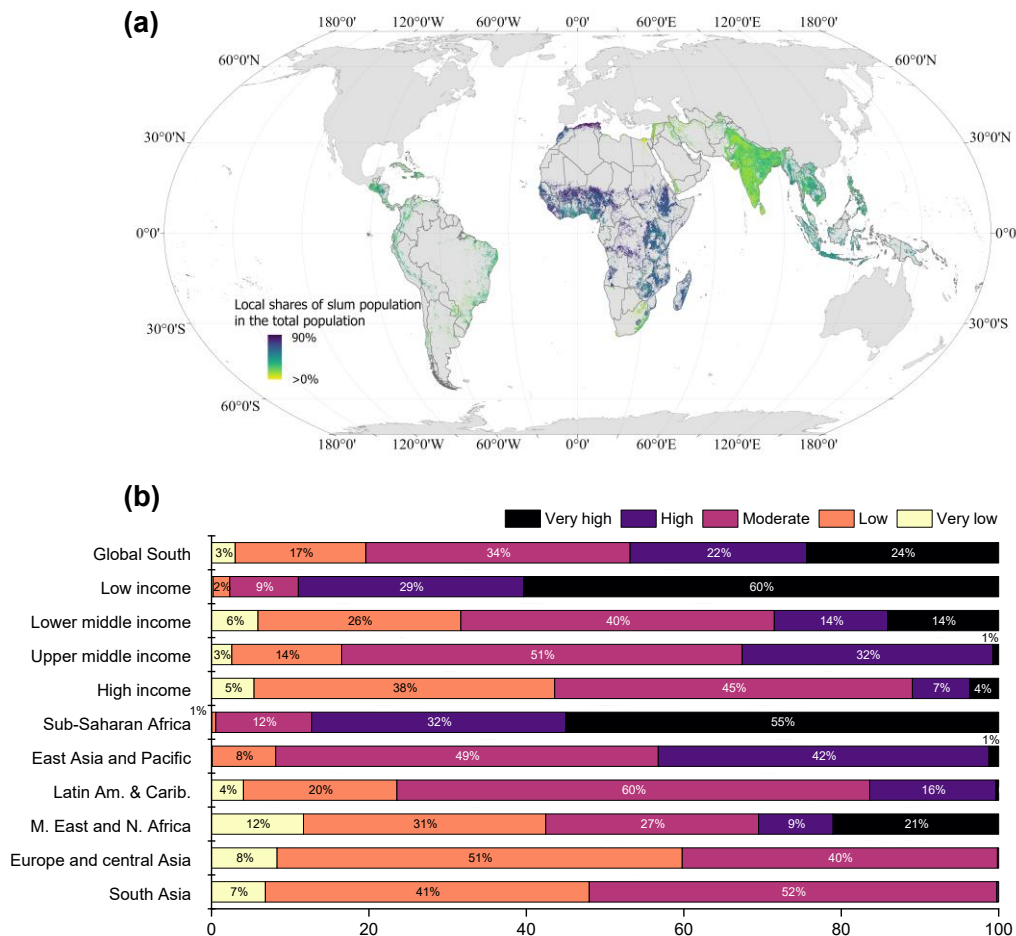
Figure 5 Slum populations categorized by concentration levels, ranging from very low to very high, and their geographic and socioeconomic disparities. (a) Map displaying
