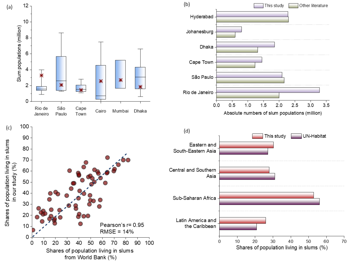
Figure 8 Comparison of our slum population estimates with data from previous literature and official statistics, presented as both absolute numbers and relative
