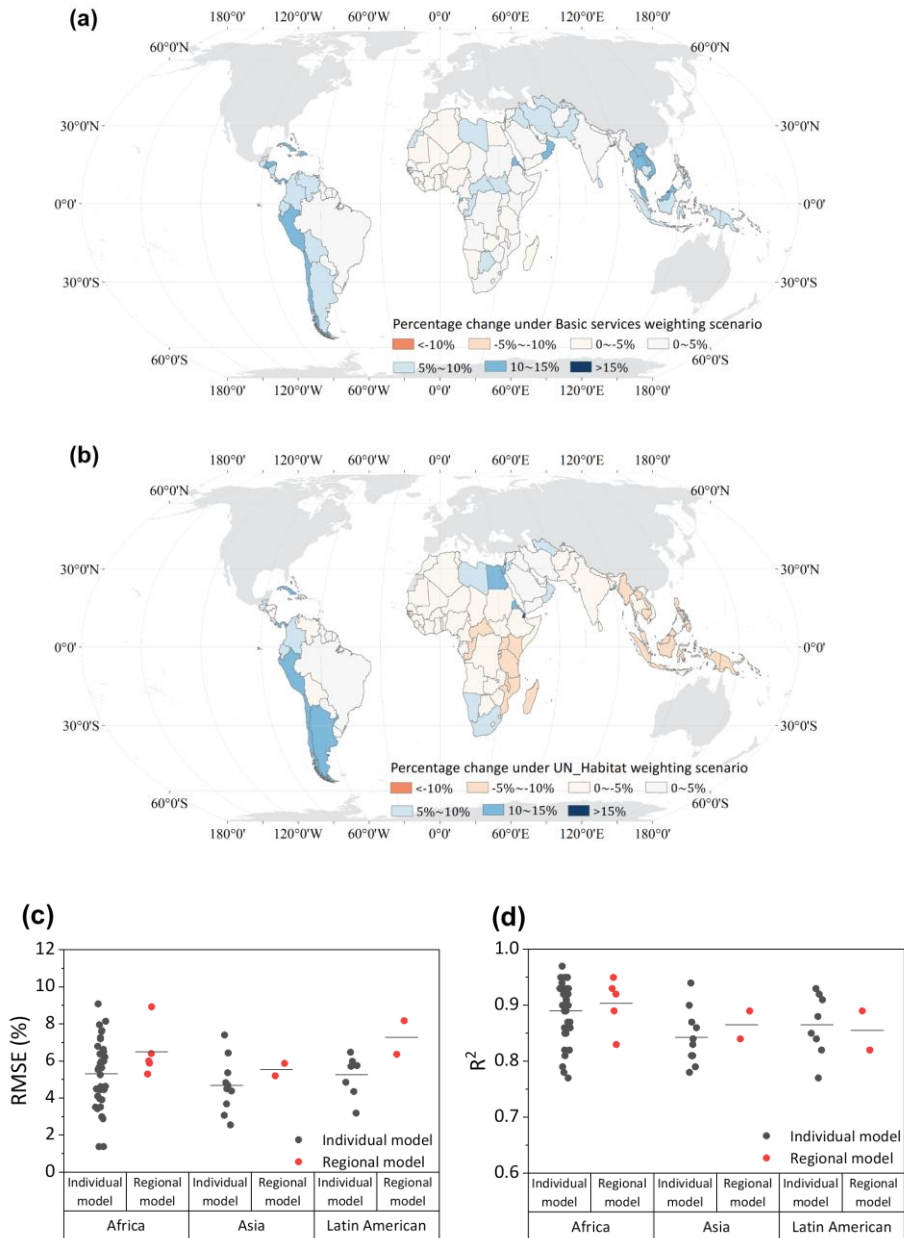
Figure 7 Differences in slum population estimates across two alternative weighting schemes and comparison of model performance between regional models and country-specific models. Panels (a) and (b) show the percentage change in slum population estimates under the Basic Services scenario and the UN-Habitat scenario, respectively. Panels (c) and (d) compare model performance between regional and country-specific individual models using RMSE and R^2 metrics, respectively.
