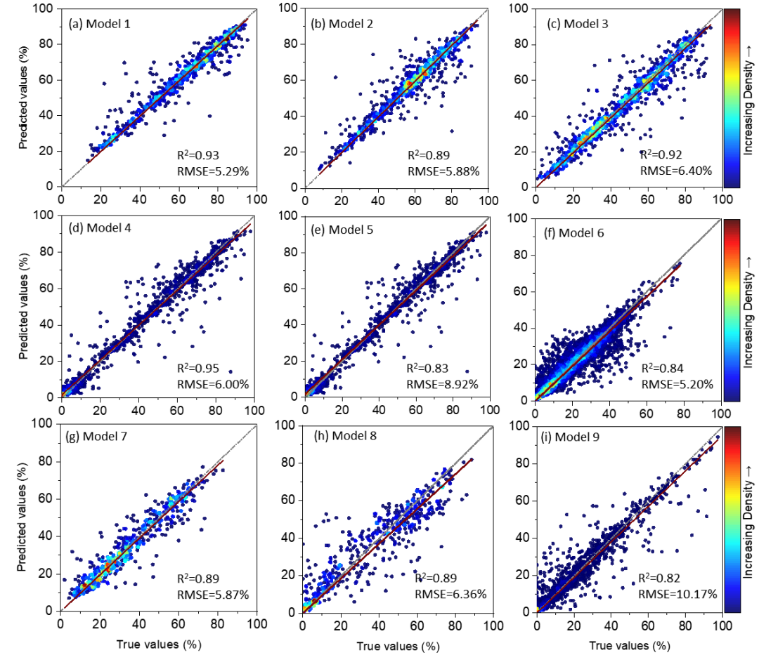
Figure 3 Model performances across different geographical regions and income groups. The true values represent the slum indicator calculated from DHS data using our slum framework, while the predicted values are produced by our machine learning-based models. For each model, a linear regression line is displayed alongside a reference line with a slope of one for comparison.
