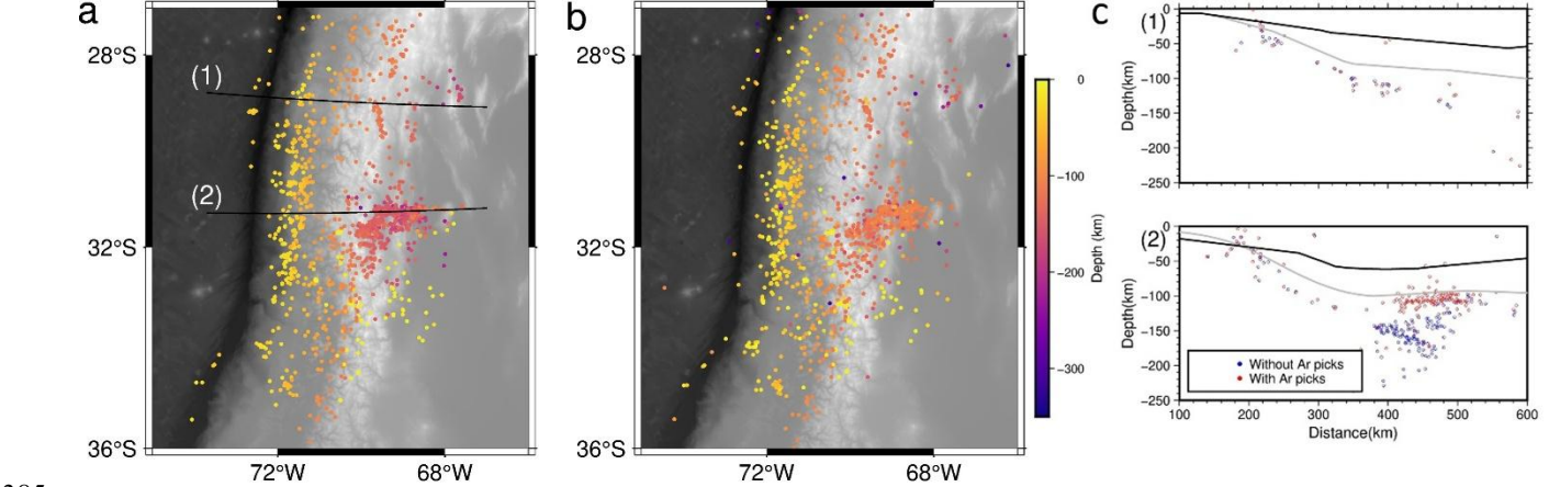
385 Figure 10: a-b) Maps showing only earthquakes for which we retrieved and added INPRES picks from the ISC Bulletin a) Hypocenters with our picks only. b) Hypocenters after including INPRES picks. Black lines indicate cross-sections 1-2. 1-2) Cross-sections comparing hypocenters when including (red) and not including (blue) INPRES picks. Each cross-section contains a 30 km swath of seismicity, i.e. events 15 km to the north and south of each cross-section. Black lines indicate the continental Moho (Tassara and Echaurren et al., 2012) and gray lines the slab (Hayes et al., 2018). 390
