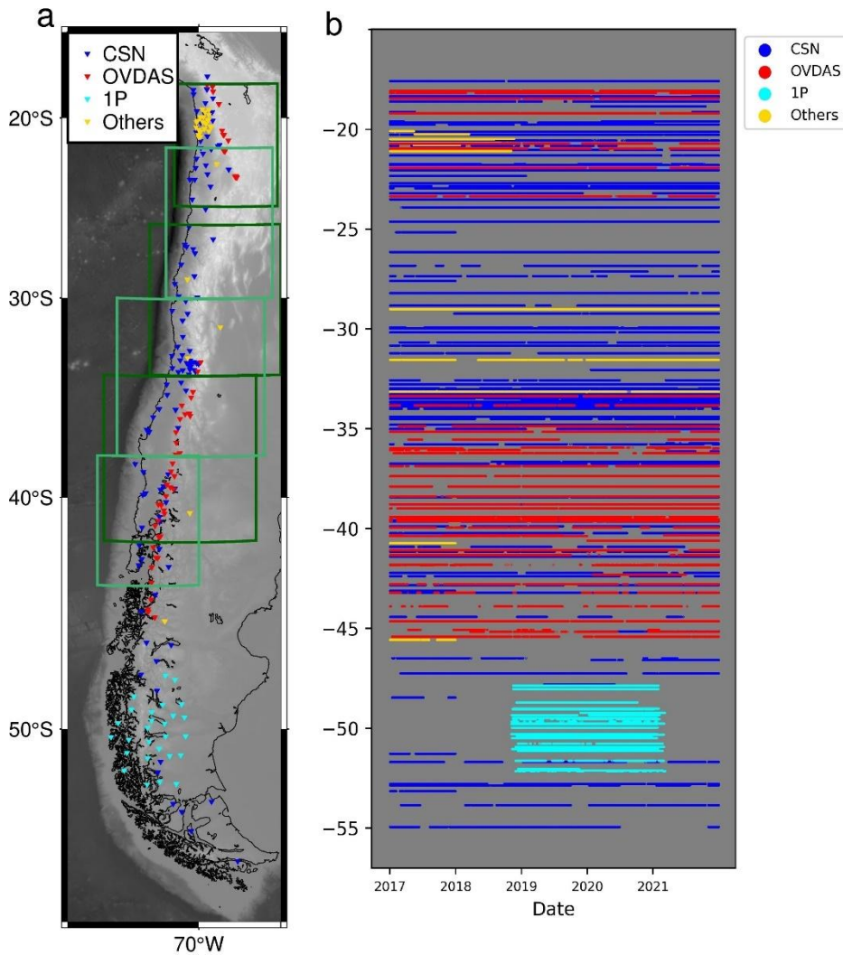
Figure 1: a) Station distribution map and b) General overview of station availability over time. The x axis shows date, between 2017-01-01 and 2021-12-31, and the Y axis shows stations sorted by latitude and color-coded with blue for all networks used by the CSN to build their catalogue (C, Universidad de Chile, 1991; C1, Universidad de Chile, 2012; CX, GFZ, 2006; IU, USGS, 1988 and G, IPGP and EOST, 1982), red for the OVDAS network (VC, Sernageomin, 2012), cyan for 1P (Wiens & Magnani, 2018) and yellow for all others. Dark and light green rectangles on a) indicate segments of the main catalogue. Thin black lines represent political boundaries. Figures S1-S20 in the supplementary material provide a more complete overview of station availability in time.
