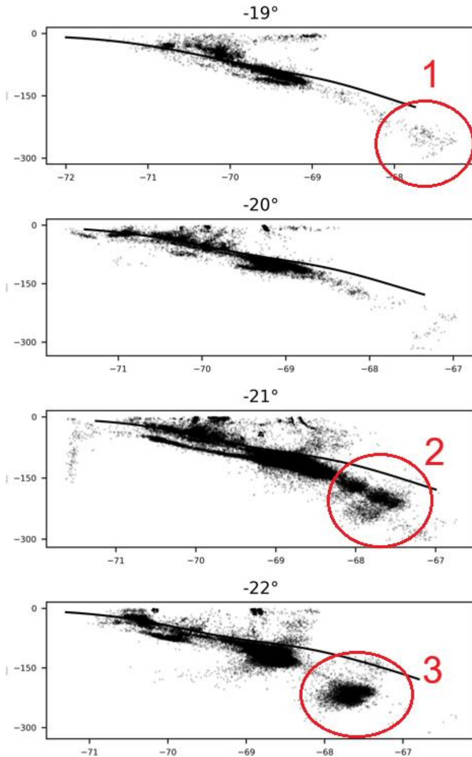
Figure: Latitudinal profiles at 19\text{--}22^\circ S. Circle 1 highlights the mentioned cluster, while circles 2 and 3 highlight clusters at the same depth but further south, which do appear in previous catalogues.
