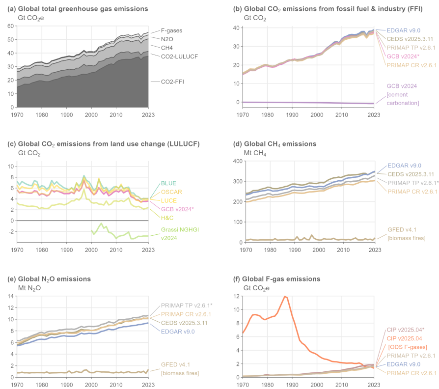
316 317 Figure 2 Annual global anthropogenic GHG emissions by source, 1970–2023. Refer to Sect. 2.1 and Table S1 for a list of 318 datasets. Datasets with an asterisk (*) indicate the sources used to compile global total greenhouse gas emissions following 319 the WGIII assessment in (a). CO 2 -equivalent emissions in (a) and (f) are calculated using GWP100 from the AR6 WGI 320 Chap. 7 (Forster et al., 2021). F-gas emissions in (a) comprise only UNFCCC F-gas emissions (see Sect. 2.1 for a list of 321 species). F-gas emissions in (f) refer to UNFCCC F-gases, except for “CIP v2024.04 [ODS F-gases]”. Some of the major 322 depicted differences between datasets (e.g. between GCB v2024 and Grassi NGHGI v2024 in panel c) are due to varying 323 system boundaries, rather than underlying uncertainties in activity levels or emissions factors.
