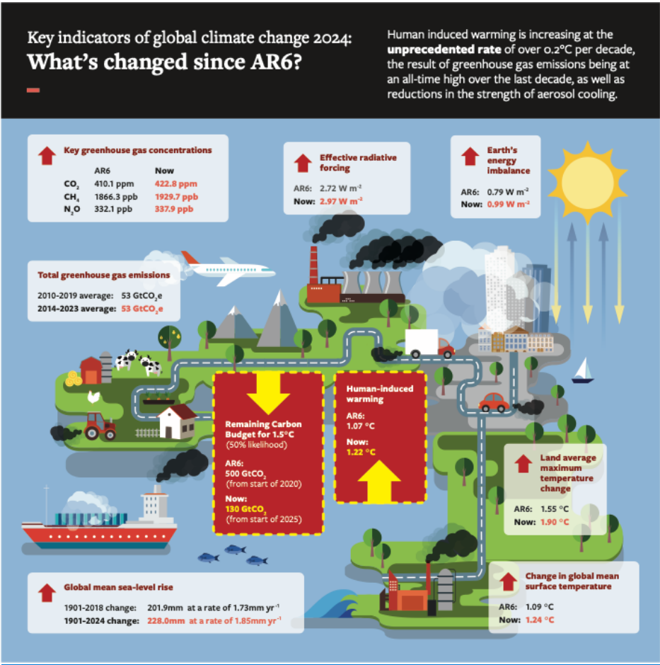
211 Figure 15. Infographic for the best estimate of headline indicators assessed in this paper.
