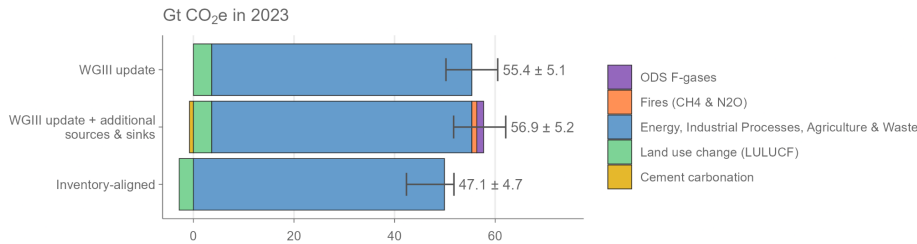
332 Figure 3 Annual global anthropogenic greenhouse gas emissions by assessment convention in 2023. Refer to Table 1 for a 333 list of underlying datasets. Differences between conventions are primarily due to differences in system boundaries (Lamb 334 et al., 2025). Uncertainties are ±8 % for CO 2 -FFI, ±70 % for CO 2 -LULUCF, ±30 % for CH 4 and F-gases, and ±60 % for 335 N 2 O, corresponding to a 90 % confidence interval. 336
