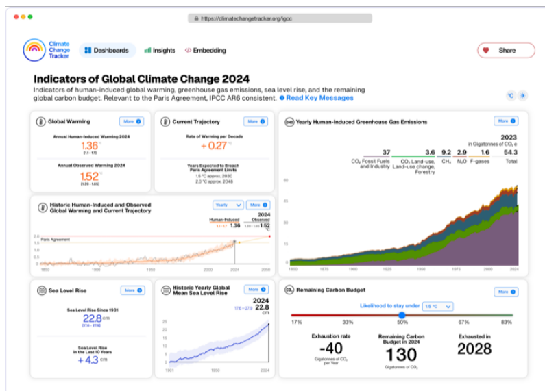
Figure 14 Screenshot of the IGCC dashboard, ( https://climatechangetracker.org/ , Climate Change Tracker, 2025).
