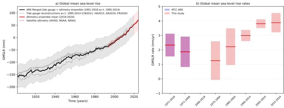
Figure 13 (a) Global mean sea-level rise time series 1901-2024 (mm). The GMSLR ensemble from AR6 in black, w.r.t. the period 1995-2014; the updated satellite altimetry ensemble in red, w.r.t. the AR6 ensemble in 2018. Individual time series are shown in dashed lines. (b) GMSLR rates (mm yr -1 ) for different periods. Uncertainties in a) show the likely range and in b) the very likely range, computed relative to 1901, including estimates of both structural uncertainty and parametric uncertainty (Palmer et al., 2021).
