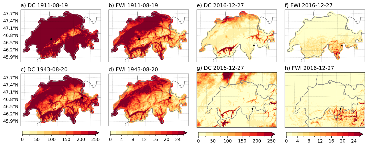
Figure 11. Drought code (DC) and fire weather index (FWI) for the three forest fires in the reconstruction . a and b) Forest fire in Simmenfluh, 1911, c and d) forest fire in August 1943 on the Calanda mountain slopes, e and f) forest fire in Misox in winter 2016 , 2016 . g and h) same show the forest fire in Misox , but for based on the COSMO-1 model . The approximate locations of the fires are shown as black asterisks in each panel.
