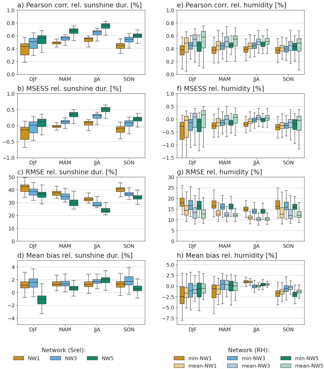
Figure 8. Cross-validation results for relative sunshine duration and relative humidity across the different networks and seasons. a) Pearson correlation coefficients, b) MSESS, c) normalized RMSE, and d) mean bias of seasonal relative sunshine duration for five the three different networks. de ) Pearson correlation coefficients , ef ) MSESS, fg ) RMSE, and fg-h ) mean bias for daily minimum and daily mean humidity considering the three networks. Relative sunshine duration is evaluated in the reference period from 1971 to 2020, and relative humidity is evaluated from 2016 to 2020.
