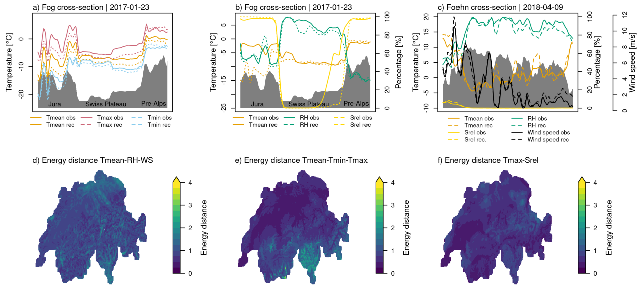
Figure 9. Consistency of the different variables based on cross-section of a-b) a fog day in the Swiss Plateau on the 2017-01-23 and c) a foehn day in Meiringen on the 2018-04-09. The dashed lines show the reconstruction, while the solid lines show the reference data set (i.e. observations). The maps of energy distance are shown for d) daily mean temperature, relative humidity and wind speed, e) maximum, minimum, and daily mean temperature, and f) maximum temperature and sunshine duration.
