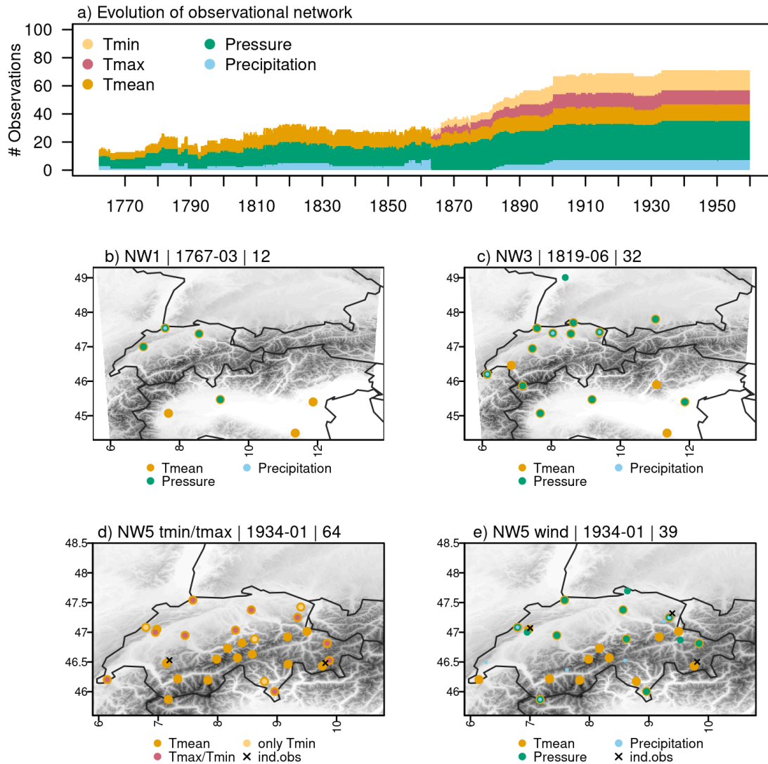
Figure 1. a) Evolution of available observations over time between 1763 and 1960 . b) Network Locations of stations in the network NW 1 in 1767 , c) locations of stations in network NW 3 in 1819 , d) locations of stations used for the reconstruction of maximum and minimum temperature for the period since 1864 in 1934 , e) Network locations of stations used for the reconstruction of wind fields for the periods since 1864 . The networks prior to 1864 in 1934, NW 1 and NW 3 are identical to the data networks used in Imfeld et al. (2023) (see Fig. 1 therein) . The date in the headings indicates the year for which the network is representative, while the number corresponds to the available observations for that time step . A black star-cross indicates that measurements from this station have been used for an independent evaluation (tmin/tmax and wind speed). Note that panel a) shows considerably fewer observations than in Imfeld et al. (2023), because evaluations showed that using fewer precipitation observations led to better results.
