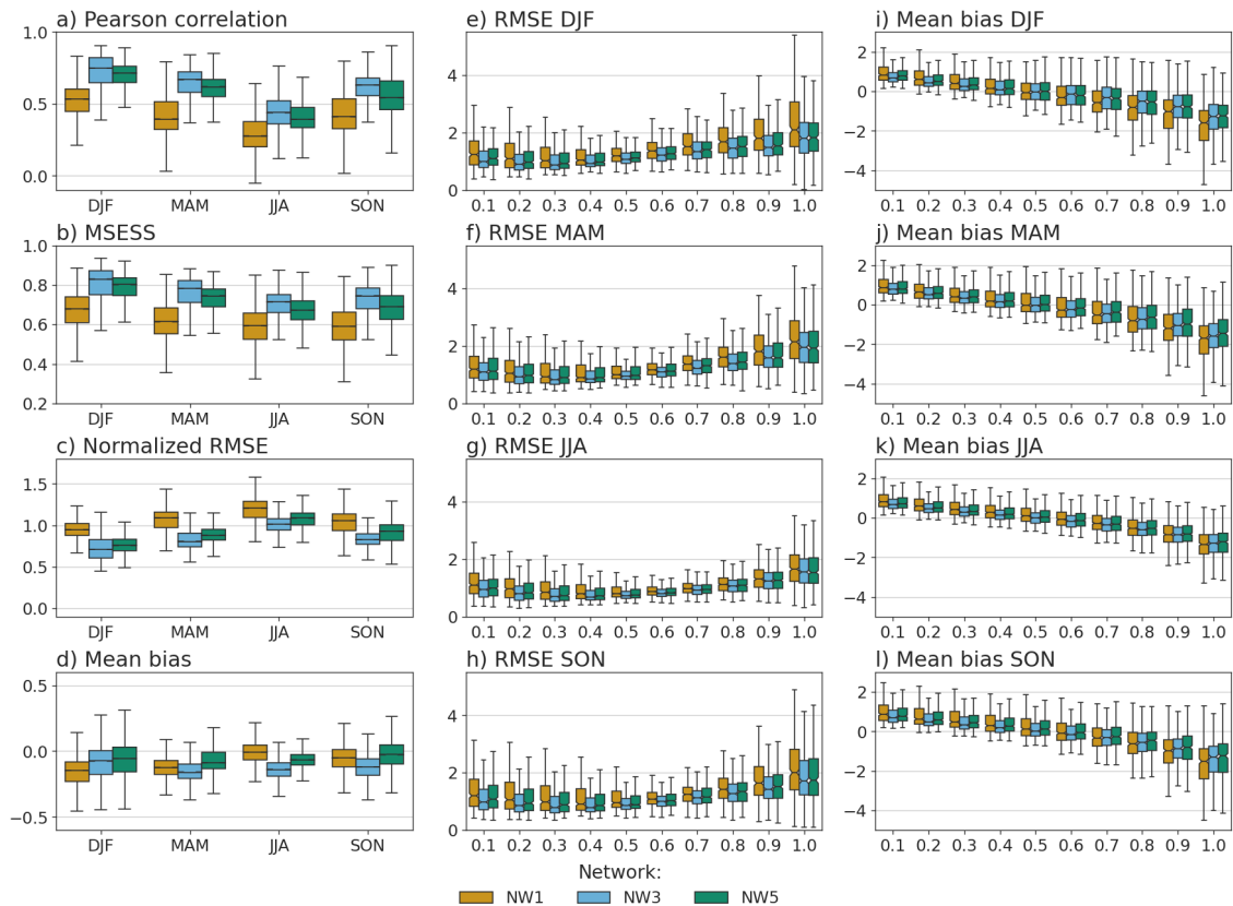
Figure 3. Cross-validation results of wind speed for different the three networks (NW1, NW3, and NW5) and for the four seasons . a) Pearson correlation coefficient, b) MESS, c) normalized RMSE, and d) mean bias of seasonal wind speed for five-three different networks . The second and third columns show cross-validation results calculated by deciles of the observed value for the four seasons and three networks : e-h) RMSE of percentiles wind speed for DJF, MAM, JJA, and SON for three networks, and i-l) mean bias of percentiles of wind speed. The cross-validation results are shown for DJF, MAM, JJA successive decile bins, and SON with the x-axis indicating the upper bound of each bin. Percentiles The deciles are calculated based on the reference data set separately for each grid cell.
