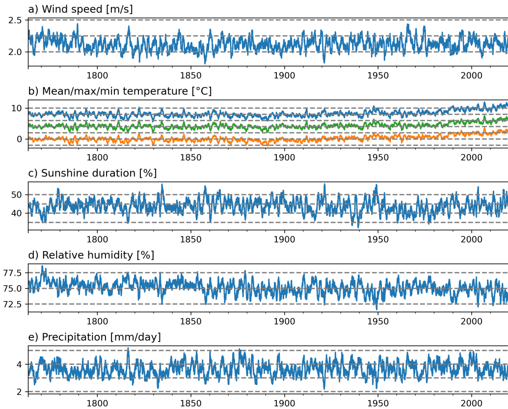
Figure 10. Long-term evolution of the reconstructed variables. a) daily Daily wind speed [m/s], b) daily mean, maximum, and minimum temperature [ ^{\circ} C], c) daily relative sunshine duration [%], d) mean daily relative humidity [%], and e) daily precipitation sums [mm/day] for comparison. The time series shows the area mean across the entire Switzerland, smoothed with a 1-year running mean.
