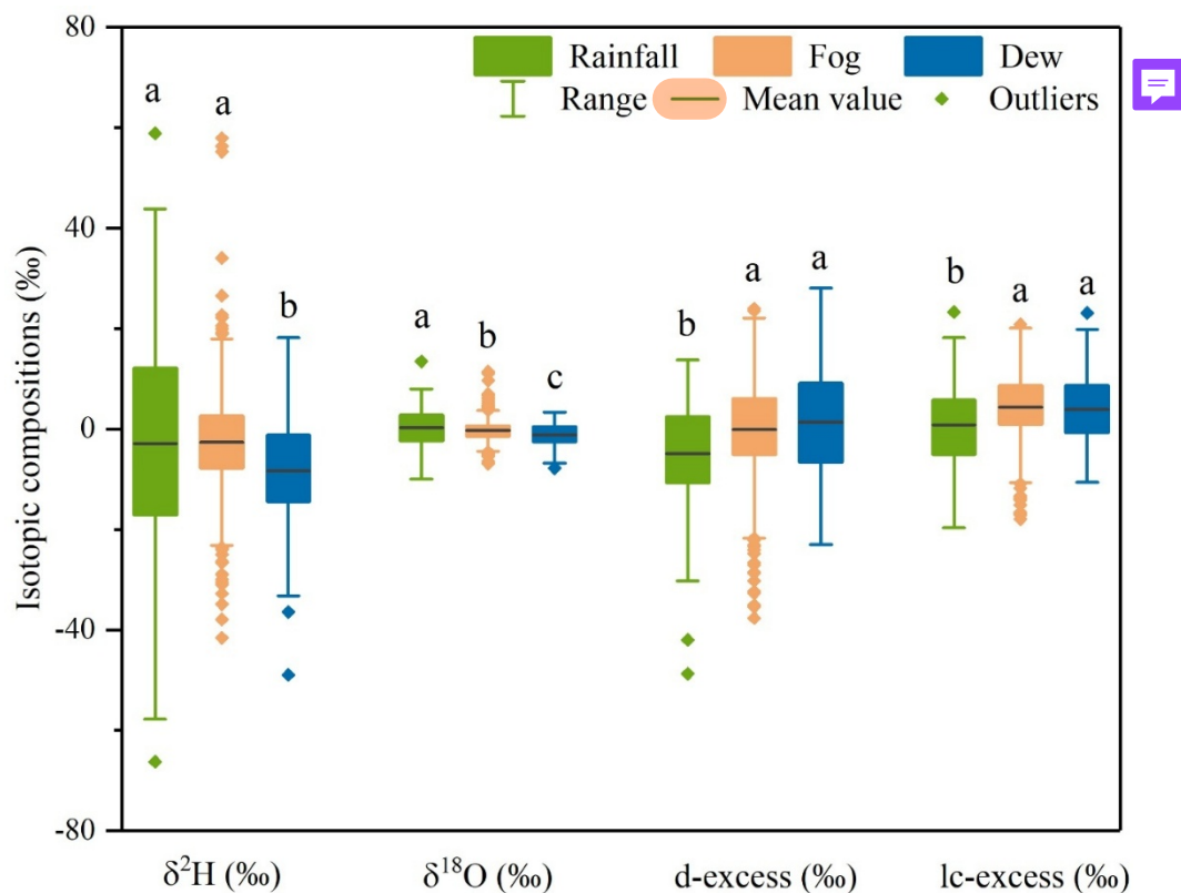
Figure 9: Comparison of stable isotope compositions ( \delta^2\text{H} , \delta^{18}\text{O} , d-excess, and lc-excess) of rainfall, fog, and dew water samples during 2014 and 2023 at the Gobabeb–Namib Research Institute.
