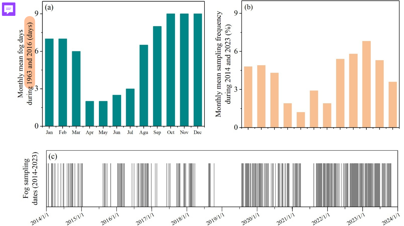
160 Figure 2: Monthly mean foggy days during 1963 and 2016 and the actual coverage and consistency of our isotope dataset at the Gobabeb–Namib Research Institute throughout the study period (2014–2023). a. Monthly mean number of foggy days from 1963 to 2016. b. Monthly sampling frequency of fog water during the study period from 2014 to 2023. c. Fog sampling dates during the study period from 2014 to 2023. The monthly mean fog days between 1963 and 2016 were derived from Spirig et al. (2019).
