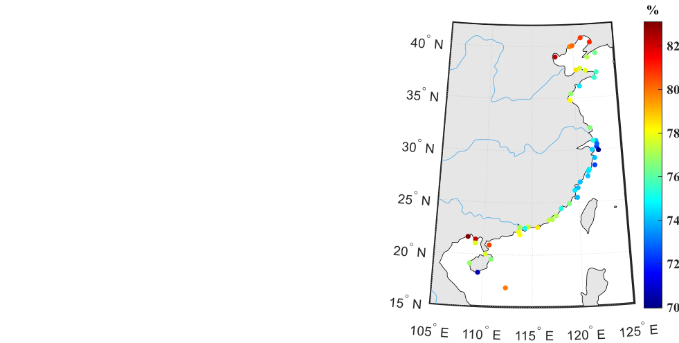
315 Figure 14: Correlation coefficients between GNSS PWV and SST.
