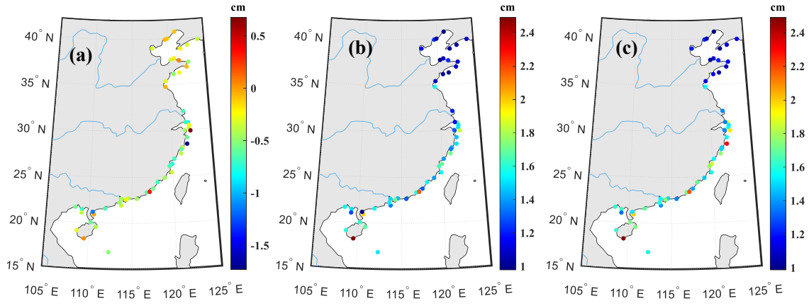
Figure 4: Comparison between GNSS ZTDs and ERA5 ZTDs: mean bias (a), STD (b), and RMS (c).
