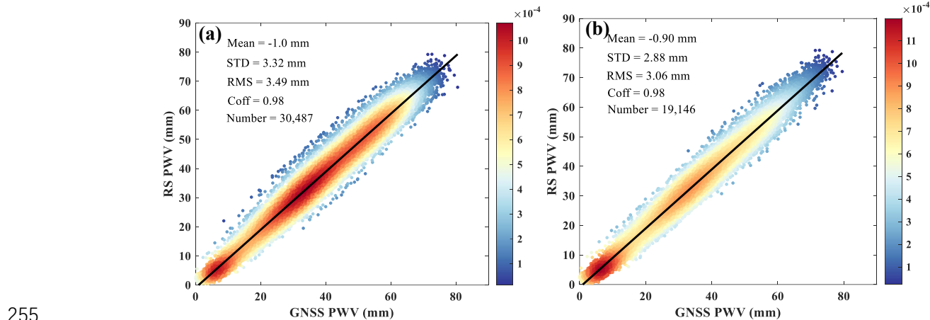
Figure 9: Comparison between GNSS PWV and RS PWV using 10 levels (a) and 11 levels (b).
