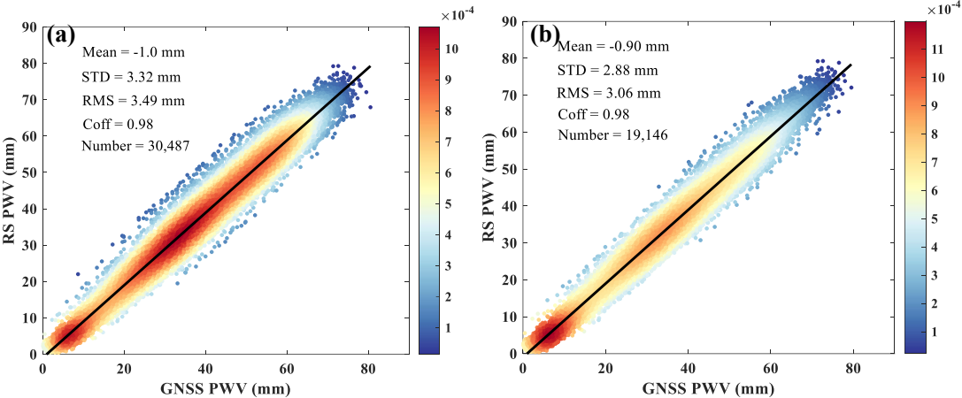
Figure 9: Comparison between GNSS PWV and RS PWV using 10 levels (a) and 11 levels (b).
