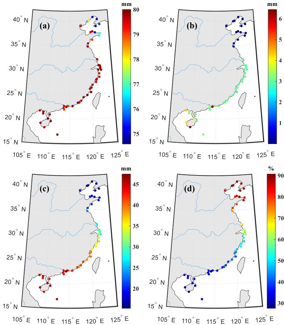
Figure 11: Maxima (a), minima (b), mean values (c), and coefficients of variations (d) of hourly PWV products of China coastal GNSS stations.
