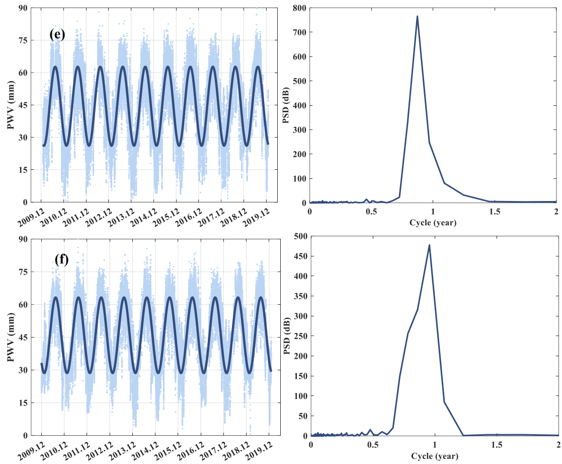
300 Figure 12: PWV time series and corresponding spectrum analysis in BLHT(a), BTGU (b), DLSI (c), DSPU (d), NHZH (e), and NWZU (f).
