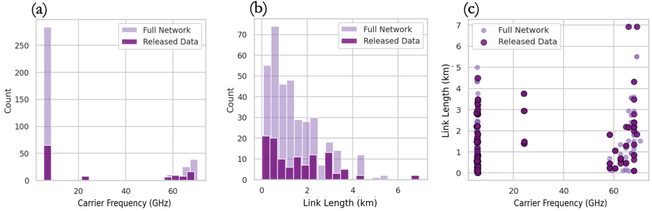
Figure 5. Feature distributions of OpenMesh dataset: sublink lengths range in kilometers (km) and carrier frequencies (GHz). (a) Carrier-frequency histogram; (b) sublink-length histogram; (c) sublink length versus carrier frequency scatter.
