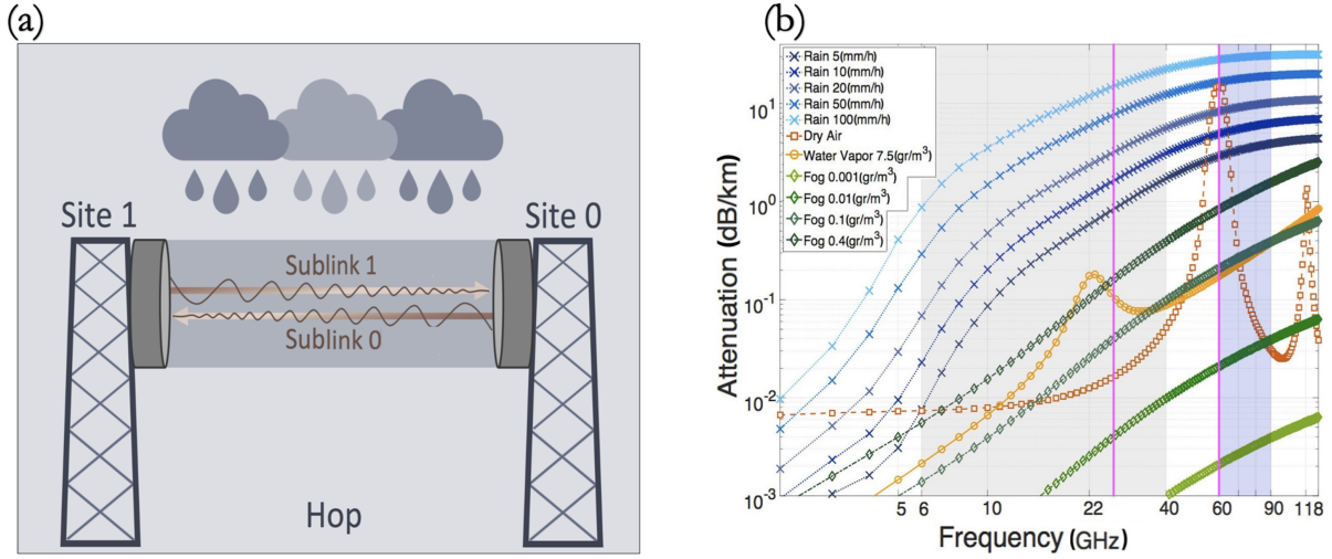
Figure 2. (a) Schematic of a point-to-point wireless communication link (Fencl et al., 2023). (b) Signal attenuation per km for various atmospheric phenomena as a function of frequency (ITU-R P.530, 2017; Ostrometzky, 2017).
