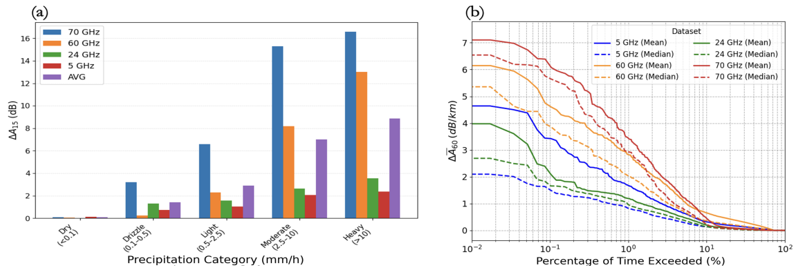
Figure 11. Attenuation patterns across frequencies over the study period. (a) Attenuation for a 1.5 km sublink per frequency band, grouped by precipitation intensity (World Meteorological Organization, 2018). (b) Exceedance probability plots. The x-axis shows the percentage of samples that exceed the y-axis value of hourly aggregated attenuation across all sublinks, grouped by carrier frequency.
