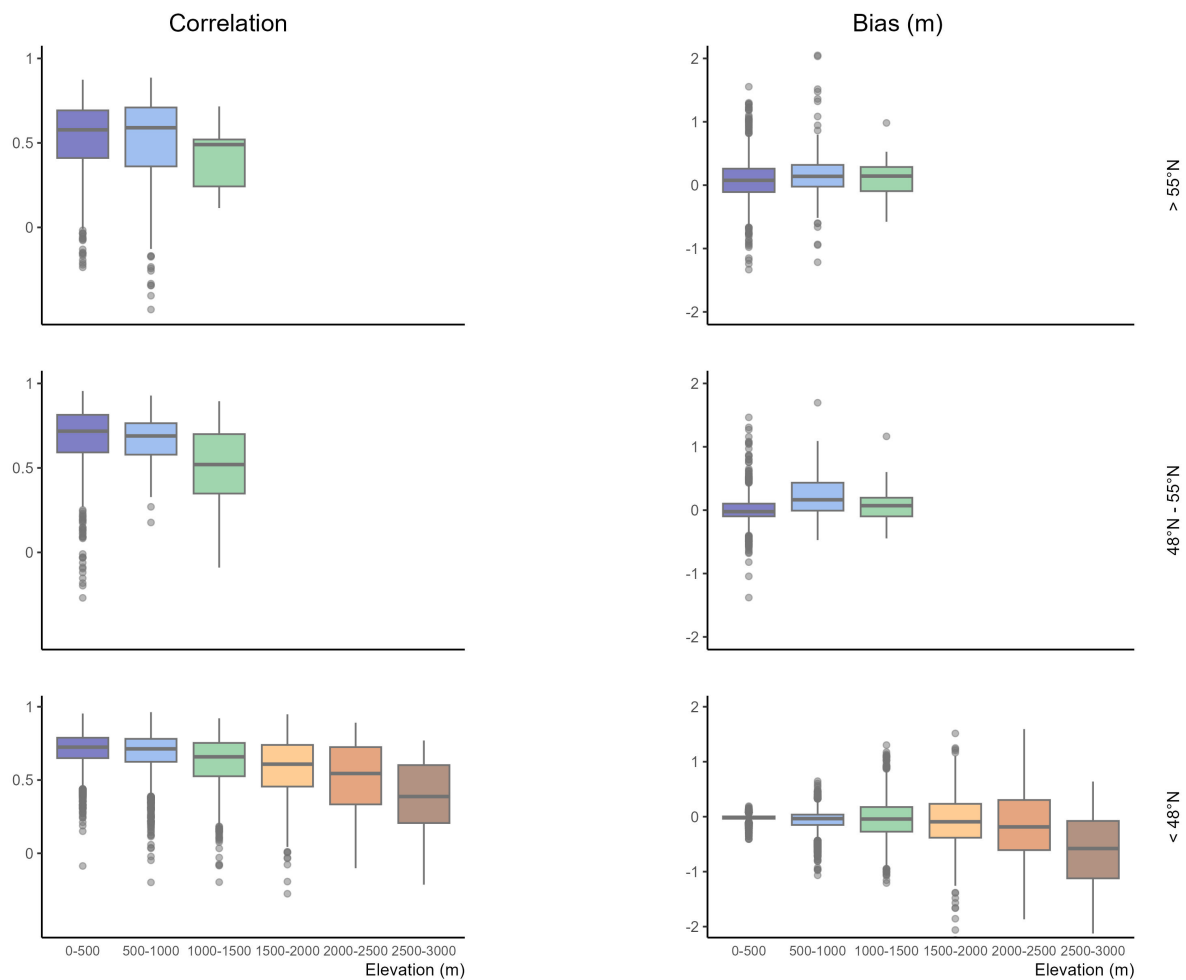
Figure 6. Correlation and bias boxplots resulting from MTMSI evaluation by 500 meter elevation bands, the three lines corresponding to different latitude ranges.
