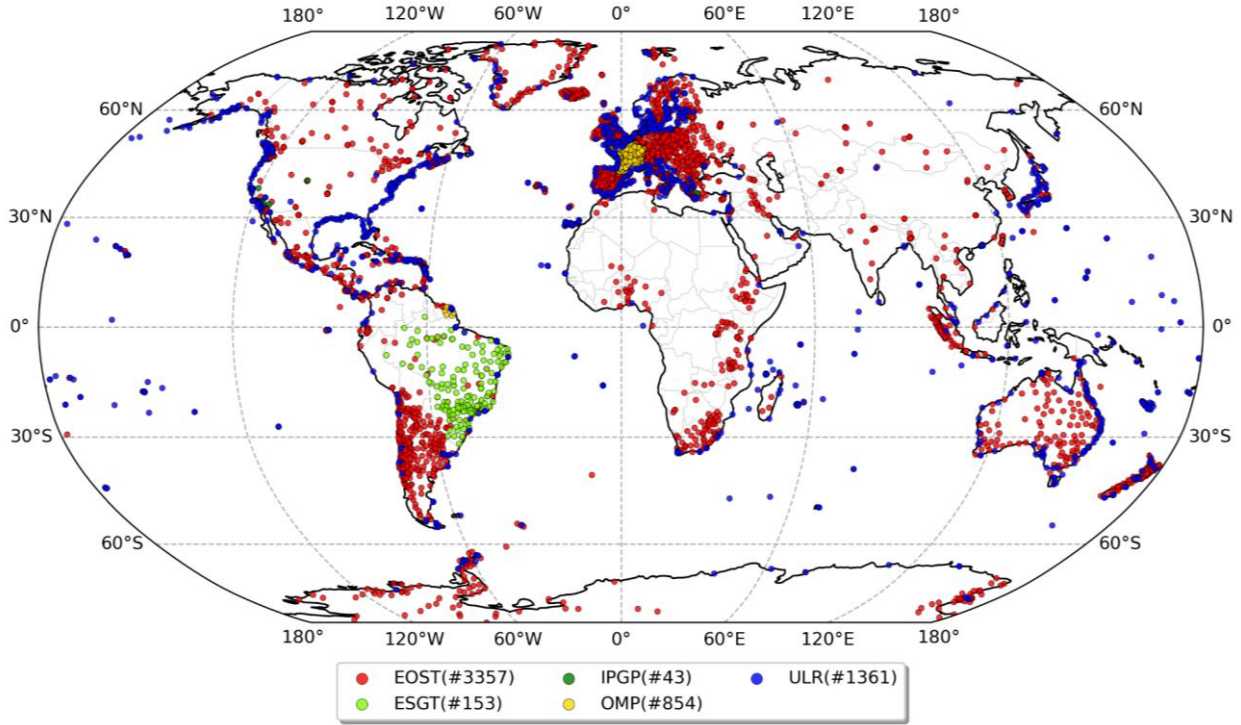
Figure 1: The SPOTGINS sub-networks processed by each member in August 2025. The number of stations included in each sub-network is also indicated.
