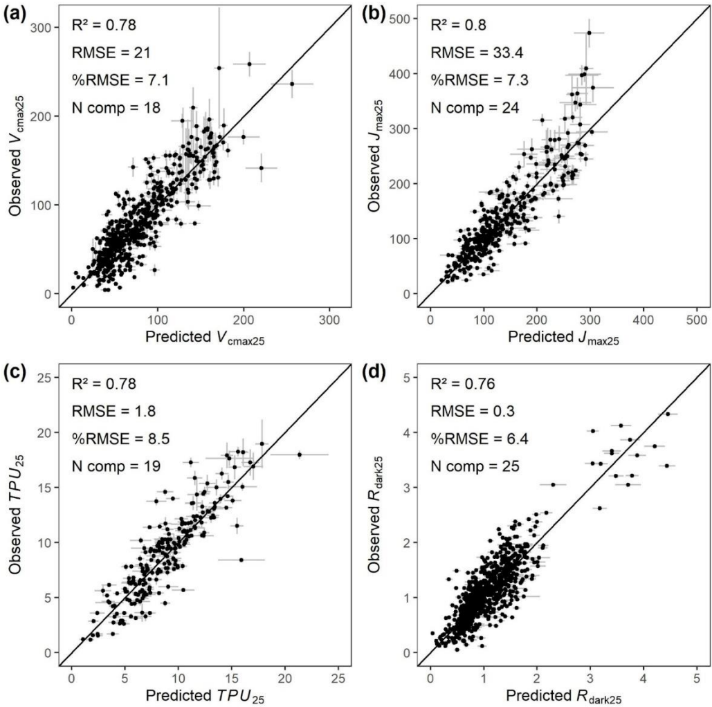
385 Figure 8: Observed photosynthetic properties obtained from gas exchange measurements vs reflectance-based partial least square regression prediction. a) Maximum carboxylation rate of Rubisco ( V_{cmax25} ). b) Maximum potential rate of electron transport ( J_{max25} ).
