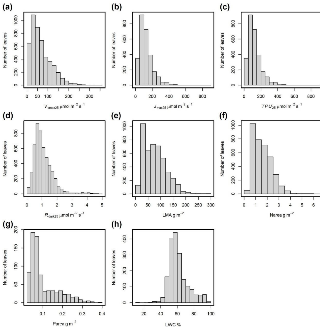
360 Figure 6: Frequency distributions of observations for the main leaf traits. a) Maximum carboxylation rate at 25 °C ( V_{cmax25} ). b) Maximum potential electron transport rate at 25 °C ( J_{max25} ). c) Triose phosphate utilization rate at 25 °C ( TPU_{25} ). d) Dark-adapted leaf respiration rate at 25 °C ( R_{dark25} ). e) Leaf dry mass per unit area of fresh leaf (LMA). f) Nitrogen content per surface area (Narea). g) Phosphorus content per surface area (Parea). h) Leaf water content (LWC).
