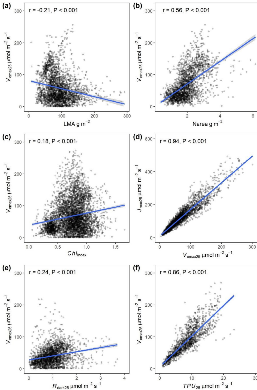
370 Figure 7: Scatter plot between the photosynthetic capacity ( V_{cmax25} ) and other leaf traits included in the GSTI database. a) Leaf mass per surface area (LMA). b) Nitrogen content on an area basis (Narea). c) Chlorophyll index derived from the reflectance data using Gitelson et al. (2003) index. d) Maximum potential electron transport rate at 25°C ( J_{max25} ). e) Dark-adapted leaf respiration rate at 25 °C ( R_{dark25} ). f) Triose phosphate utilization rate at 25 °C ( TPU_{25} ). The blue lines are linear regression fits.
