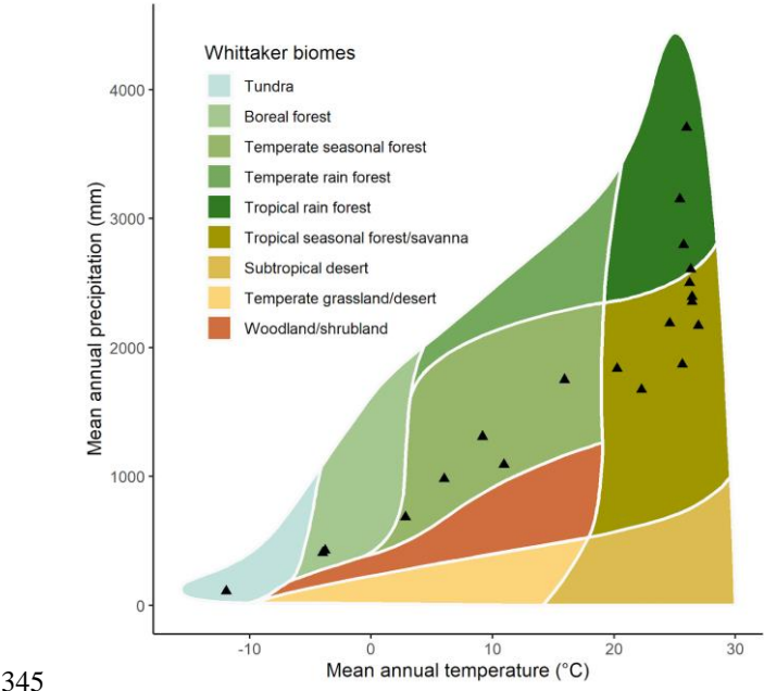
345 Figure 4: Mean annual rainfall and mean annual temperature for the 20 natural sites included in the GSTI database plotted within the climatic boundaries of Whittaker's biomes.
