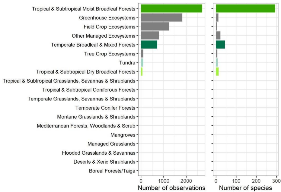
350 Figure 5 Number of observations and species per biome. The list of biomes derives from Olson et al., (2001) list of 14 terrestrial biomes that we completed with 5 managed environment classes (managed grasslands, field crop ecosystems, tree crop ecosystems, greenhouse ecosystems, and other managed ecosystems).
